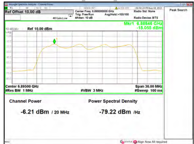
Channel Power+PSD_802.11n20_802.11n20 6895MHz
