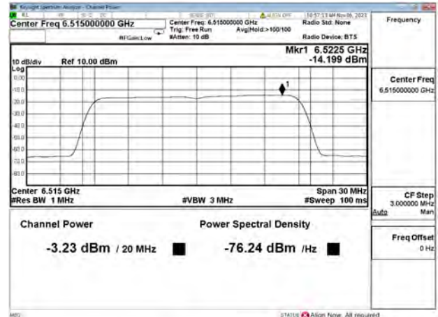
Channel Power+PSD_802.11n20_802.11n20 6515MHz
