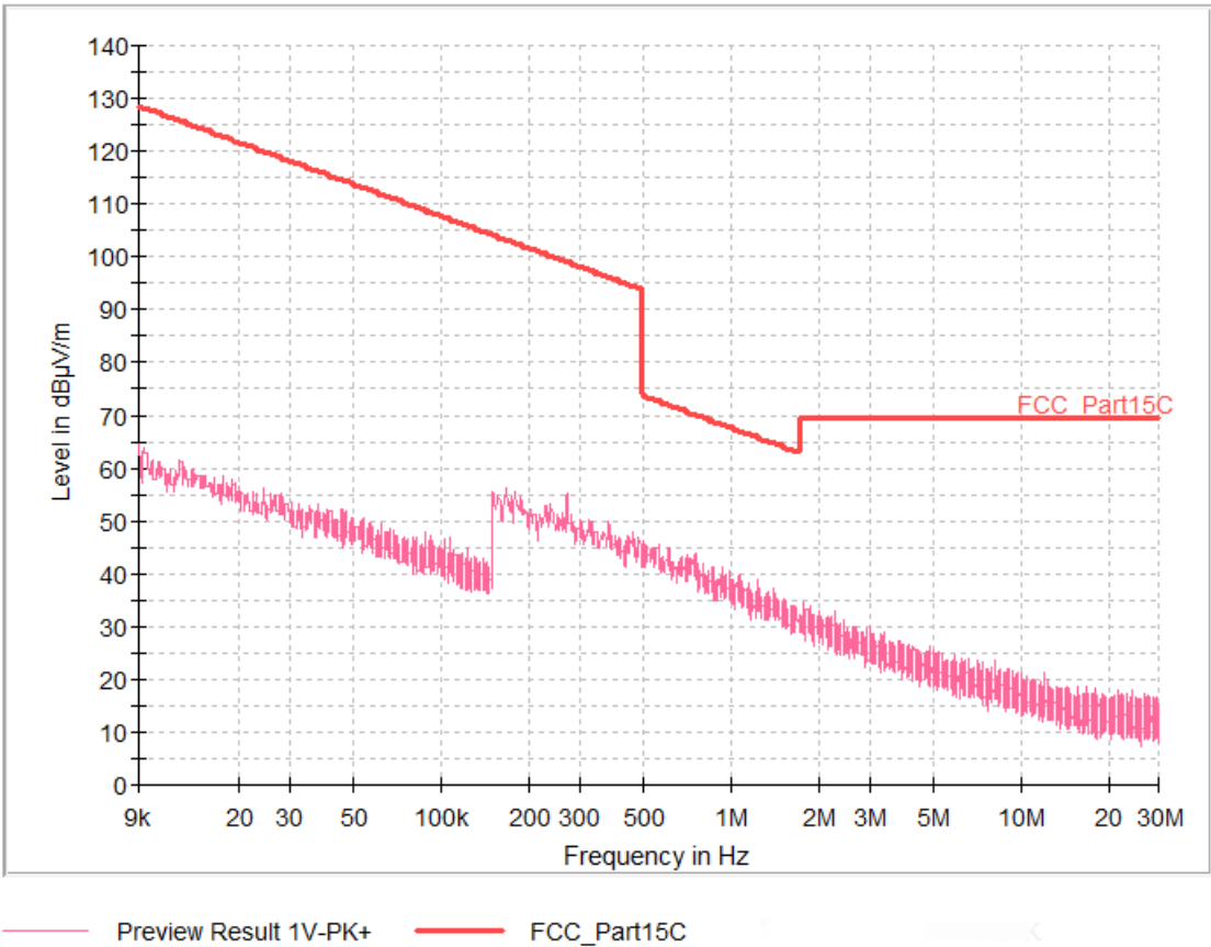
Fig. 52: Ambient level. Frequency range: 9 kHz – 30 MHz - Axis X
