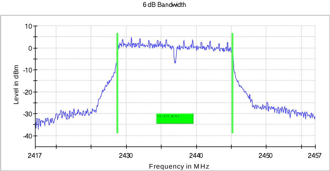
Fig. 26: Middle Channel -DTS Bandwidth
