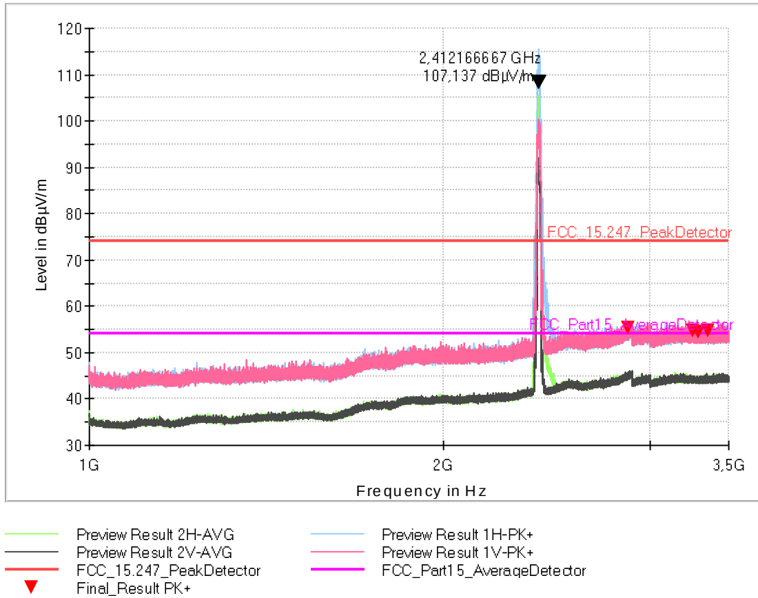
Fig. 69: Low Channel - Frequency range: 1 GHz – 3.5 GHz
