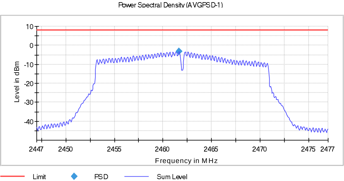
Fig. 41: High Channel - Power Spectral Density
