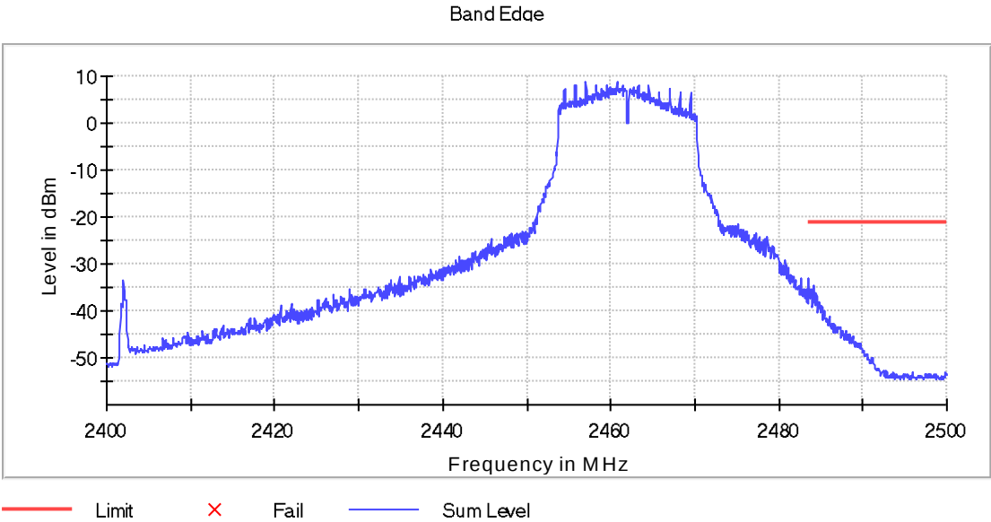
Fig. 46: High Channel - Band Edge
