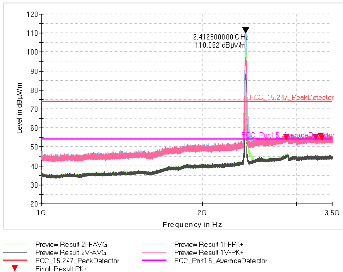
Fig. 75: Low Channel - Frequency range: 1 GHz – 3.5 GHz
