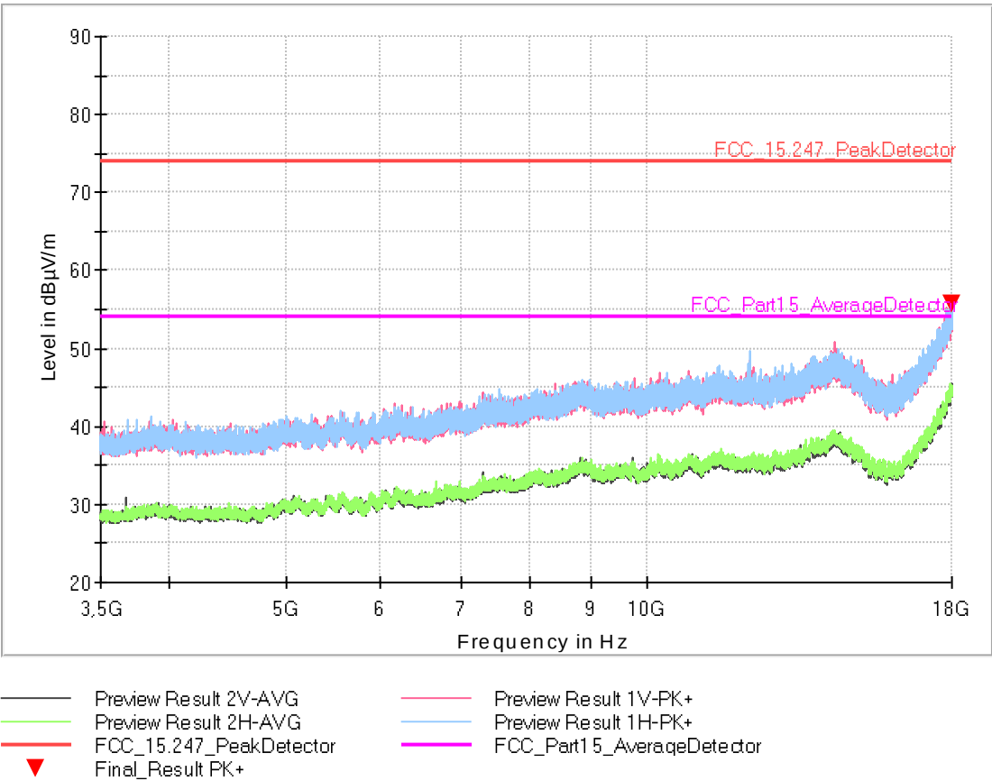
Fig. 74: High Channel - Frequency range: 3.5 GHz – 18 GHz
