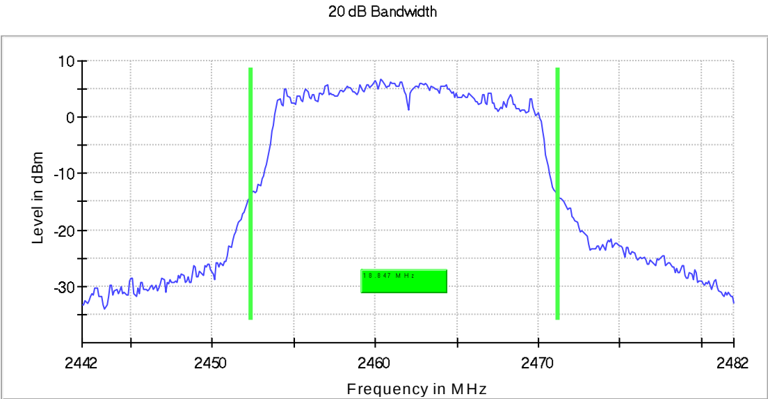
Fig. 14: High Channel - Emission Bandwidth 20dB
