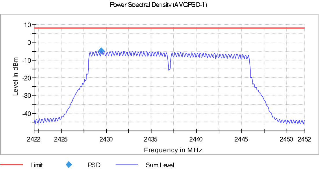
Fig. 40: Middle Channel - Power Spectral Density
