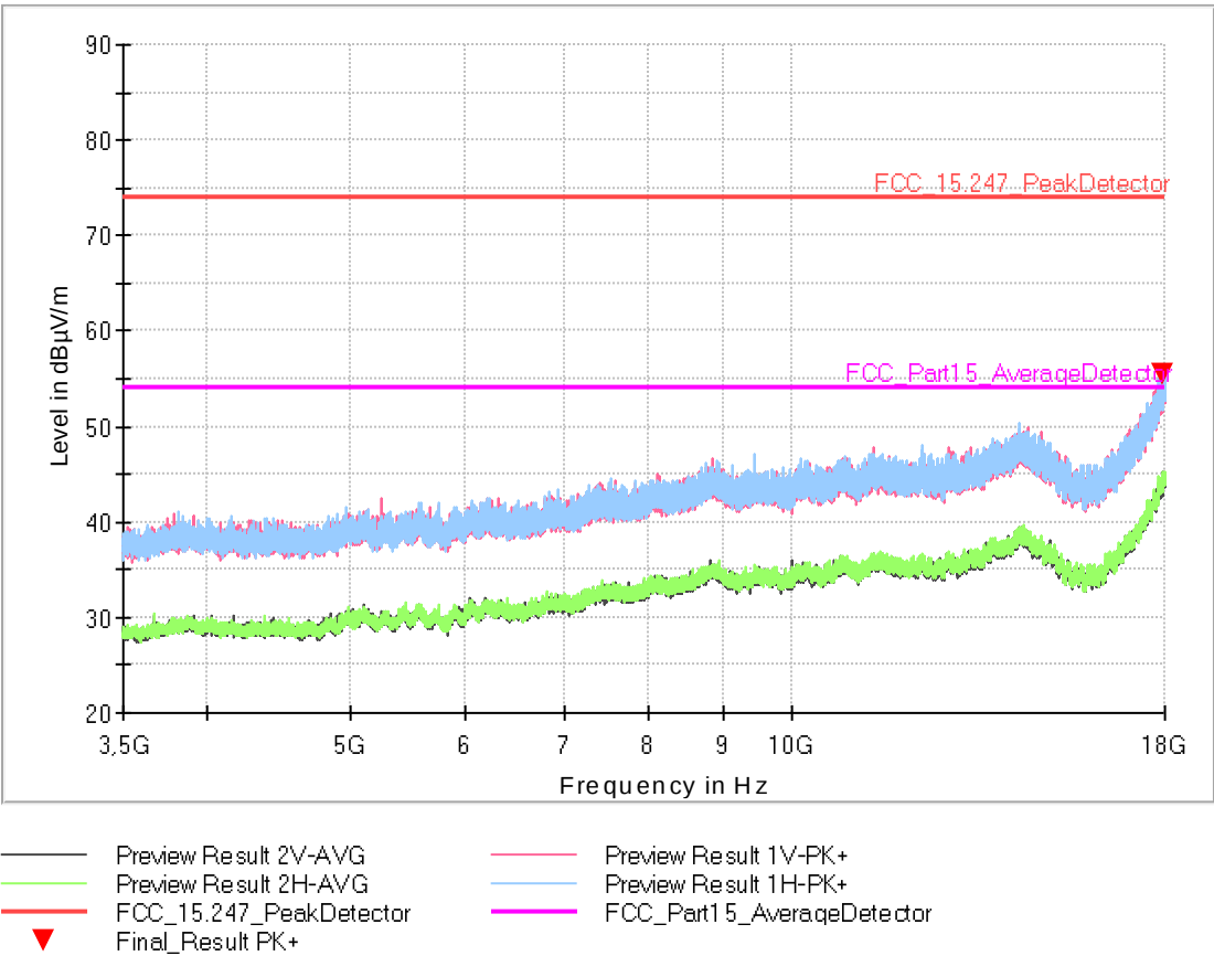
Fig. 80: High Channel - Frequency range: 3.5 GHz – 18 GHz
