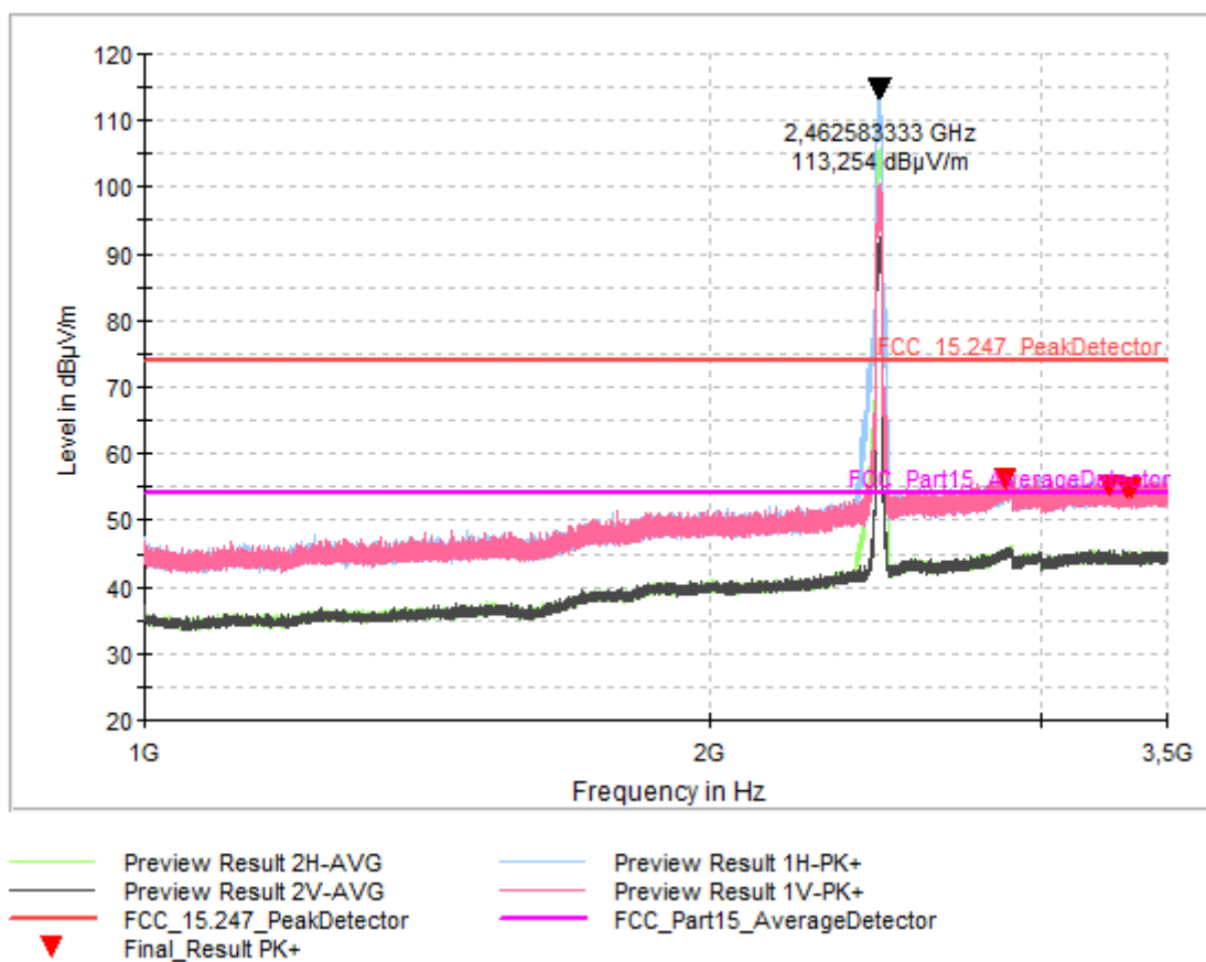
Fig. 71: High Channel - Frequency range: 1 GHz – 3.5 GHz
