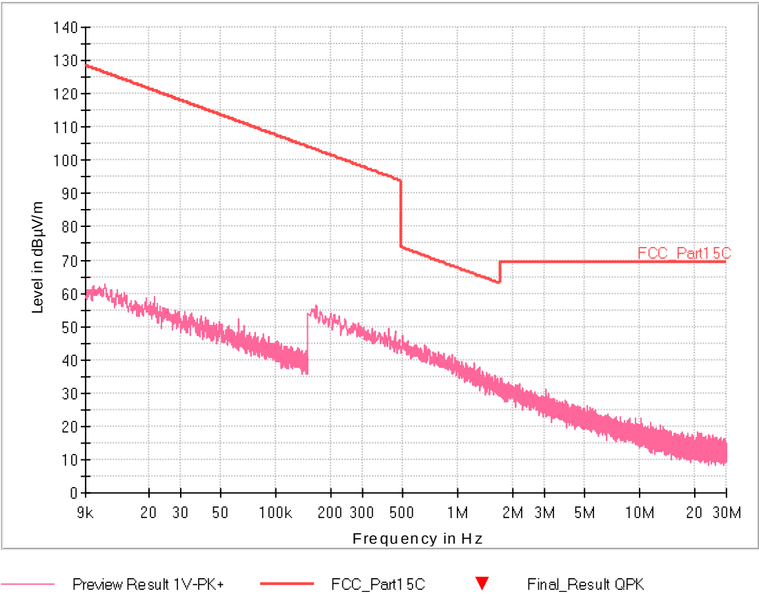
Fig. 61: All Modulation/All Channel. Frequency range: 9 kHz – 30 MHz – Axis Z
