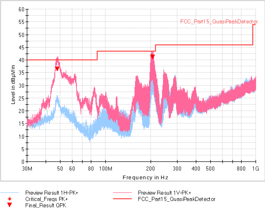
Fig. 62: All Modulation/All Channel - Frequency range: 30 MHz – 1GHz
