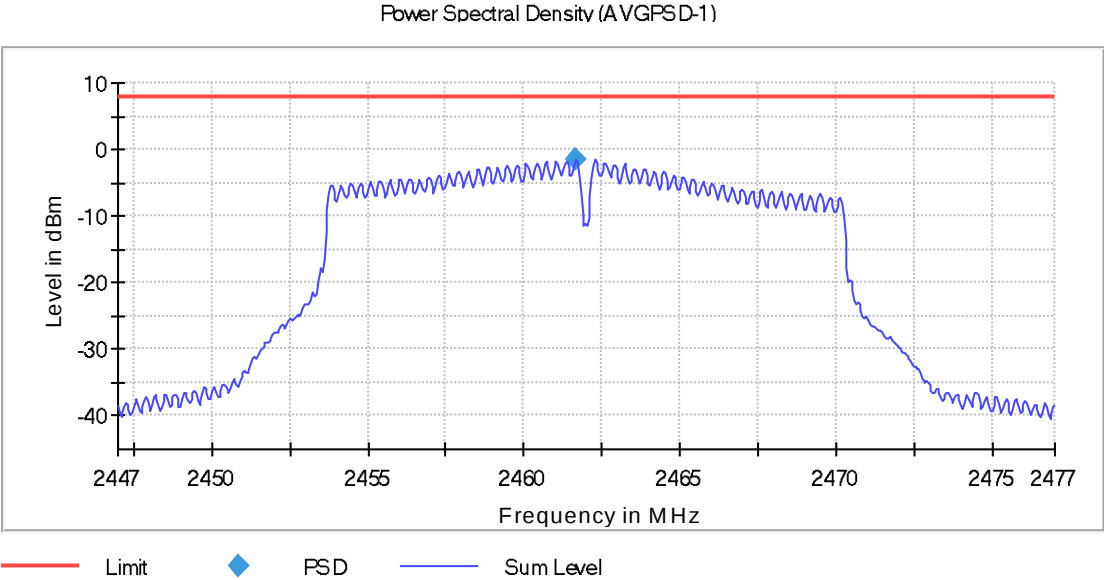
Fig. 38: High Channel - Power Spectral Density
