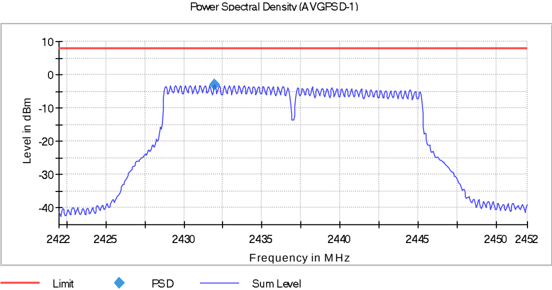
Fig. 37: Middle Channel - Power Spectral Density
