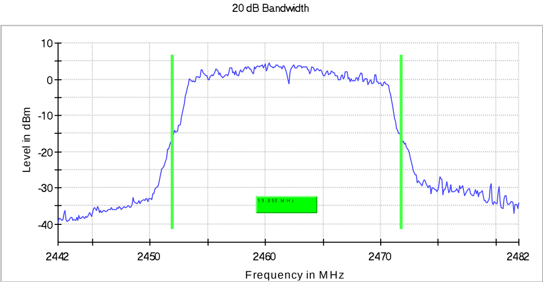
Fig. 20: High Channel - Emission Bandwidth 20dB
