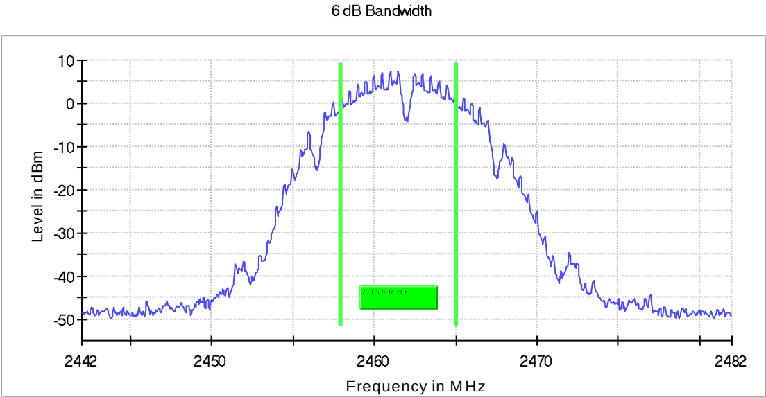
Fig. 24: High Channel - DTS Bandwidth
