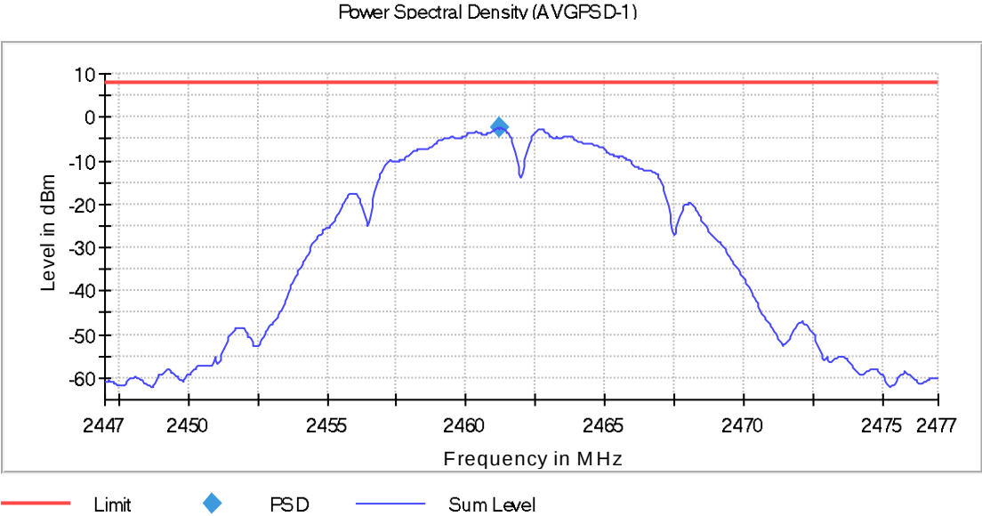
Fig. 35: High Channel - Power Spectral Density
