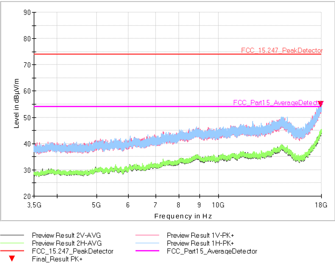
Fig. 73: Middle Channel - Frequency range: 3.5 GHz – 18 GHz
