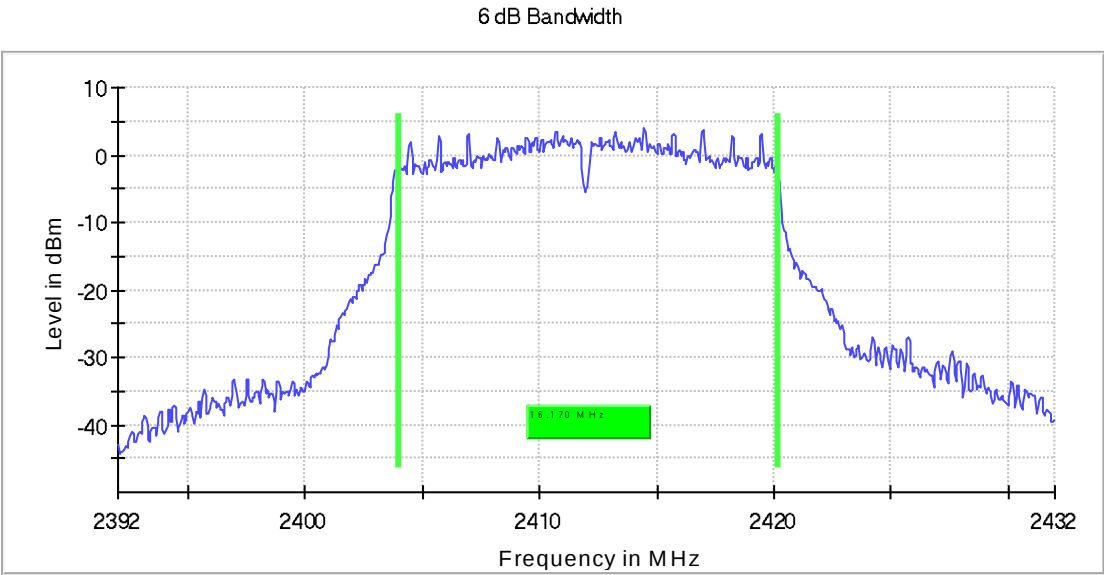
Fig. 25: Low Channel - DTS Bandwidth
