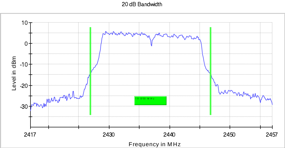
Fig. 12: Middle Channel - Emission Bandwidth 20dB
