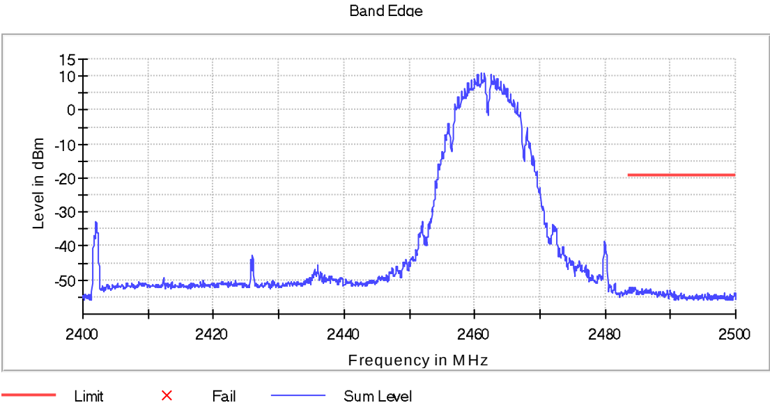
Fig. 44: High Channel - Band Edge
