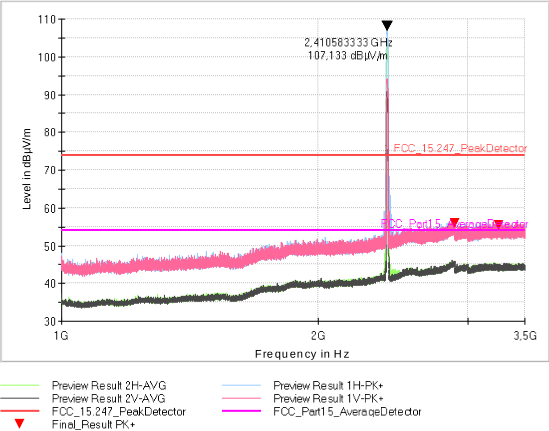
Fig. 63: Low Channel - Frequency range: 1 GHz – 3.5 GHz
