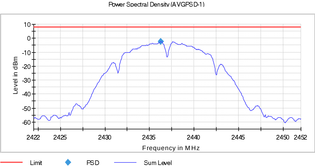
Fig. 34: Middle Channel - Power Spectral Density
