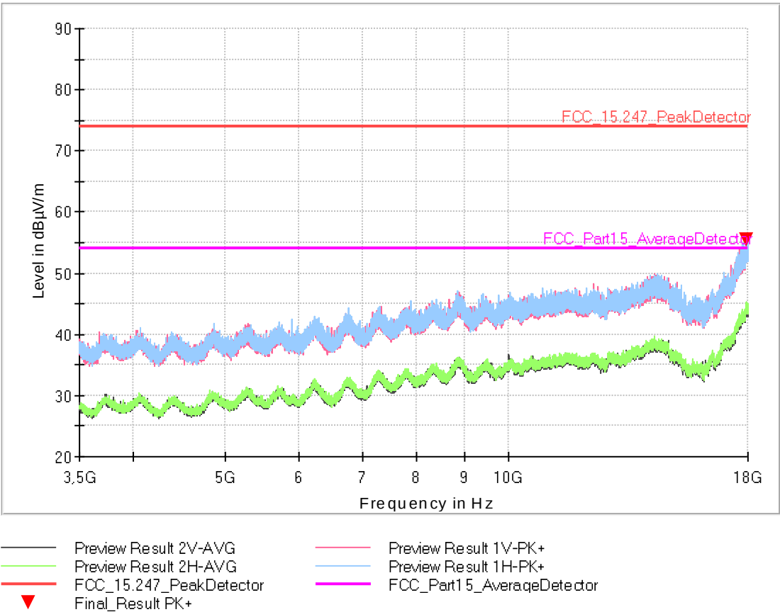
Fig. 68: High Channel - Frequency range: 3.5 GHz – 18 GHz
