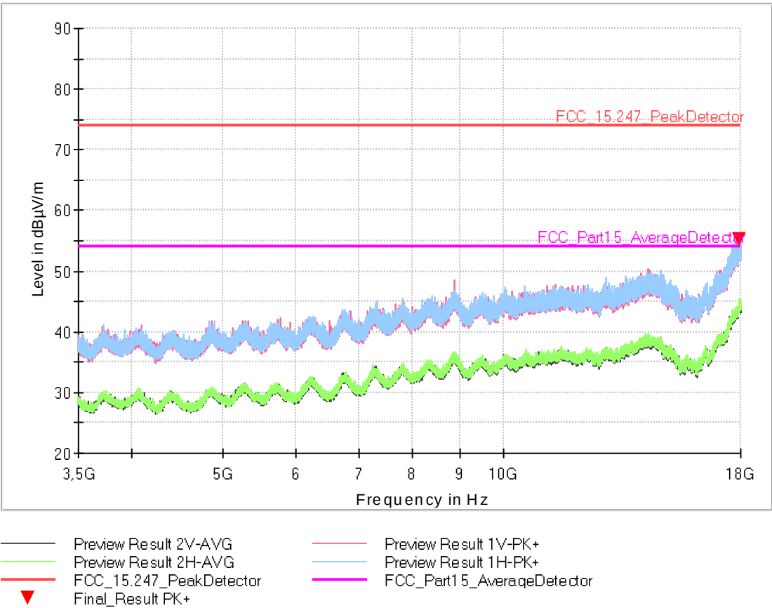
Fig. 67: Middle Channel - Frequency range: 3.5 GHz – 18 GHz
