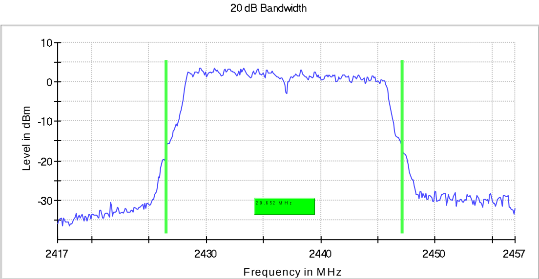
Fig. 18: Middle Channel - Emission Bandwidth 20dB
