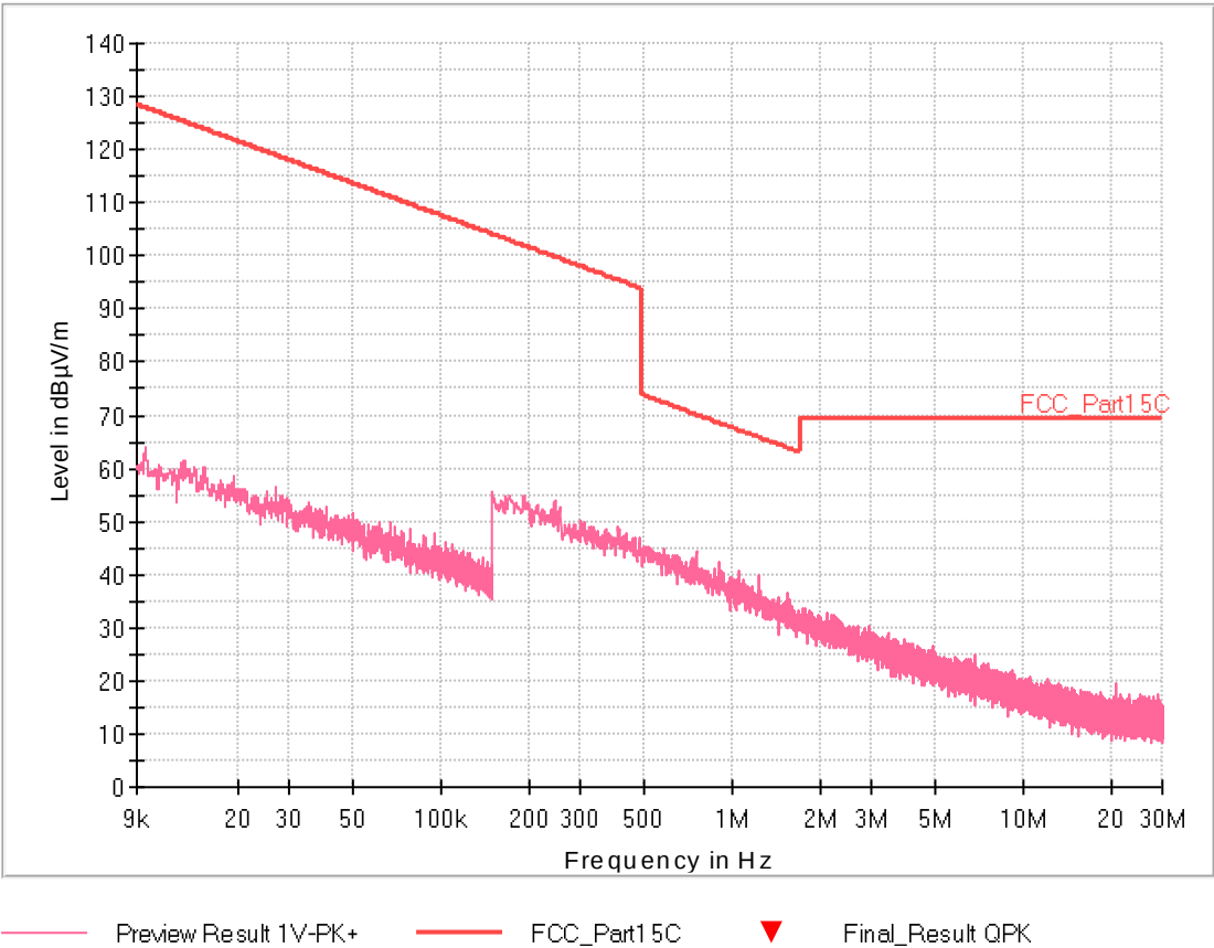
Fig. 60: All Modulation/All Channel. Frequency range: 9 kHz – 30 MHz – Axis Y
