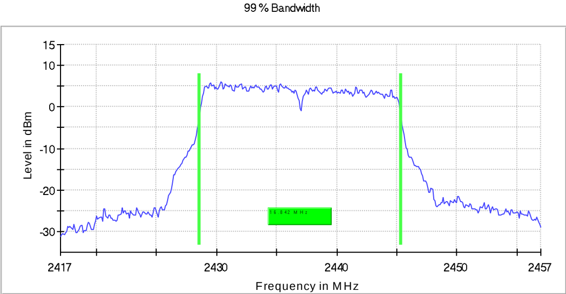
Fig. 11: Middle Channel - 99% Occupied Channel Bandwidth
