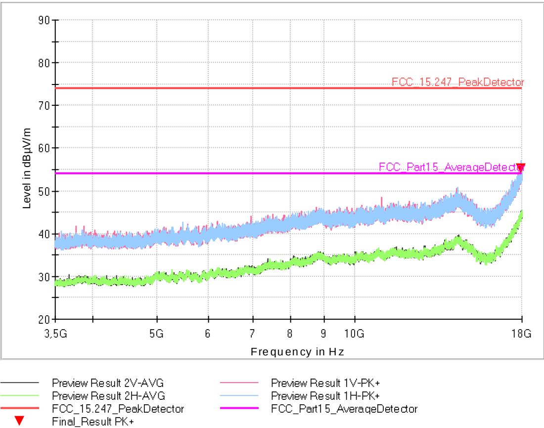
Fig. 79: Middle Channel - Frequency range: 3.5 GHz – 18 GHz
