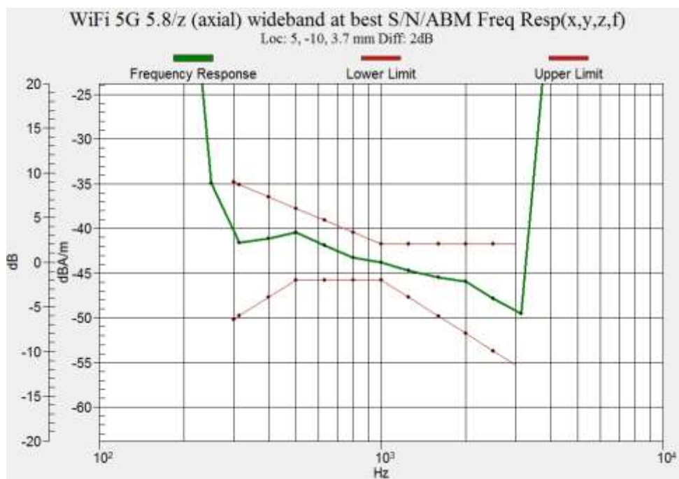
Figure B.24 Frequency Response of WIFI 5.8G
