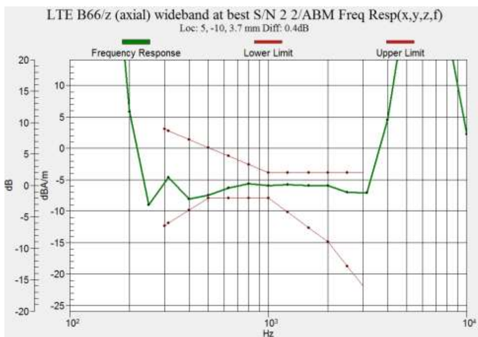
Figure B.42 Frequency Response of LTE B66 (Google Duo)
