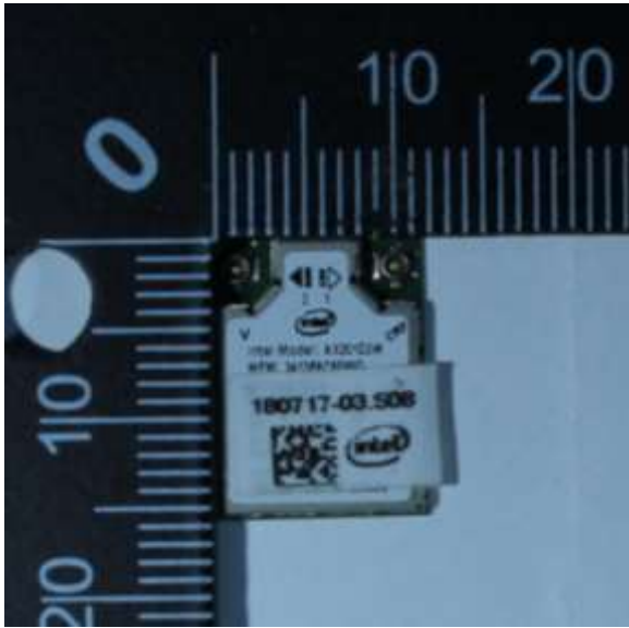
Adapter Front
