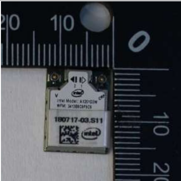
Adapter Front
