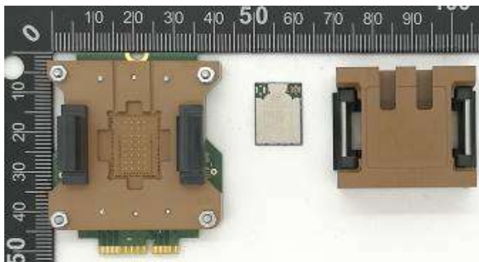
Extender board
