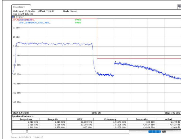
n25 SCS=15kHz DFT_QPSK BW=5MHz HighChannel=382500 RB=25@0
