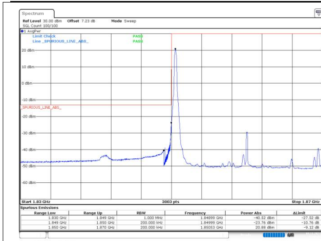
n25 SCS=15kHz DFT_64QAM BW=20MHz LowChannel=372000 RB=1@0
