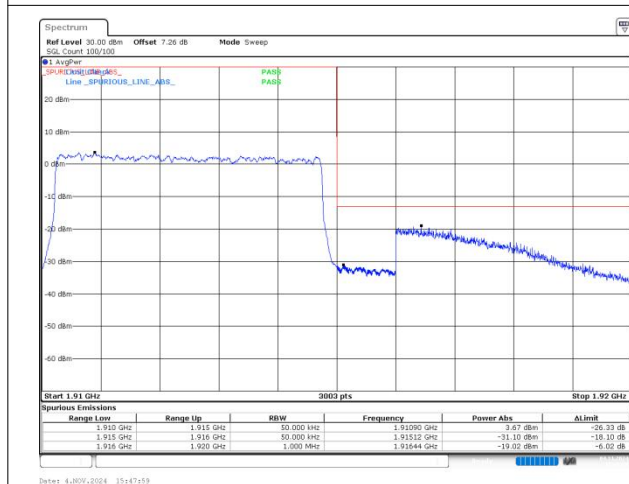
n25 SCS=15kHz DFT_16QAM BW=5MHz HighChannel=382500 RB=25@0
