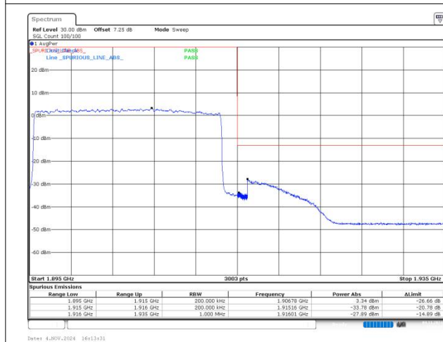
n25 SCS=15kHz DFT_16QAM BW=20MHz HighChannel=381000 RB=100@0
