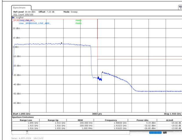
n25 SCS=15kHz DFT_QPSK BW=20MHz HighChannel=381000 RB=100@0
