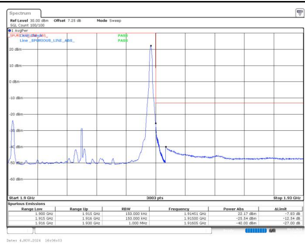
n25 SCS=15kHz DFT_BPSK BW=15MHz HighChannel=381500 RB=1@78
