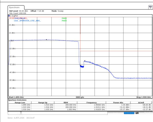
n25 SCS=15kHz CP_QPSK BW=20MHz HighChannel=381000 RB=106@0
