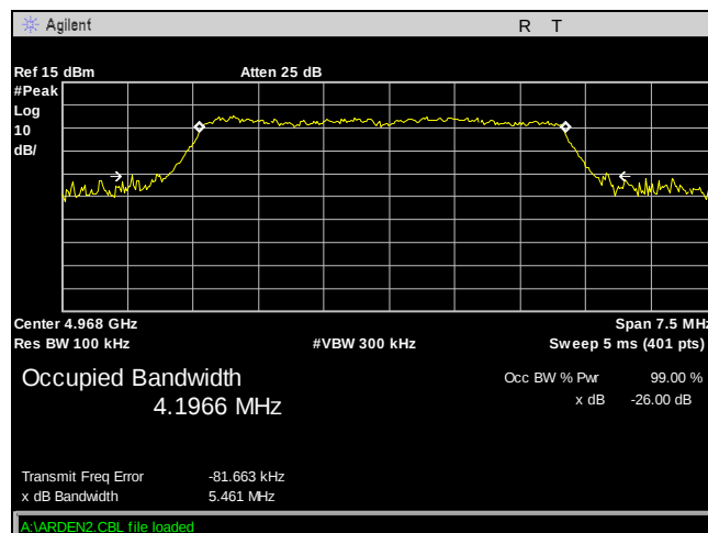
Plot 26. Occupied Bandwidth, Power, BW 5M, Ch. 4967.5M, 16 dB, TP6
