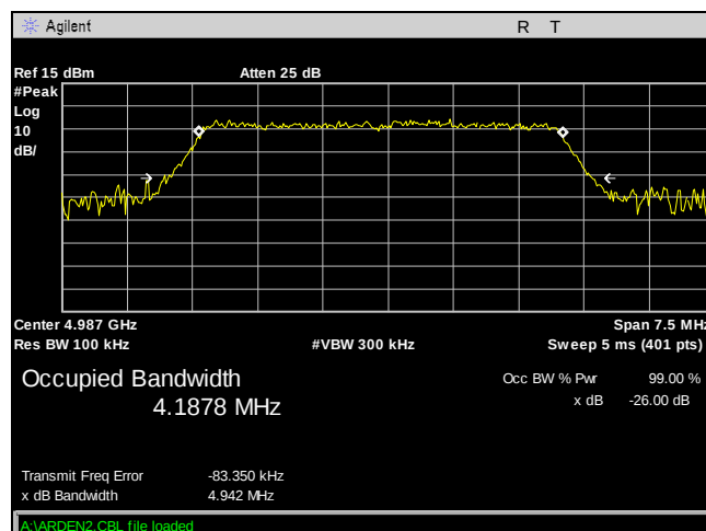
Plot 27. Occupied Bandwidth, Power, BW 5M, Ch. 4987.5M, 16 dB, TP6
