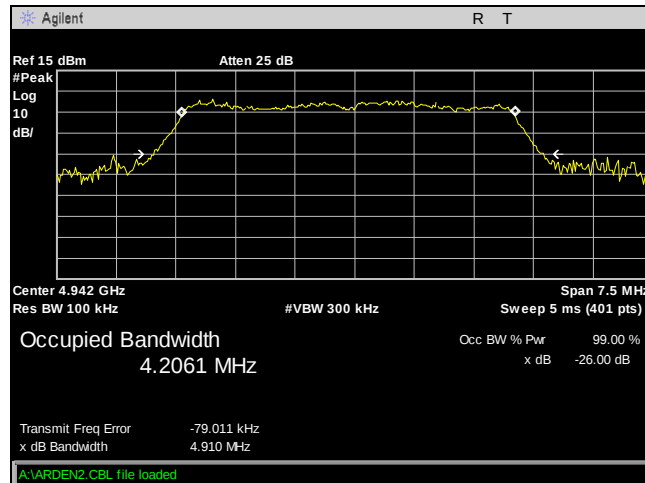
Plot 25. Occupied Bandwidth, Power, BW 5M, Ch. 4942.5M, 16 dB, TP5.5
