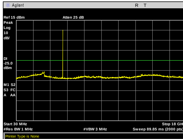
Plot 34. Conducted Spurious Emission 30MHz - 18GHz -25dBm, BW 5M, Ch. 4942.5M, 16 dBi, TP5.5
