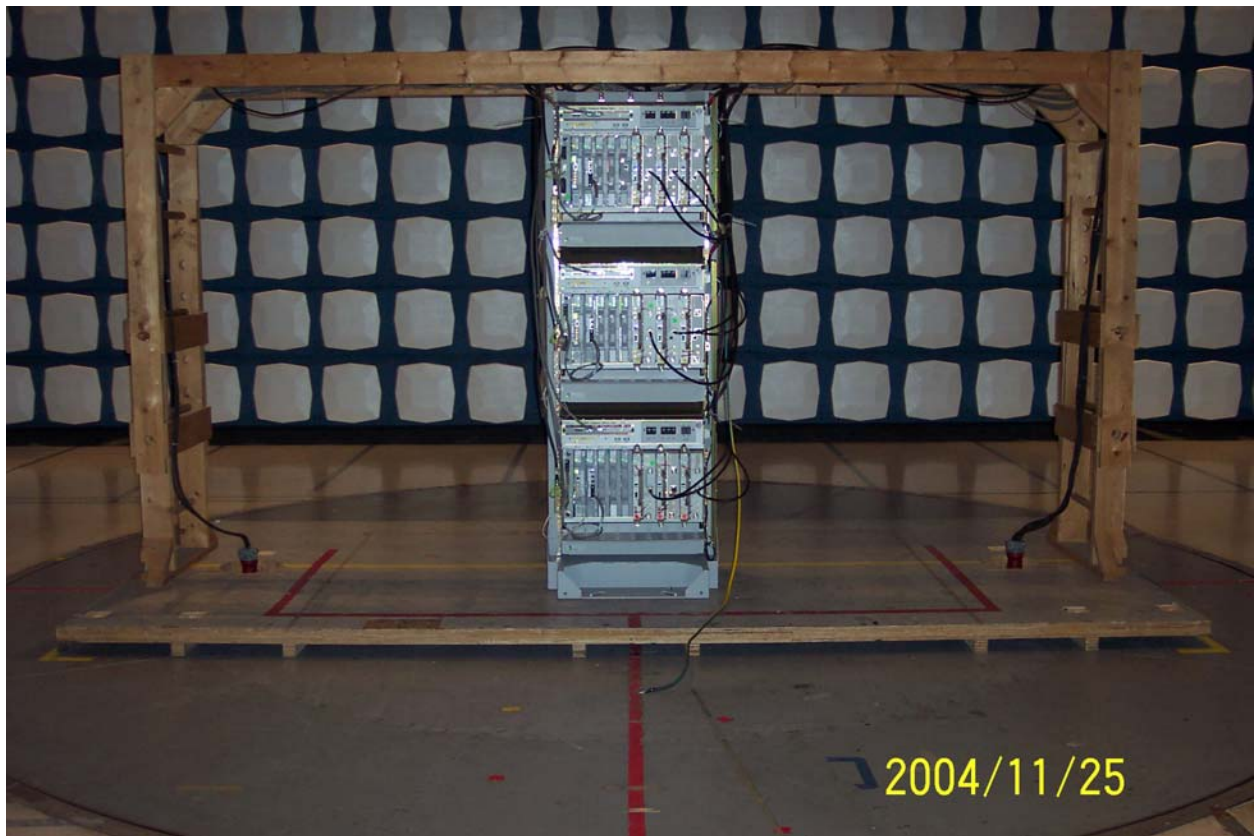
Figure 1 EUT Setup – Front View
