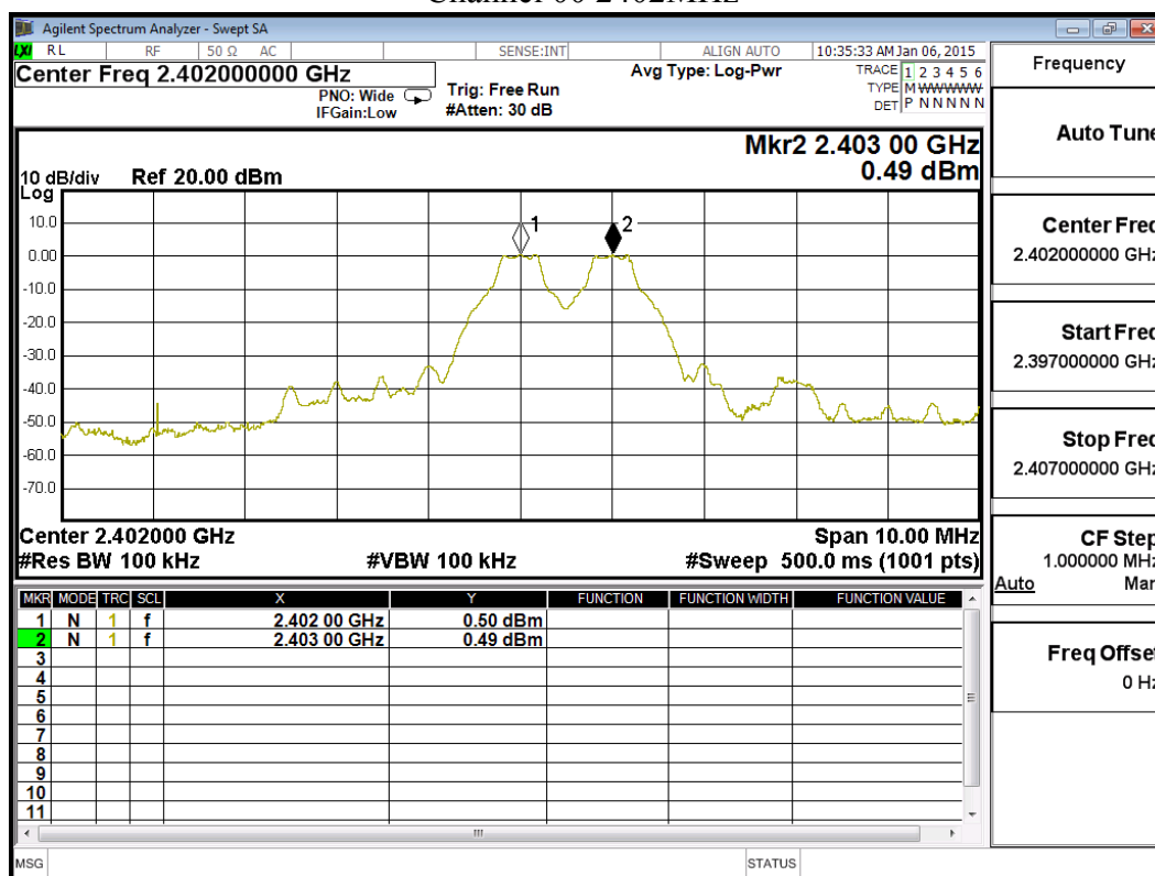
Channel 00 2402MHz
