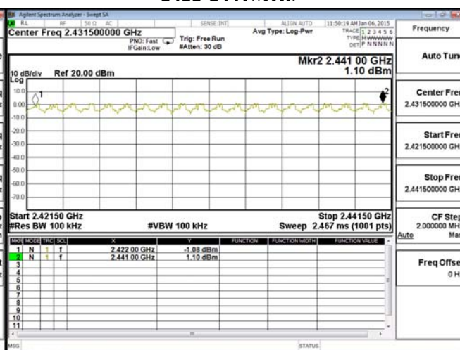
2422-2441MHz
