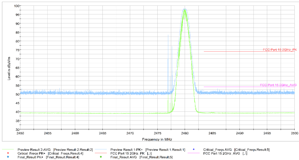
Fig.14. Frequency Band Edges: GFSK, Channel 78, Hopping Off, ch11, 2.45 GHz - 2.50GHz
