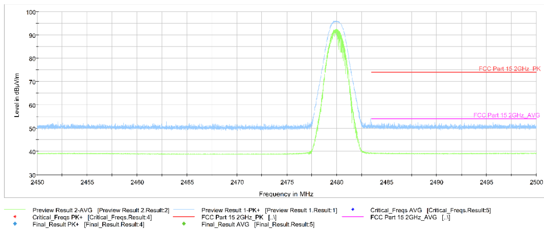
Fig.18. Frequency Band Edges: 8DPSK, Channel 78, 2.45 GHz - 2.50GHz
