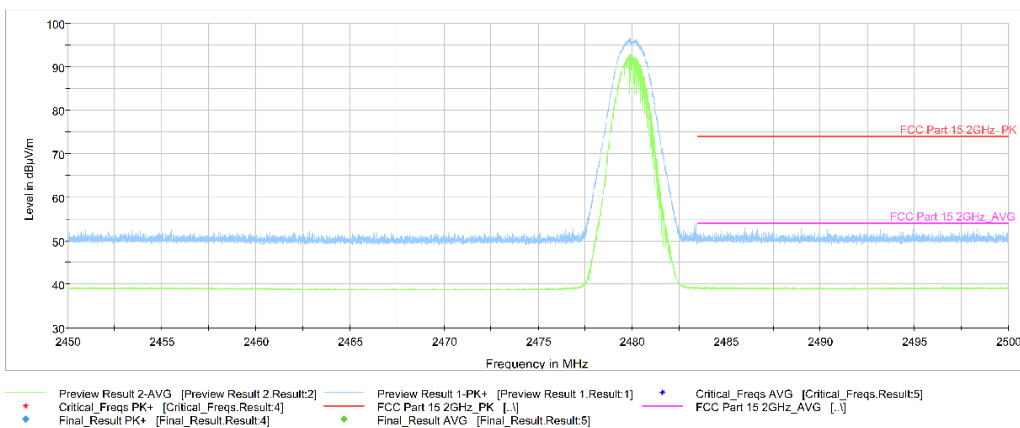
Fig.16. Frequency Band Edges: \pi/4 DQPSK, Channel 78, Hopping Off, 2.45 GHz - 2.50GHz
