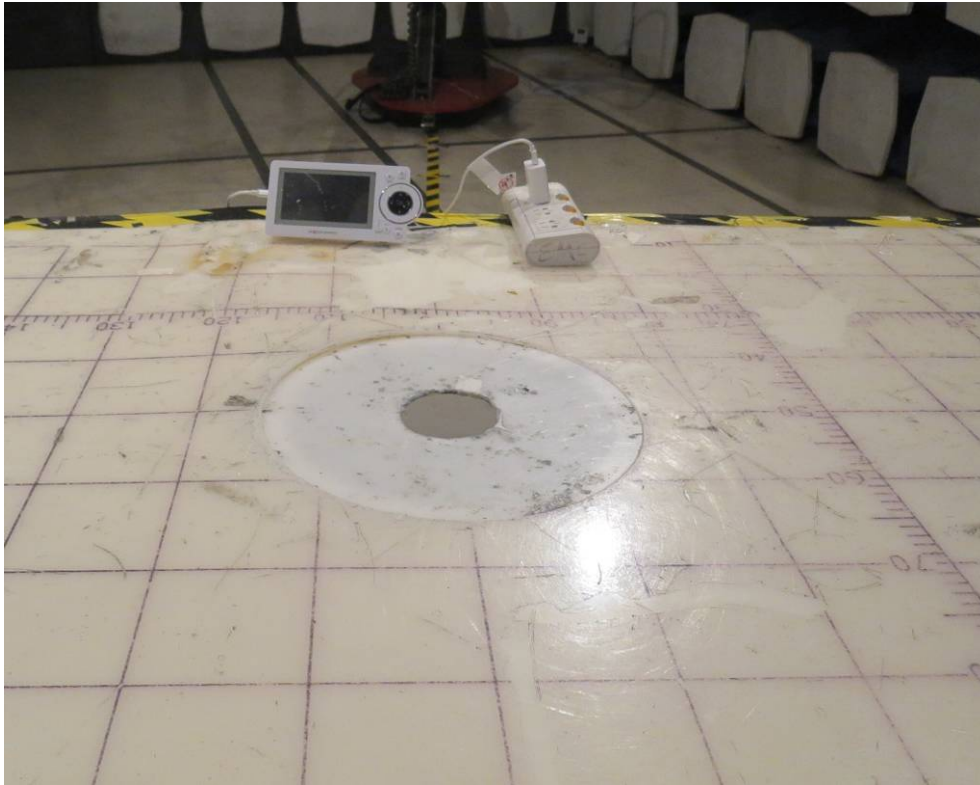
Test Setup Photo – Radiated Emission Below 1G
