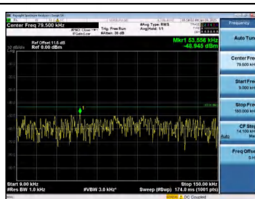
Band66-10MHz-16QAM-132622-50RB#0-0.009~ 0.15-PASS
