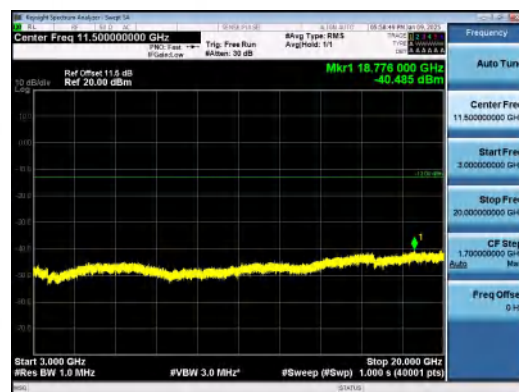
Band66-10MHz-16QAM-132622-50RB#0-3000~ 20000-PASS
