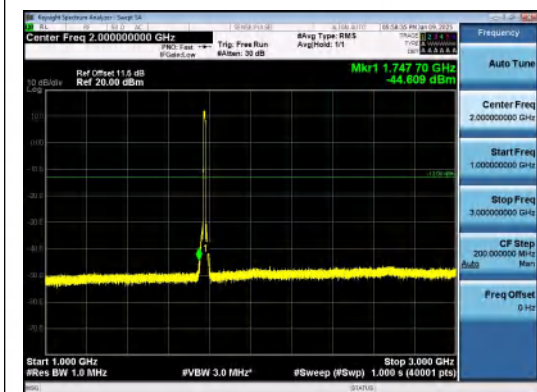
Band66-10MHz-16QAM-132622-50RB#0-1000~ 3000-PASS
