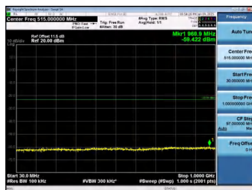
Band66-10MHz-16QAM-132622-50RB#0-30~10 00-PASS
