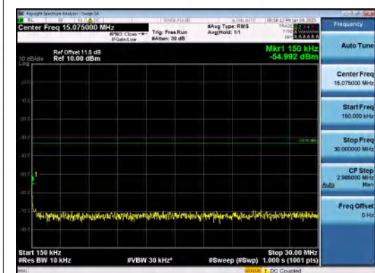
Band66-10MHz-16QAM-132622-50RB#0-0.15~3 0-PASS
