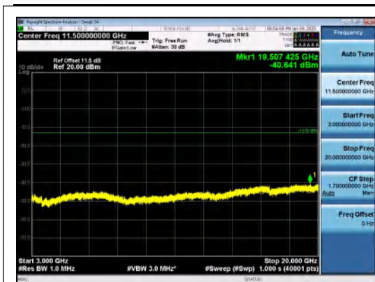
Band66-10MHz-16QAM-132622-1RB#49-3000~ 20000-PASS
