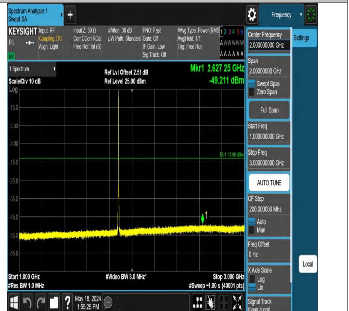
Band2_3MHz_QPSK_18900_1RB#0_1000~3000_1000~3000
