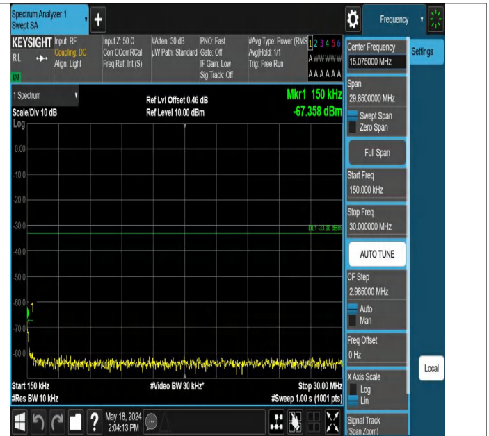
Band2_5MHz_QPSK_19175_1RB#0_0.15~30_0.15~30
