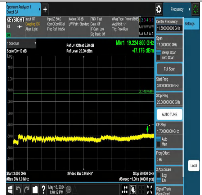
Band2_1.4MHz_QPSK_18900_1RB#5_3000~20000_3000~20000
