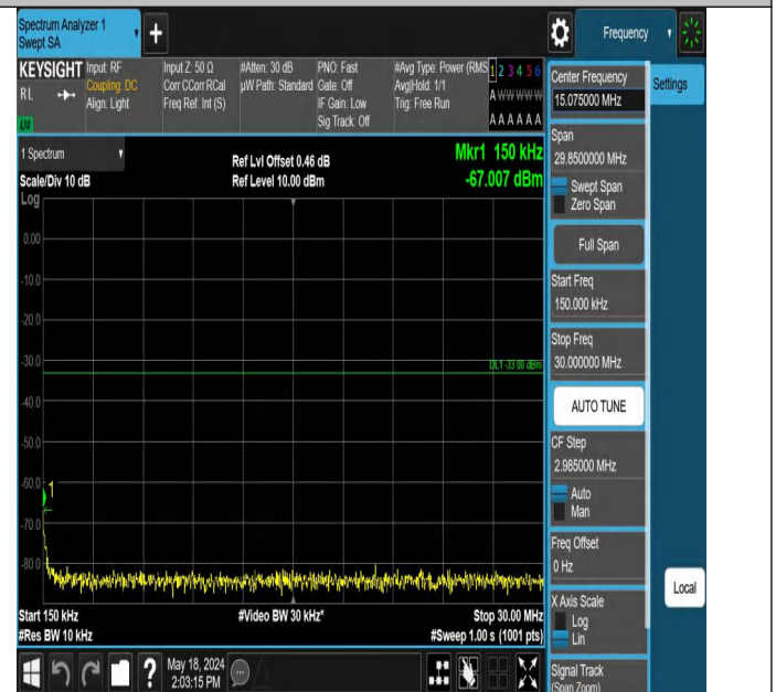
Band2_5MHz_QPSK_18900_1RB#0_0.15~30_0.15~30
