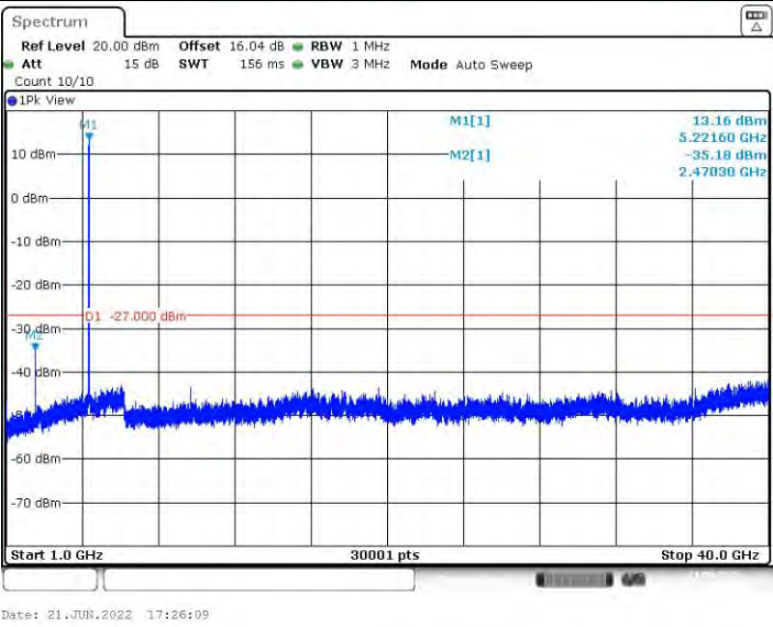
11A_Ant1_5220_1000~40000
