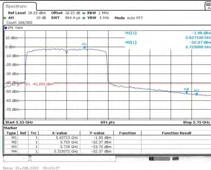
11AC80MIMO_Ant1_High_5610_AV
