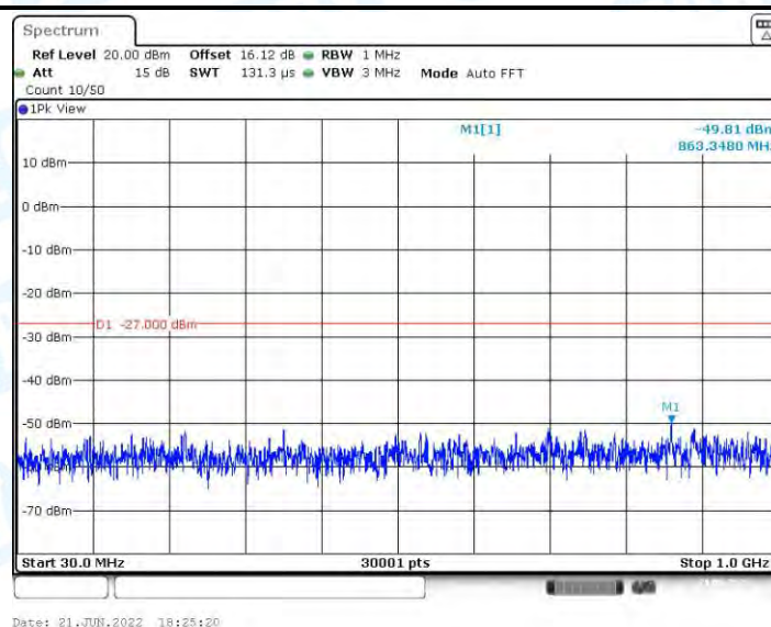
11A_Ant2_5220_30~1000
