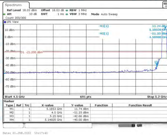
11N20MIMO_Ant1_Low_5180_Peak
