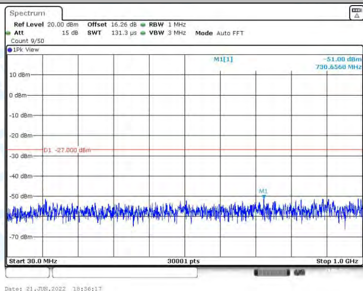
11A_Ant2_5240_30~1000
