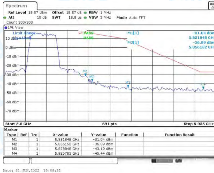
11A_Ant2_High_5825
