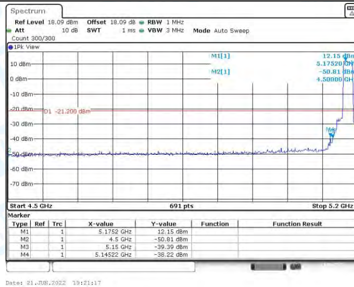
11N20MIMO_Ant2_Low_5180_Peak
