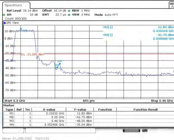
11N20MIMO_Ant1_High_5320_Peak
