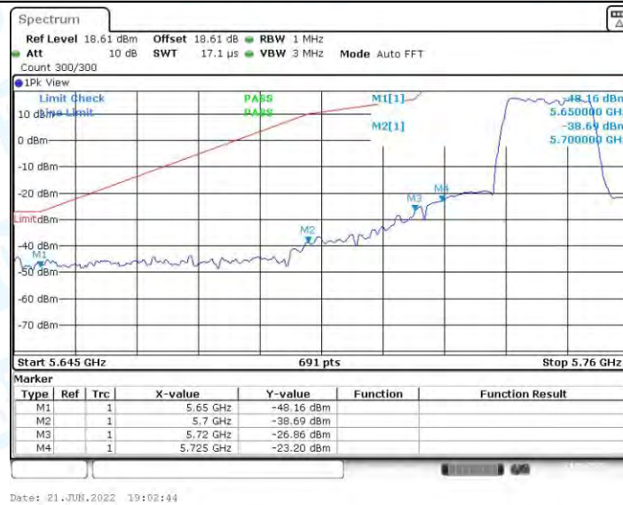
11A_Ant2_Low_5745_Peak
