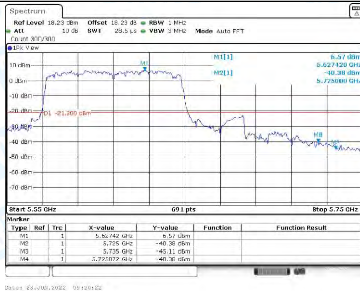
11AC80MIMO_Ant1_High_5610_Peak
