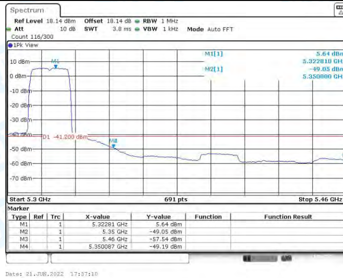
11A_Ant1_High_5320_AV
