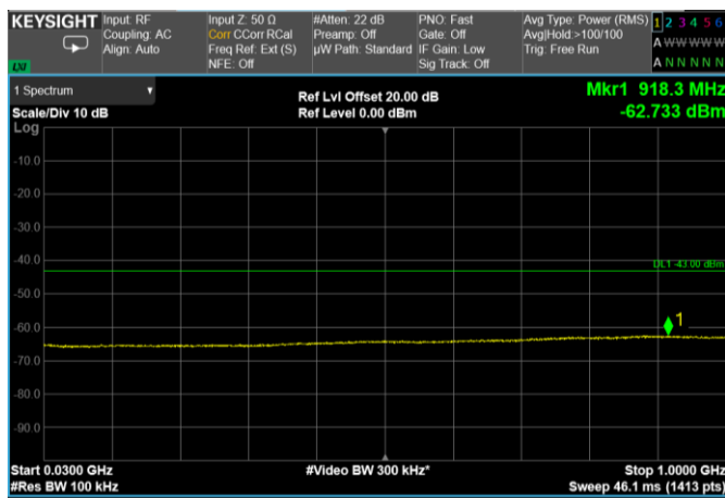
Channel: MIDDLE, Modulation: 64QAM, BW=60MHz, Range: 30 MHz – 1000 MHz
