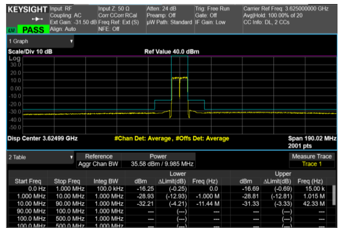
Middle Band Edge, 2 Carrier, Modulation: 64QAM, BW=5MHz
