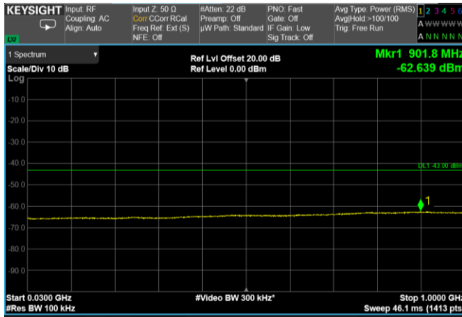
Channel: TOP, Modulation: 64QAM, BW=40MHz, Range: 30 MHz – 1000 MHz
