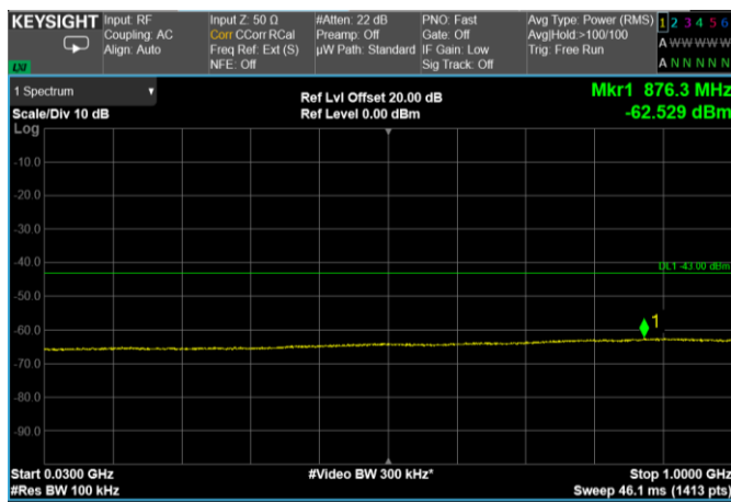
Channel: MIDDLE, Modulation: 64QAM, BW=40MHz, Range: 30 MHz – 1000 MHz
