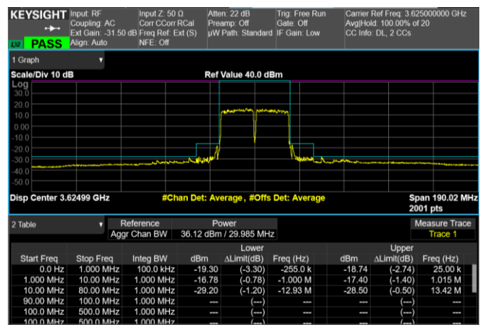
Middle Band Edge, 2 Carrier, Modulation: 64QAM, BW=15MHz
