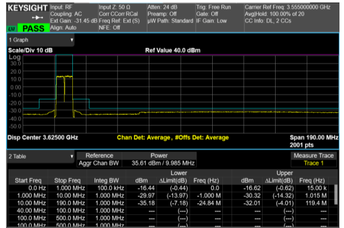
Low Band Edge, 2 Carrier, Modulation: 64QAM, BW=5MHz
