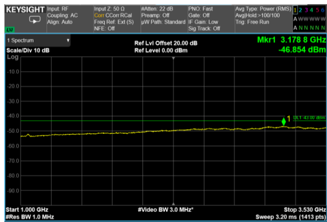
Channel: MIDDLE, Modulation: 64QAM, BW=40MHz, Range: 1000 MHz – 3530 MHz
