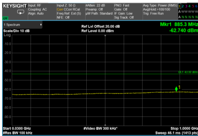
Channel: TOP, Modulation: 64QAM, BW=50MHz, Range: 30 MHz – 1000 MHz
