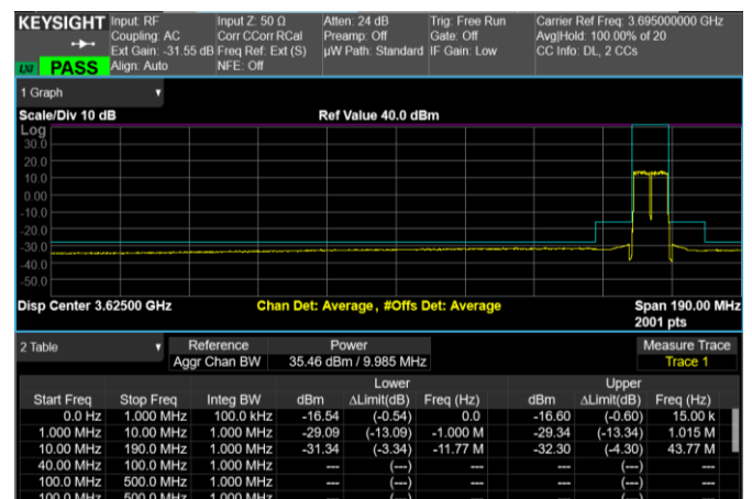
High Band Edge, 2 Carrier, Modulation: 64QAM, BW=5MHz
