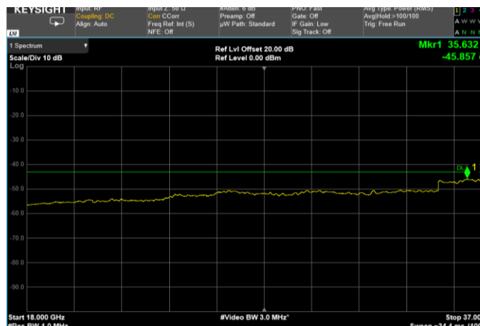
Channel: MIDDLE, Modulation: 64QAM, BW=40MHz, Range: 18 GHz – 37 GHz
