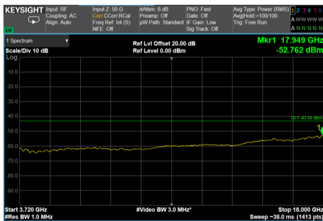
Channel: MIDDLE, Modulation: 64QAM, BW=40MHz, Range: 3720 MHz – 18 GHz
