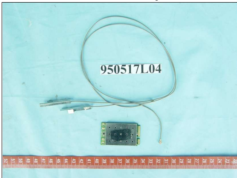
PIFA Antenna with 1.08dBi gain
