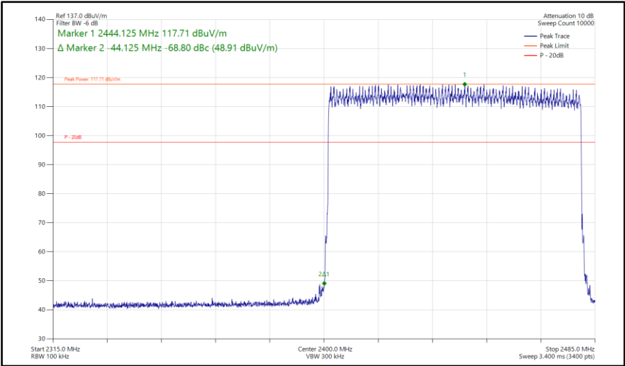
Figure 249 - Bluetooth 3-DH5, SISO, Core 1 - Hopping Band Edge Frequency 2400 MHz
