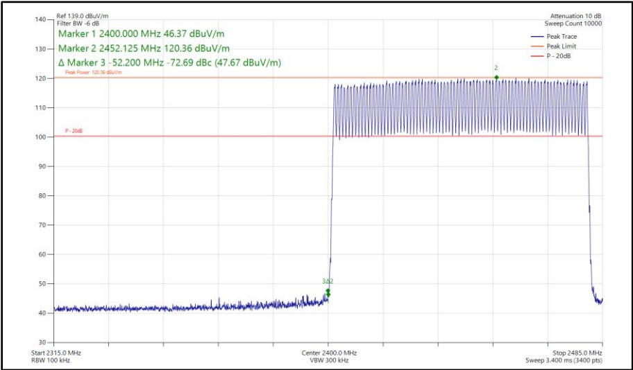
Figure 253 - Bluetooth DH5, MIMO, Core 0 - Core 1 - Hopping Band Edge Frequency 2400 MHz
