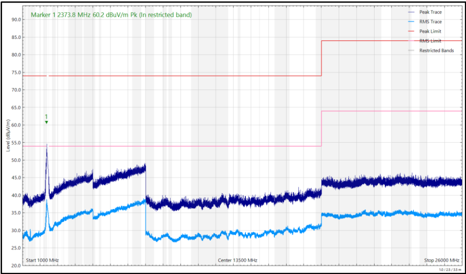
Figure 257 - 2402 MHz (CH0), DH5, ePA, Core 0 + Core 1, 1 GHz to 26 GHz, Horizontal
