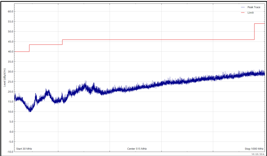
Figure 259 - 2441 MHz (CH39), DH5, ePA, Core 0 + Core 1, 30 MHz to 1 GHz, Horizontal (Peak)
