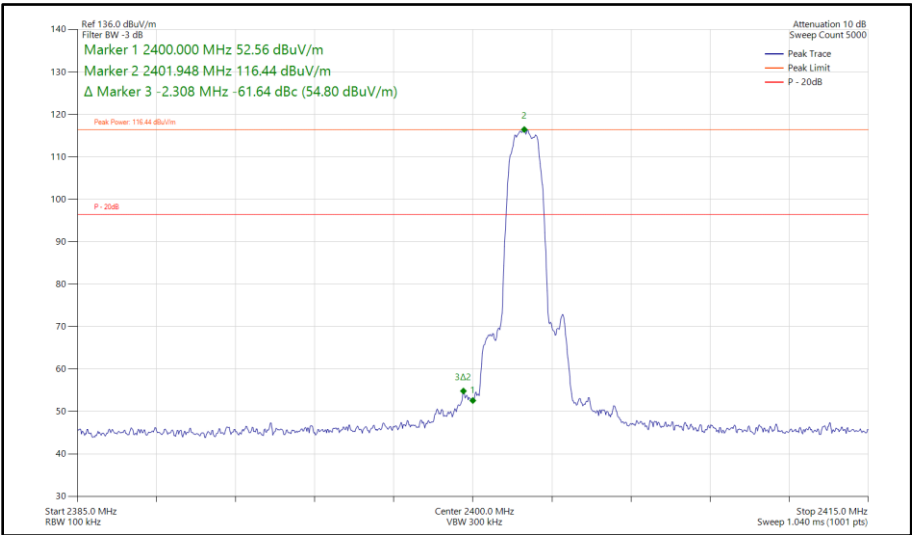
Figure 252 - Bluetooth 3-DH5, MIMO, Core 0 - Core 1 - 2402 MHz Band Edge Frequency 2400 MHz
