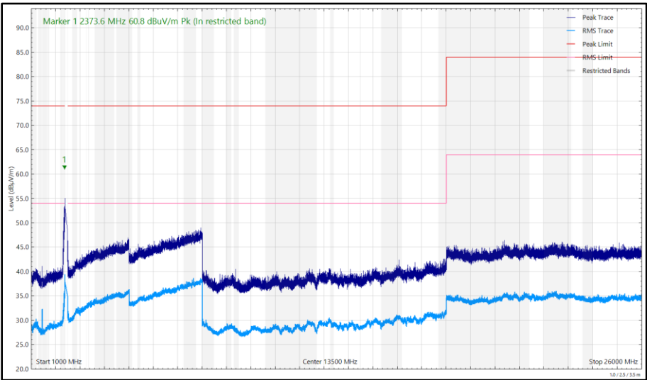
Figure 258 - 2402 MHz (CH0), DH5, ePA, Core 0 + Core 1, 1 GHz to 26 GHz, Vertical
