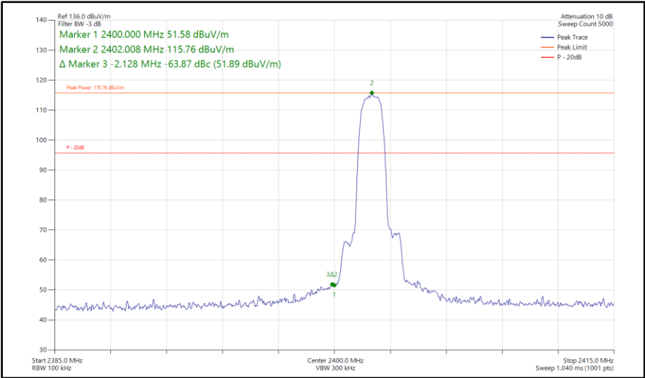
Figure 245 - Bluetooth 2-DH5, SISO, Core 1 - 2402 MHz Band Edge Frequency 2400 MHz
