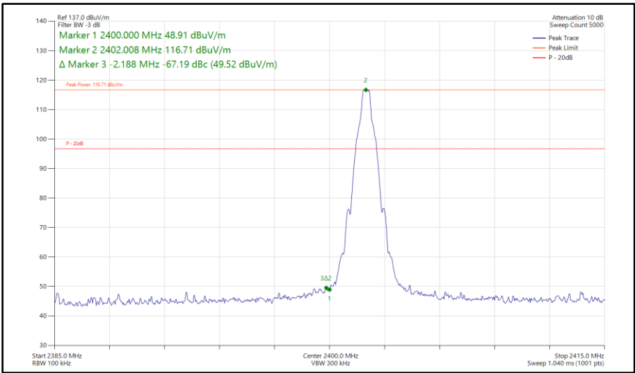
Figure 244 - Bluetooth DH5, SISO, Core 1 - 2402 MHz Band Edge Frequency 2400 MHz
