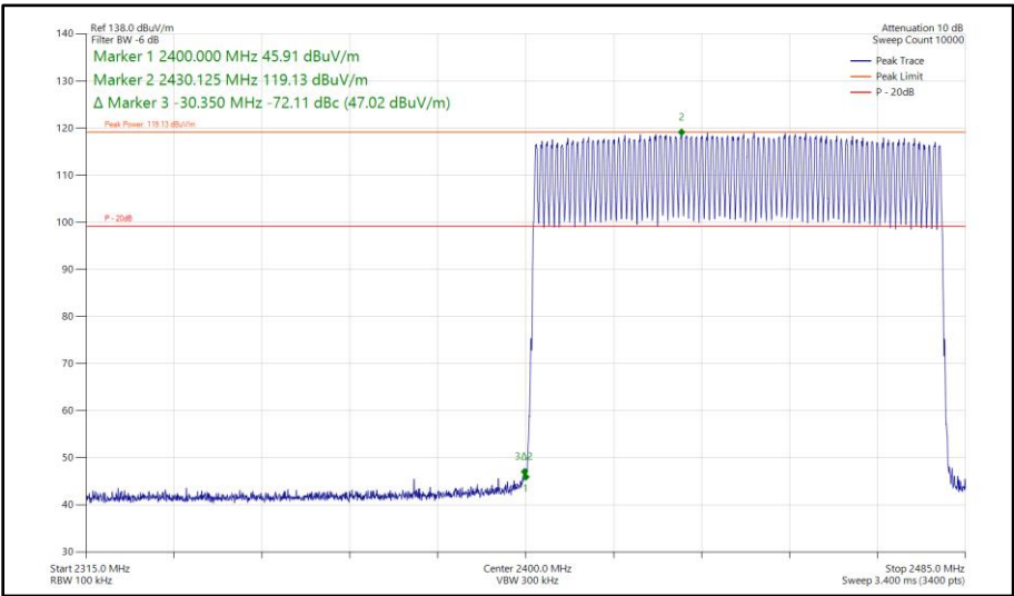
Figure 247 - Bluetooth DH5, SISO, Core 1 - Hopping Band Edge Frequency 2400 MHz
