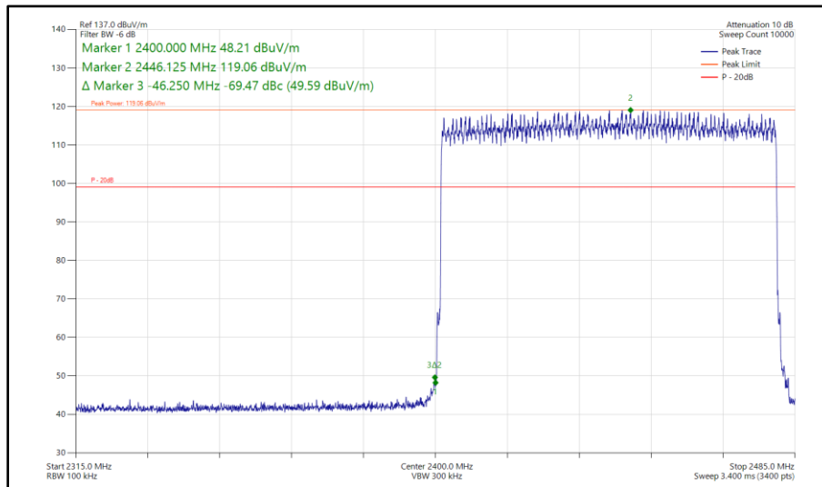
Figure 255 - Bluetooth 3-DH5, MIMO, Core 0 - Core 1 - Hopping Band Edge Frequency 2400 MHz
