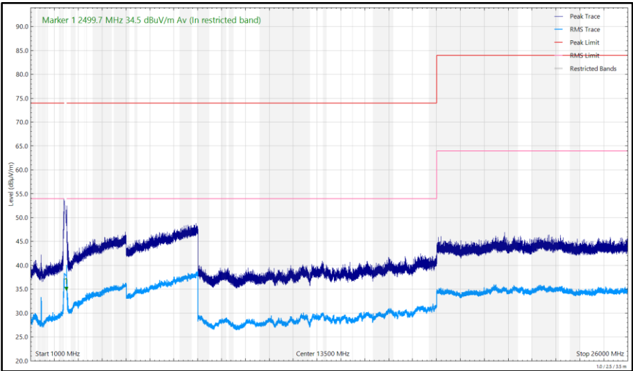
Figure 264 - 2480 MHz (CH78), DH5, ePA, Core 0 + Core 1, 1 GHz to 26 GHz, Vertical
