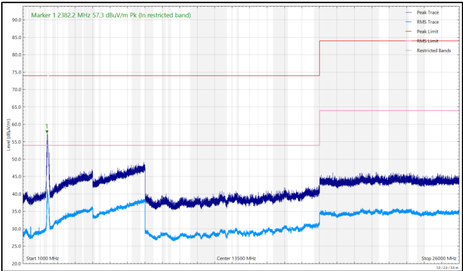
Figure 262 - 2441 MHz (CH39), DH5, ePA, Core 0 + Core 1, 1 GHz to 26 GHz, Vertical
