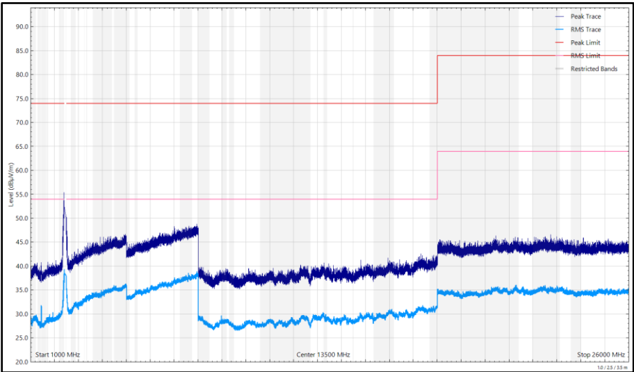
Figure 260 - 2441 MHz (CH39), DH5, ePA, Core 0 + Core 1, 1 GHz to 26 GHz, Horizontal
