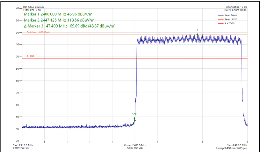
Figure 254 - Bluetooth 2-DH5, MIMO, Core 0 - Core 1 - Hopping Band Edge Frequency 2400 MHz
