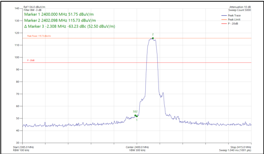
Figure 246 - Bluetooth 3-DH5, SISO, Core 1 - 2402 MHz Band Edge Frequency 2400 MHz
