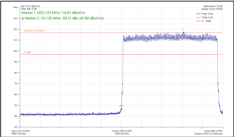
Figure 248 - Bluetooth 2-DH5, SISO, Core 1 - Hopping Band Edge Frequency 2400 MHz
