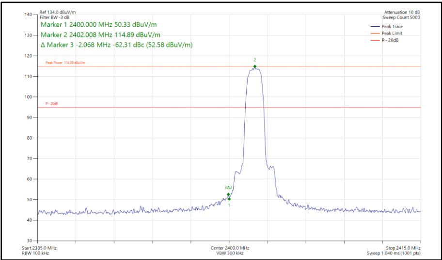
Figure 251 - Bluetooth 2-DH5, MIMO, Core 0 - Core 1 - 2402 MHz Band Edge Frequency 2400 MHz
