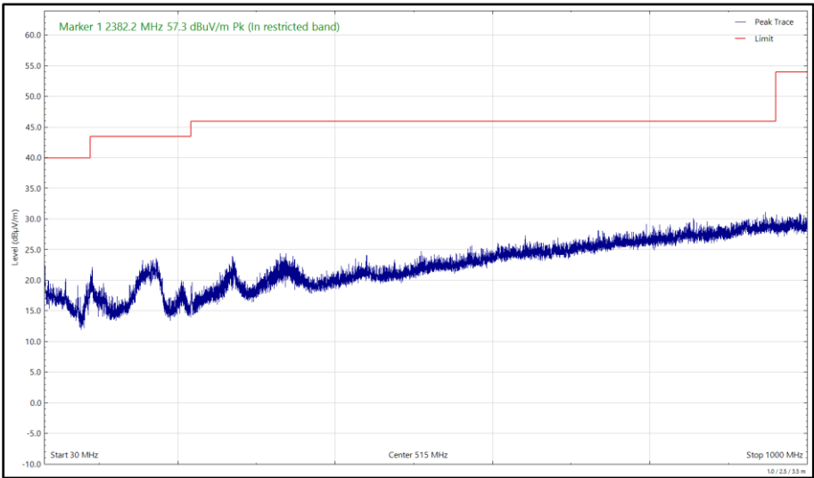
Figure 261 - 2441 MHz (CH39), DH5, ePA, Core 0 + Core 1, 30 MHz to 1 GHz, Vertical (Peak)
