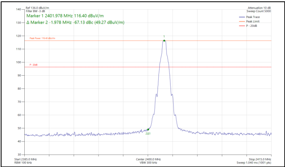
Figure 250 - Bluetooth DH5, MIMO, Core 0 - Core 1 - 2402 MHz Band Edge Frequency 2400 MHz
