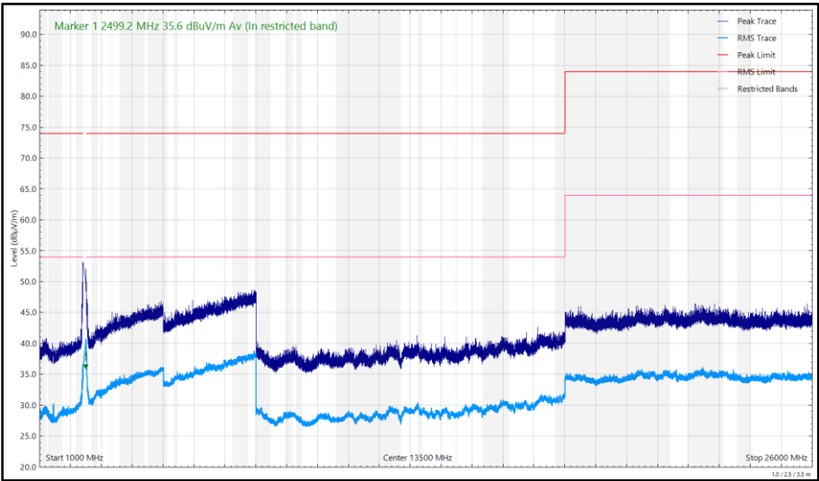
Figure 263 - 2480 MHz (CH78), DH5, ePA, Core 0 + Core 1, 1 GHz to 26 GHz, Horizontal
