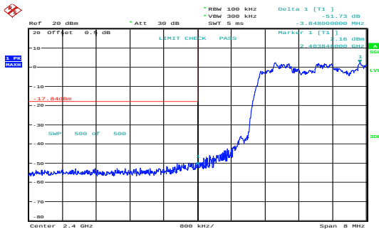
\pi/4 -DQPSK_Hopping_Lower 51.73dB
