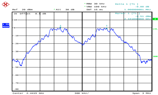
GFSK_Middle 1.001MHz
