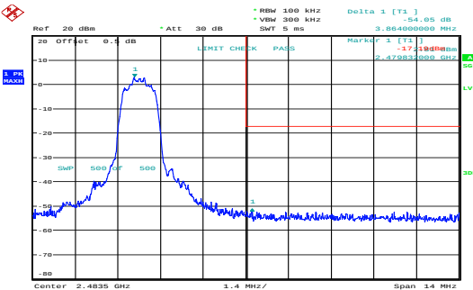
8DPSK_High 54.05dB
