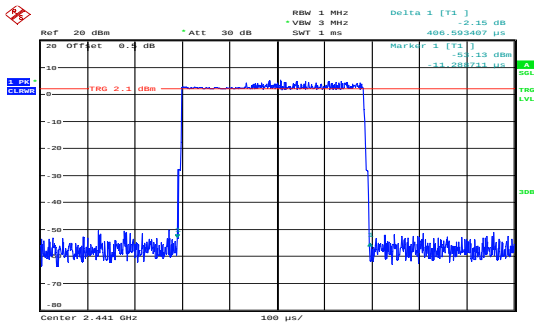
8DPSK_Hopping_3DH1 0.407ms
