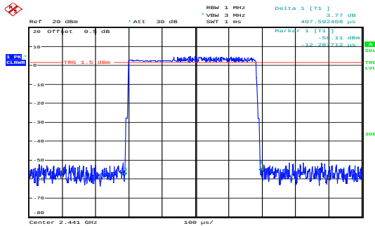
\pi/4 -DQPSK_Hopping_2DH1 0.408ms
