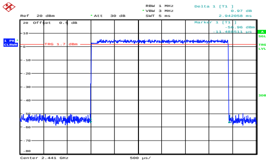
8DPSK_Hopping_3DH5 2.942ms
