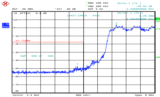
8DPSK_Hopping_Lower 49.92dB
