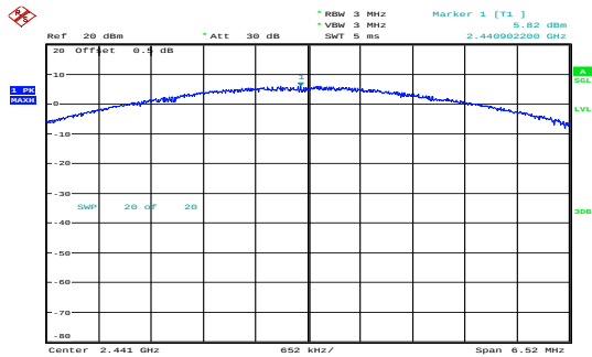
8DPSK_Middle 5.82dBm
