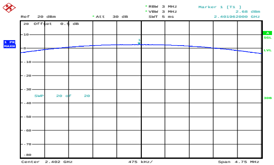
GFSK_Low 2.68dBm
