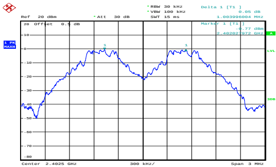
GFSK_Low 1.004MHz
