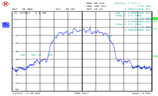
\pi/4 -DQPSK_High 1.176MHz
