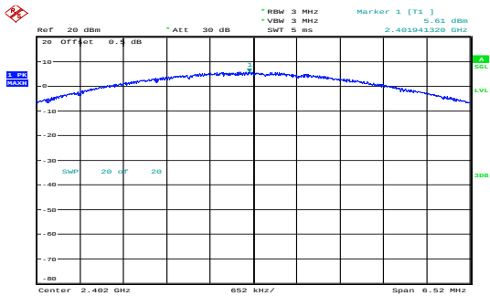
8DPSK_Low 5.61dBm
