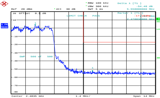
8DPSK_Hopping_Upper 54.48dB
