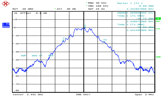
GFSK_Middle 0.864MHz
