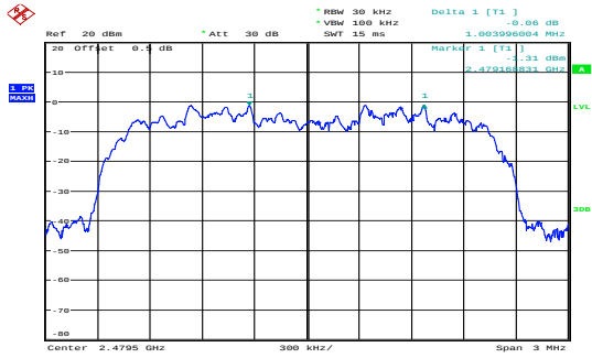
\pi/4 -DQPSK_High 1.004MHz
