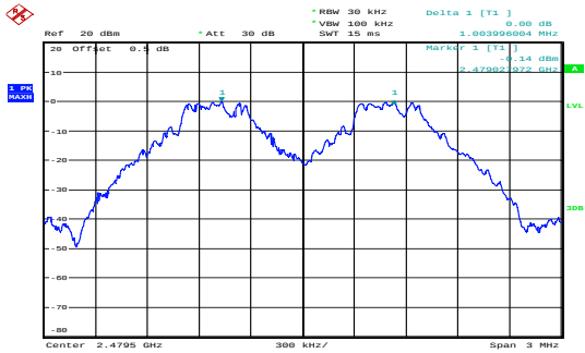
GFSK_High 1.004MHz
