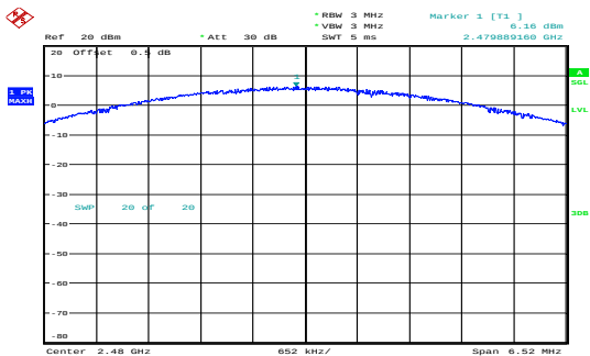
8DPSK_High 6.16dBm
