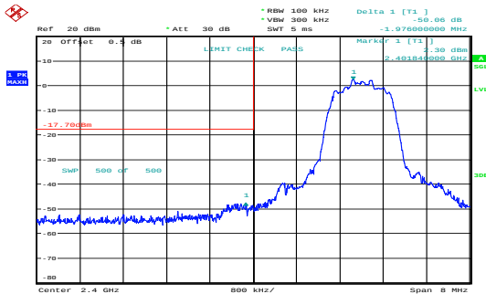
8DPSK_Low 50.06dB
