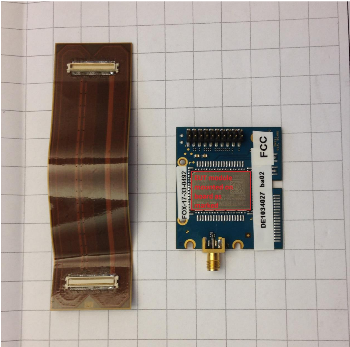
Photo3: Flex Adapter and Module
