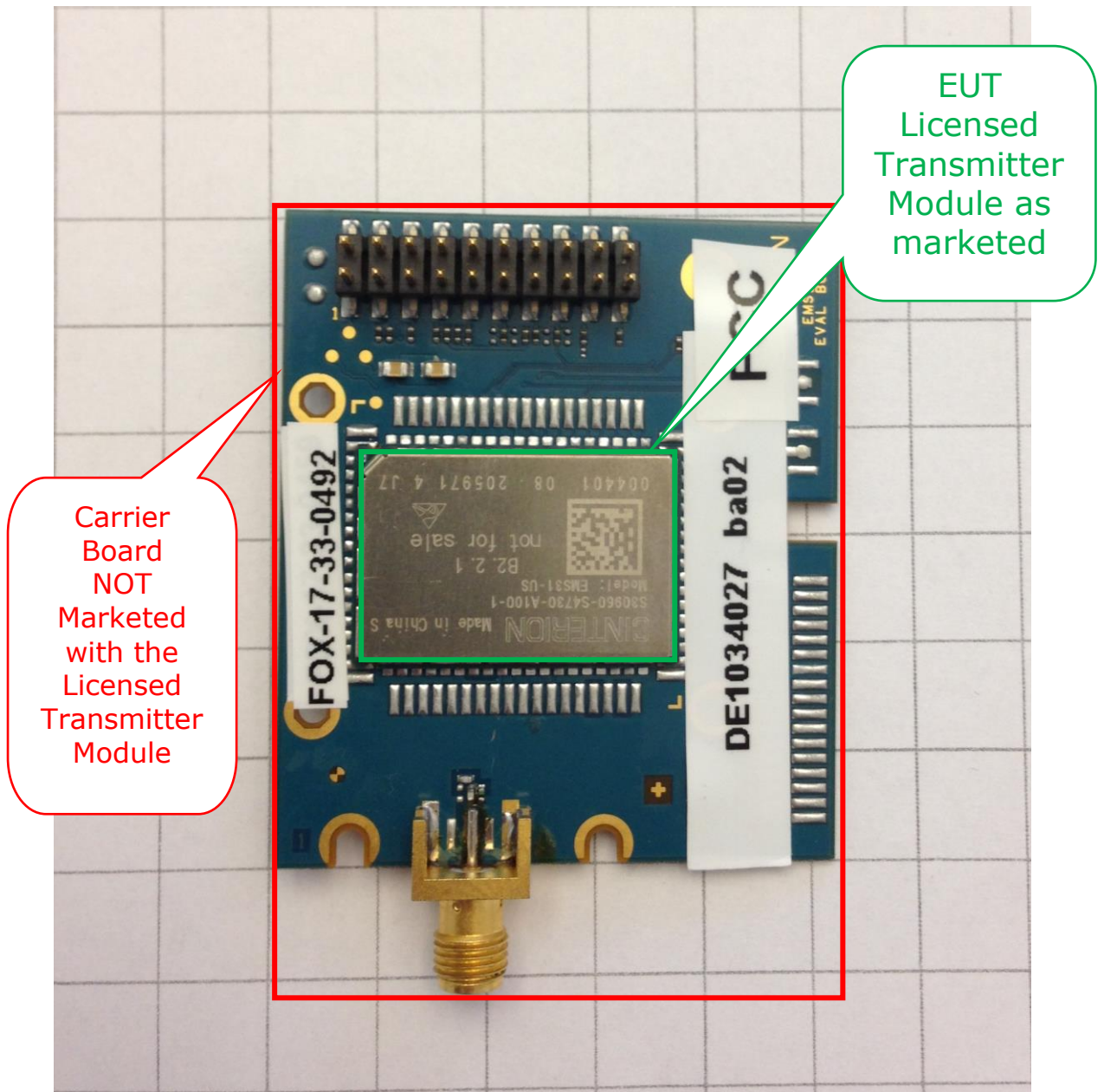
Photo 4: Module with Antenna port
