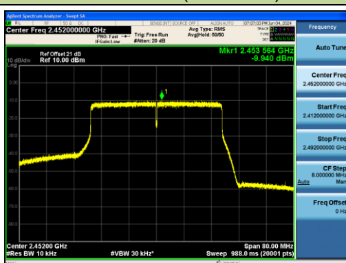
Channel 09 (2452MHz)
