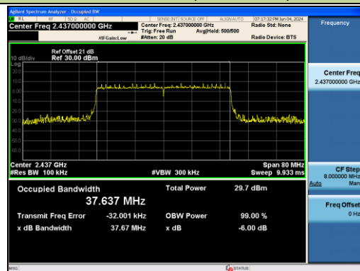
Channel 06 (2437MHz)
