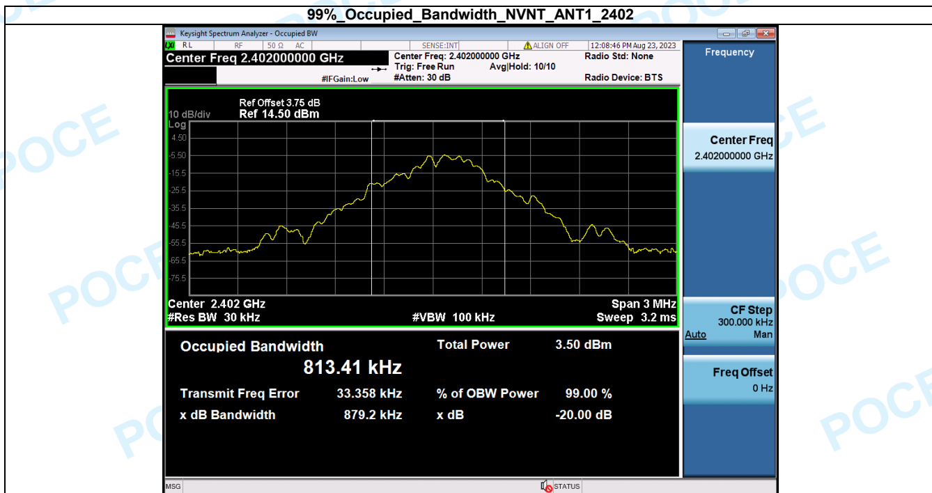
99%_Occupied_Bandwidth_NVNT_ANT1_2402
