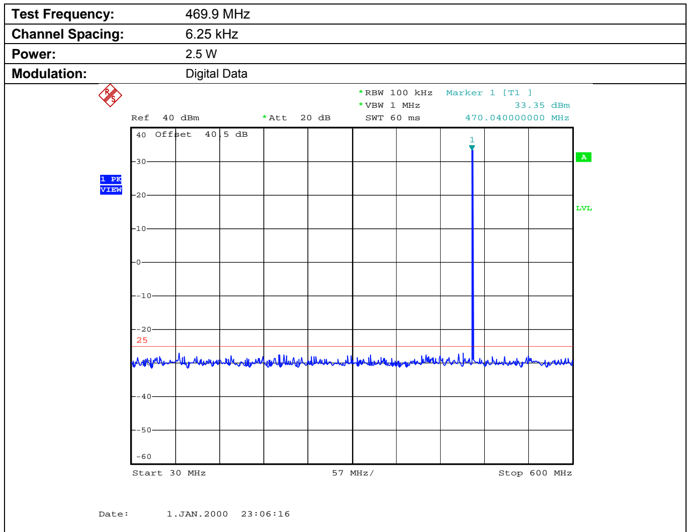
Plot 5.8.4.3.3. Conducted Transmitter Spurious Emissions for 469.9 MHz, Low Power, 30 MHz - 600 MHz
