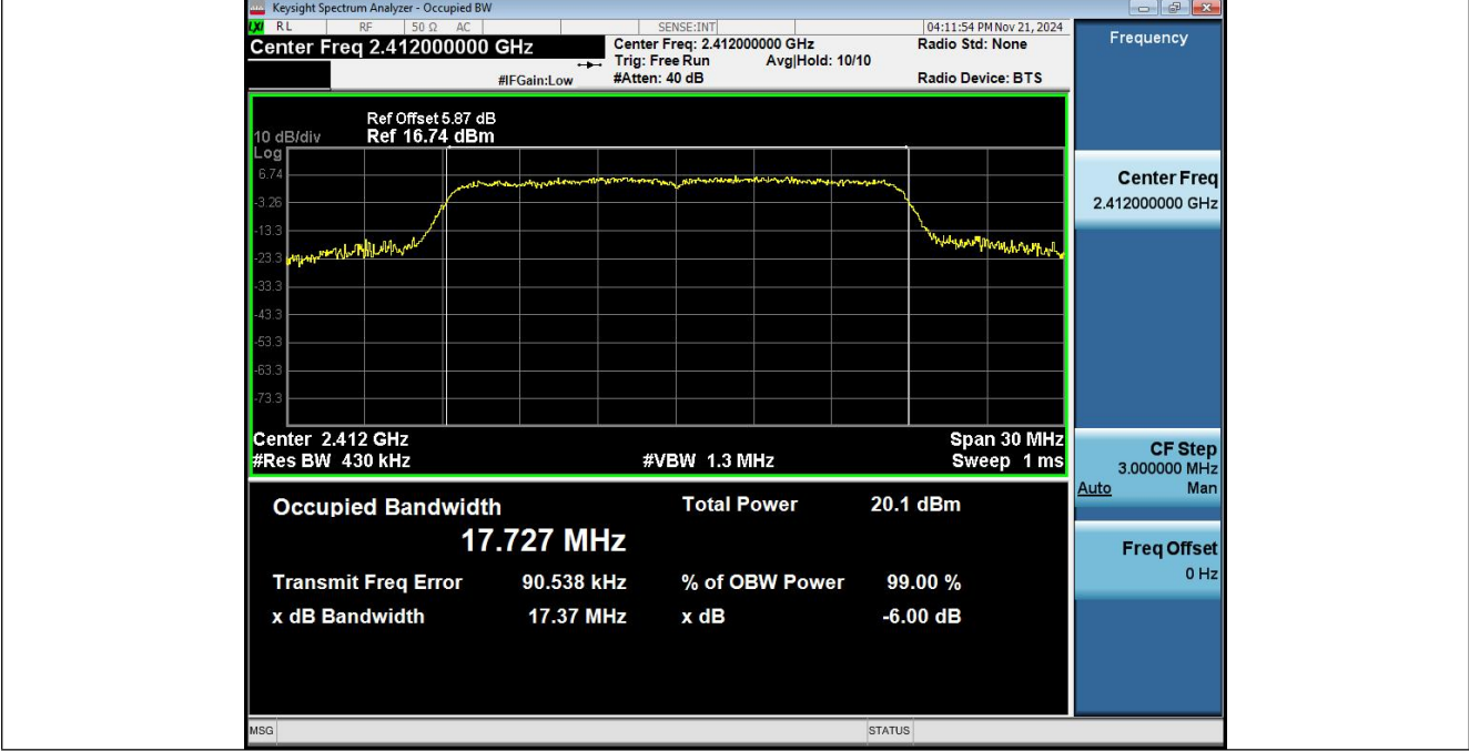
-6dB_Bandwidth_NVNT_ANT1_802_11n(HT20)_2412
