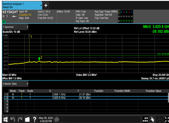
N38(15M)_DFT-s- OFDM_QPSK_Edge_1RB_Left_High_CH
