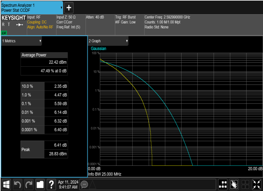
N41(20M)_DFT-s-OFDM_QPSK_Outer_Full_Mid_CH
