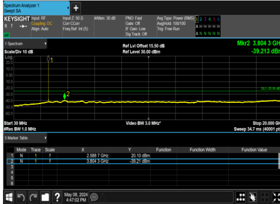
N38(15M)_DFT-s- OFDM_QPSK_Edge_1RB_Left_Mid_CH
