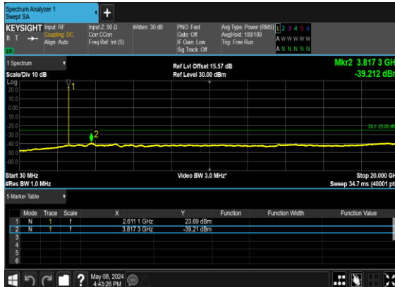
N38(10M)_DFT-s- OFDM_QPSK_Edge_1RB_Left_High_CH
