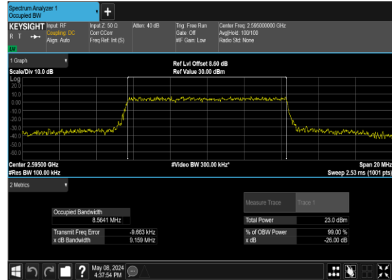
N38(10M)_CP-OFDM_256 QAM_Outer_Full_Mid_CH
