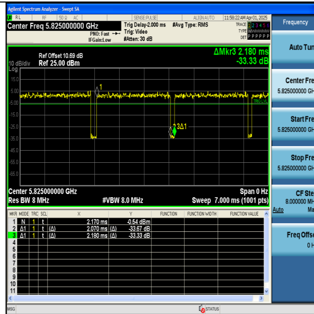
NTNV-11A-Ant2-5825
