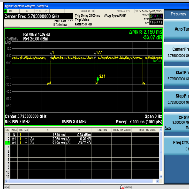
NTNV-11A-Ant2-5785
