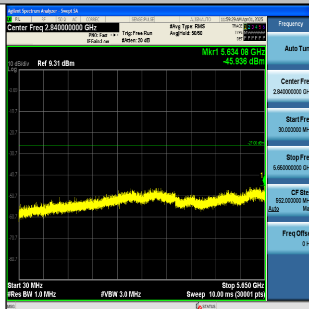
11A-Ant2-5825-30~5650-PASS
