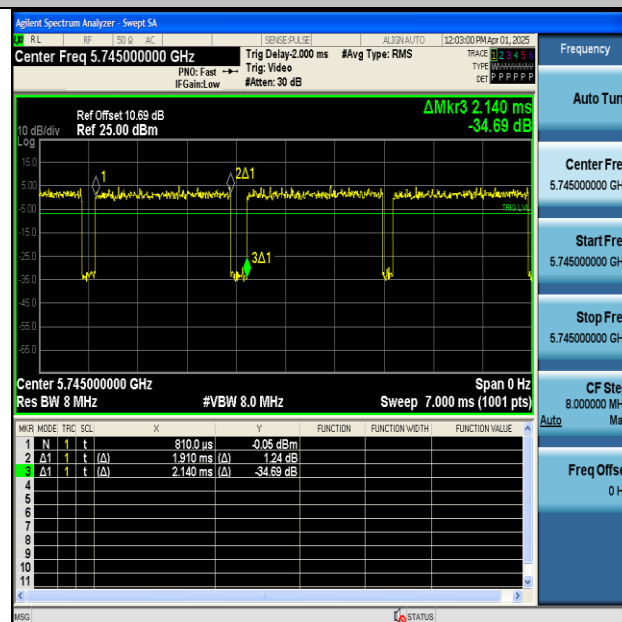
NTNV-11N20MIMO-Ant2-5745
