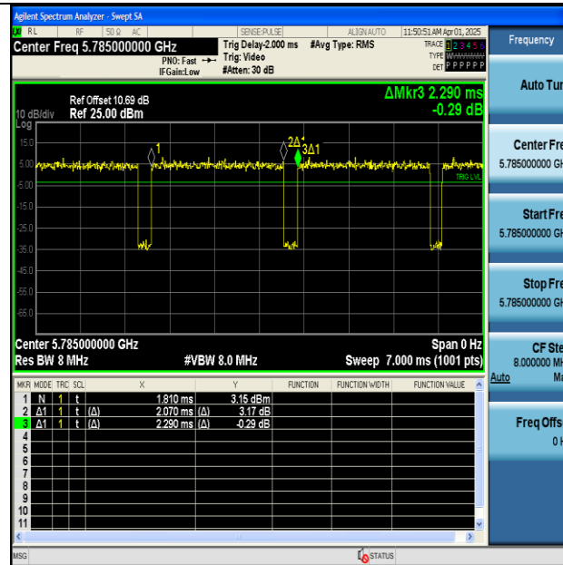
NTNV-11A-Ant1-5785
