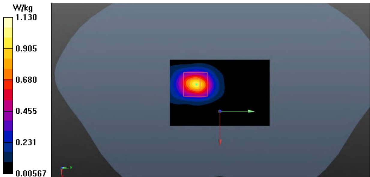
Fig.22 LTE Band 41 Body
