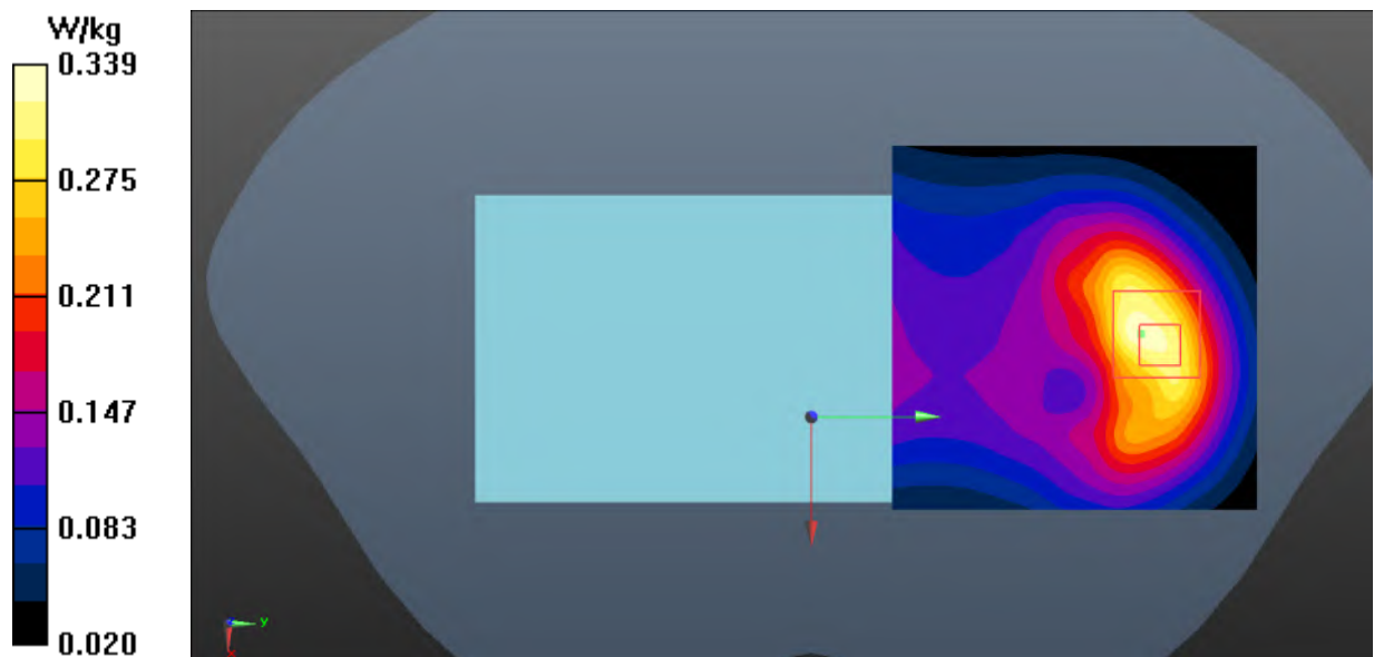
Fig.18 LTE Band 26 Body
