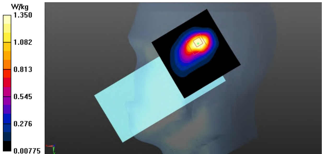
Fig.21 LTE Band 41 Head
