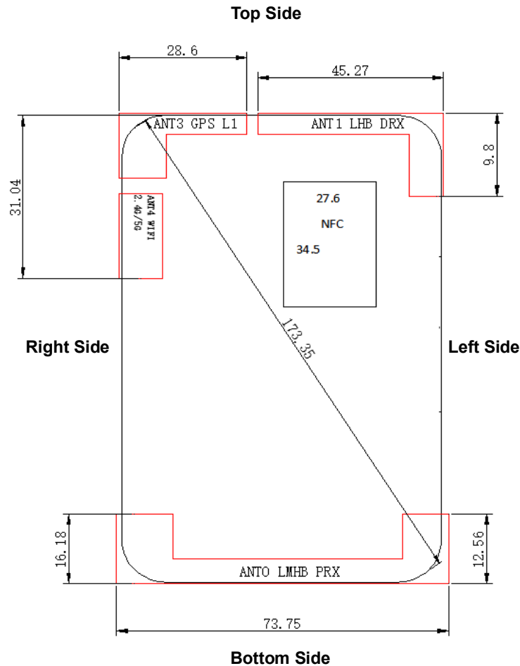
Picture 11.1 Antenna Locations (Back View)
