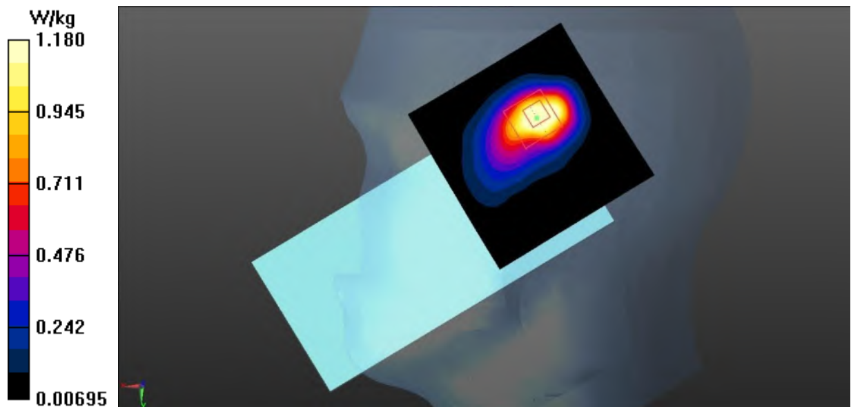
Fig.19 LTE Band 38 Head
