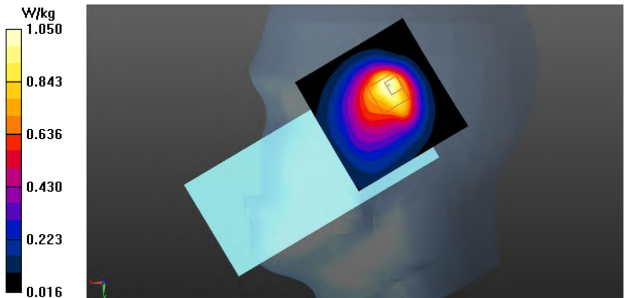
Fig.17 LTE Band 26 Head
