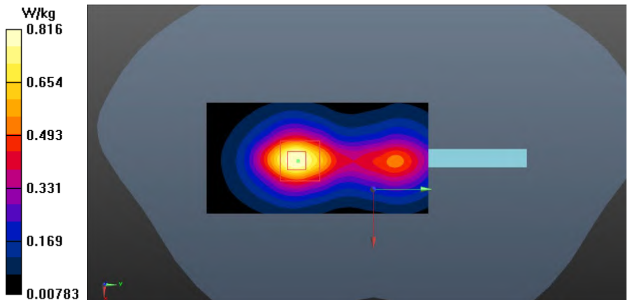
Fig.20 LTE Band 38 Body
