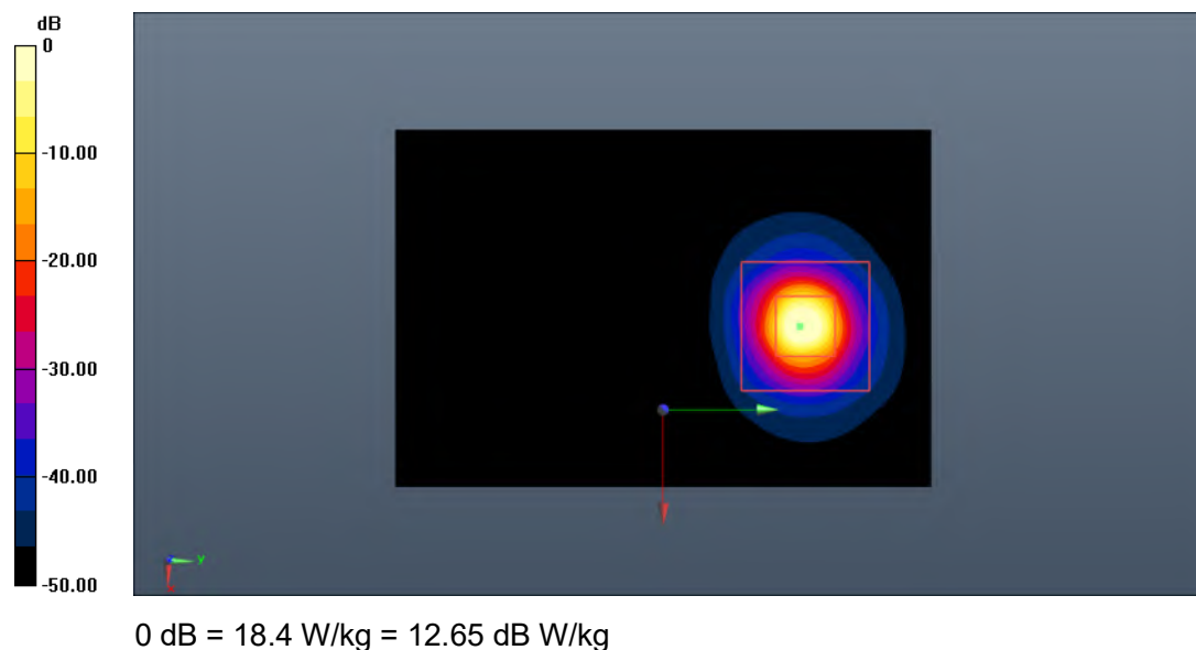
Fig.B.13. Validation 5750MHz 100mW
