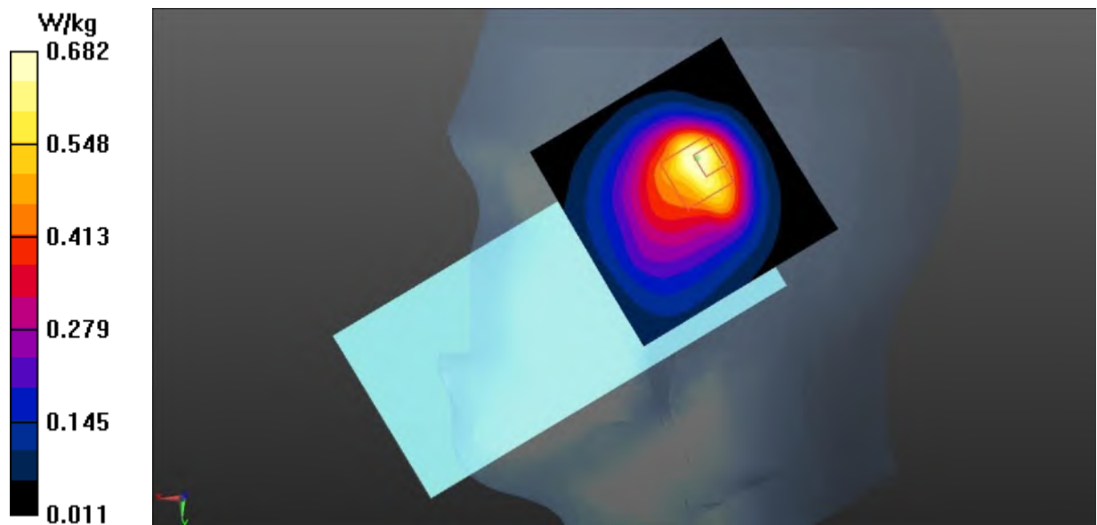
Fig.15 LTE Band 13 Head
