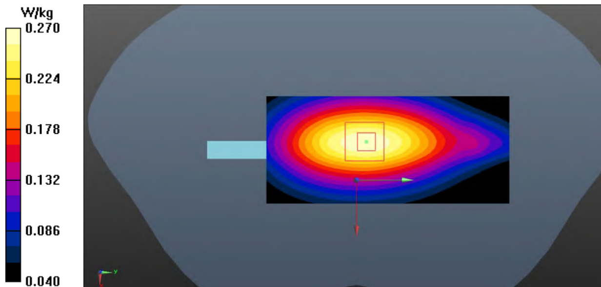
Fig.16 LTE Band 13 Body
