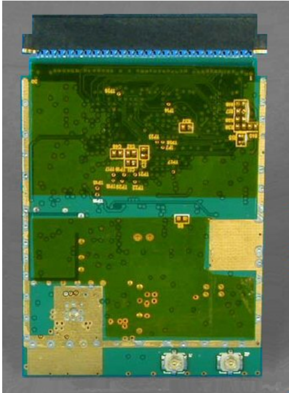
Back view of radio PCB.
