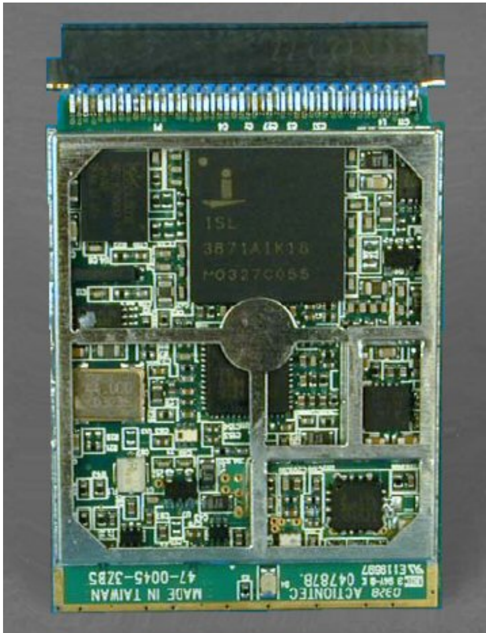
Front view of radio PCB.
