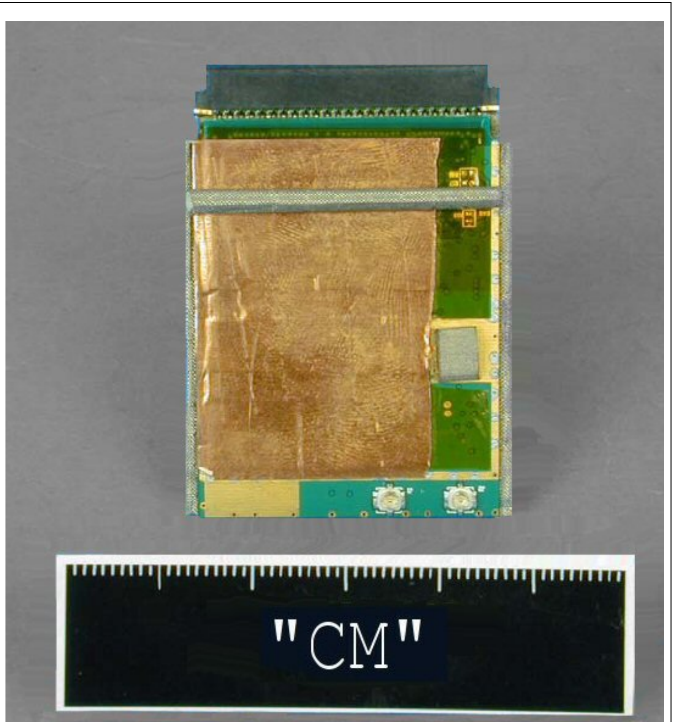
Back view of radio with internal shield.
