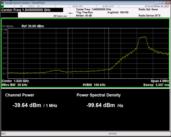
Band2 16QAM BW=5MHz Channel=18625 RB Size=1 Position=#Max Extended
