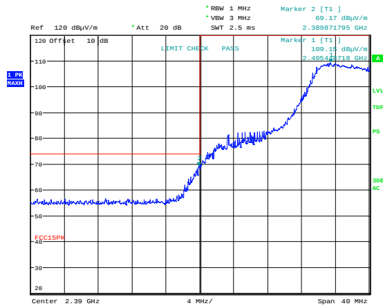
Lower Band Edge, 2412 MHz, 802.11g 54M, Peak
