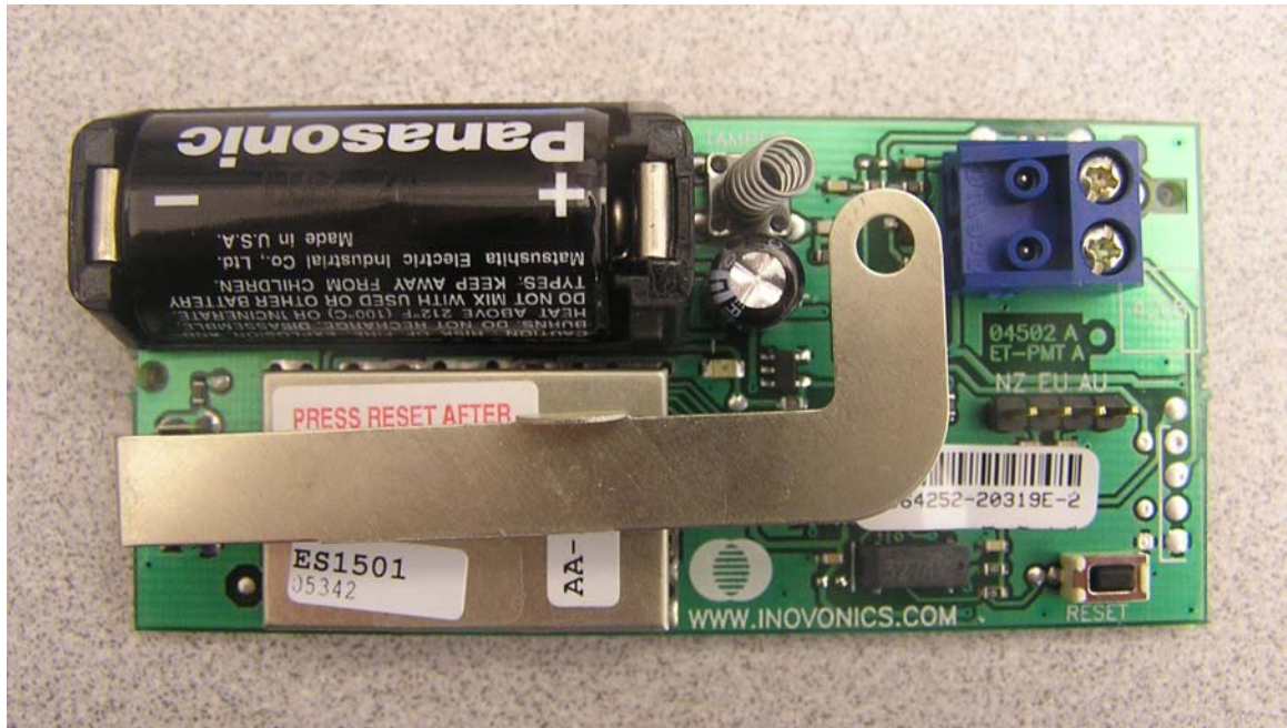
PCB front side, showing RF shielding and antenna
