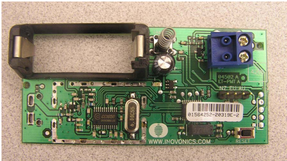
PCB front side, without shield can and antenna
