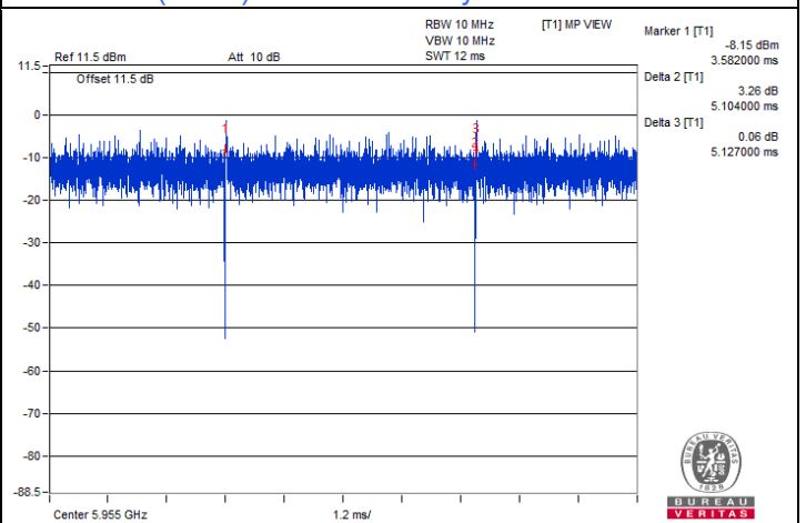
802.11ax (HE20) RU26 Under control by Low-Power Indoor AP
