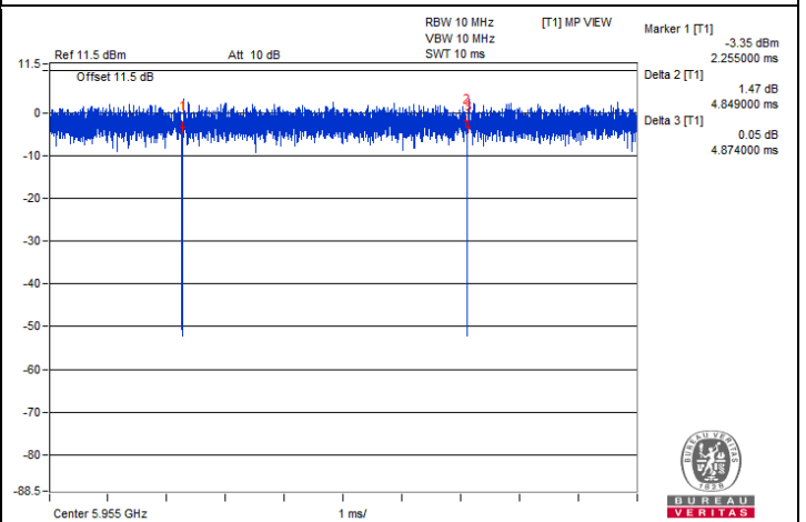
802.11ax (HE20) RU106 Under control by Low-Power Indoor AP
