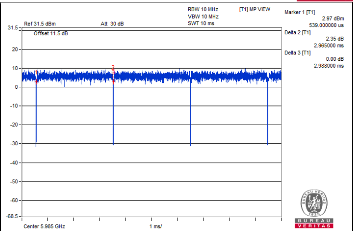
802.11ax (HE80) Under control by Low-Power Indoor AP
