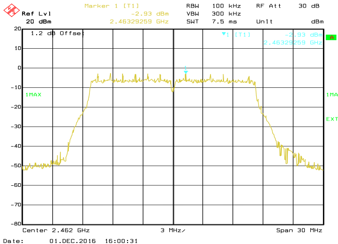
Conducted Emissions. 802.11g, Frequency 2462 MHz Reference Level
