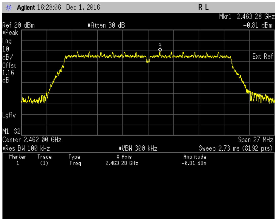
Maximum Power Spectral Density. 802.11n (HT20) Frequency 2462 MHz
