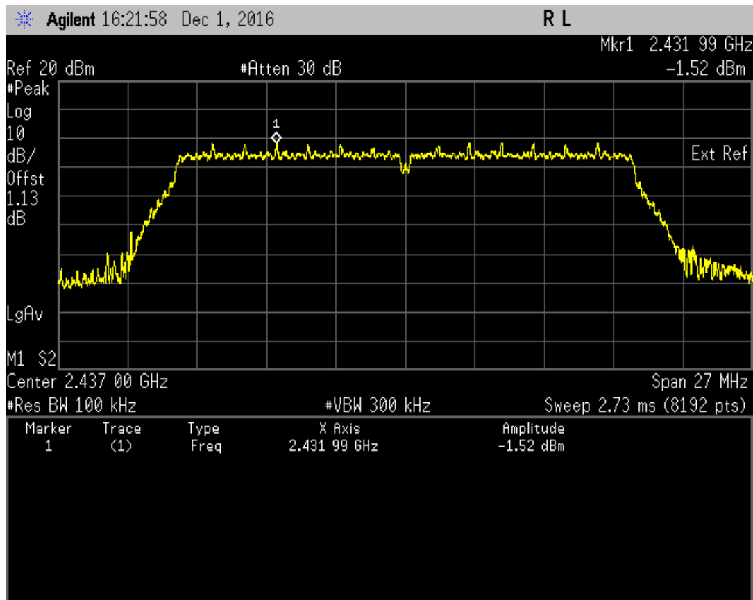
Maximum Power Spectral Density. 802.11n (HT20) Frequency 2437 MHz
