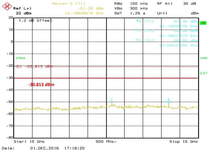
Conducted Emissions. 802.11n (HT20), Frequency 2462 MHz Emission Level, 10 GHz -> 15 GHz
