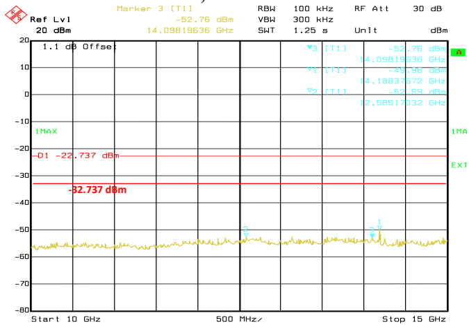
Conducted Emissions. 802.11g, Frequency 2437 MHz Emission Level, 10 GHz -> 15 GHz
