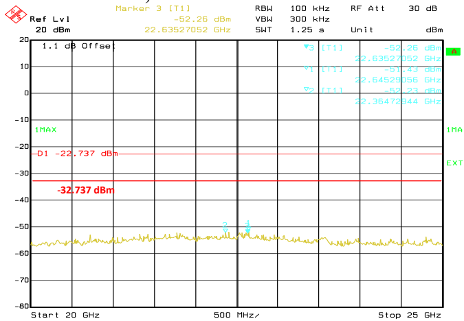
Conducted Emissions. 802.11g, Frequency 2437 MHz Emission Level, 20 GHz -> 25 GHz
