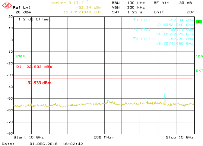
Conducted Emissions. 802.11g, Frequency 2462 MHz Emission Level, 10 GHz -> 15 GHz
