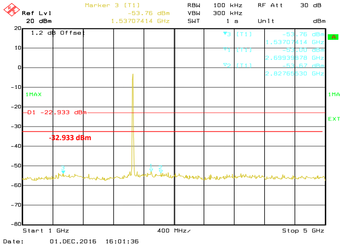
Conducted Emissions. 802.11g, Frequency 2462 MHz Emission Level, 1 GHz -> 5 GHz
