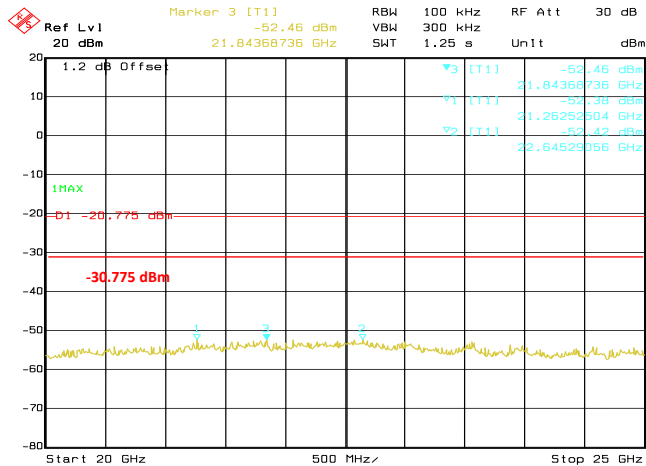
Conducted Emissions. 802.11n (HT20), Frequency 2412 MHz Emission Level, 20 GHz - > 25 GHz
