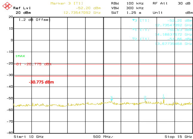
Conducted Emissions. 802.11n (HT20), Frequency 2412 Emission Level, 10 GHz -> 15 GHz
