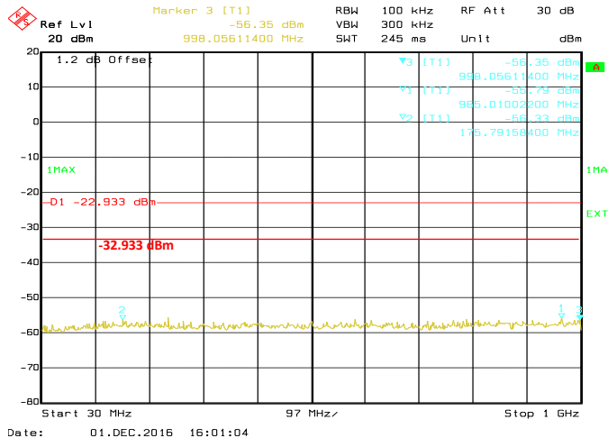
Conducted Emissions. 802.11g, Frequency 2462 MHz Emission Level, 30 MHz -> 1 GHz
