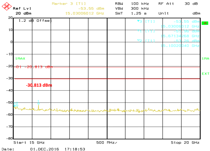
Conducted Emissions. 802.11n (HT20), Frequency 2462 MHz Emission Level, 15 GHz -> 20 GHz
