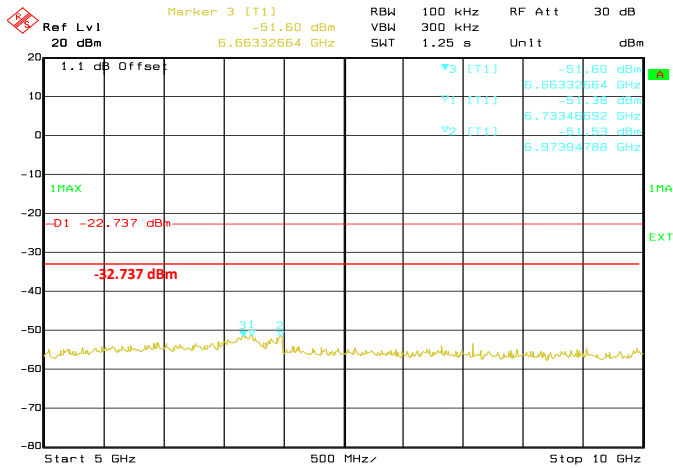
Conducted Emissions. 802.11g, Frequency 2437 MHz Emission Level, 5 GHz -> 10 GHz
