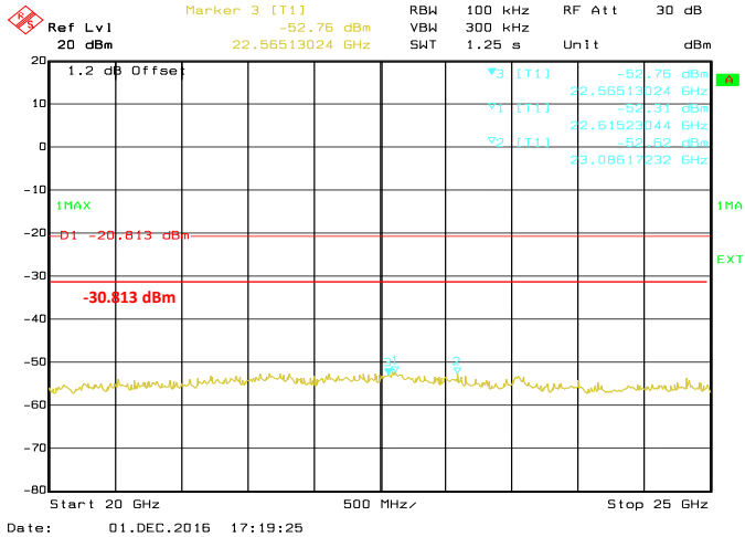
Conducted Emissions. 802.11n (HT20), Frequency 2462 MHz Emission Level, 20 GHz -> 25 GHz
