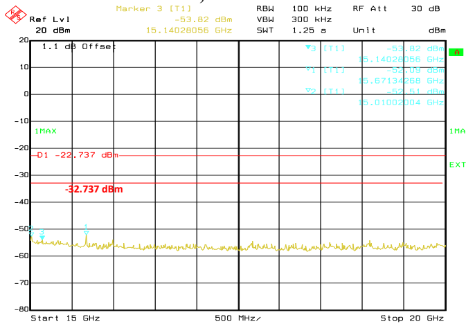
Conducted Emissions. 802.11g, Frequency 2437 MHz Emission Level, 15 GHz -> 20 GHz
