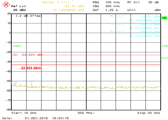
Conducted Emissions. 802.11g, Frequency 2462 MHz Emission Level, 15 GHz -> 20 GHz
