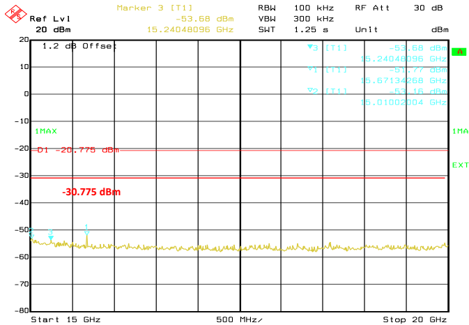
Conducted Emissions. 802.11n (HT20), Frequency 2412 MHz Emission Level, 15 GHz - > 20 GHz
