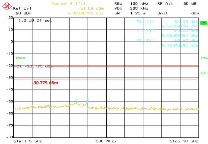
Conducted Emissions. 802.11n (HT20), Frequency 2412 MHz Emission Level, 5 GHz -> 10 GHz
