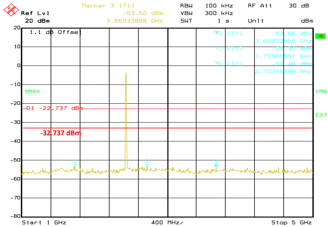
Conducted Emissions. 802.11g, Frequency 2437 MHz Emission Level, 1 GHz -> 5 GHz
