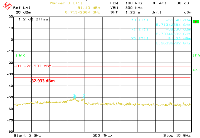
Conducted Emissions. 802.11g, Frequency 2462 MHz Emission Level, 5 GHz -> 10 GHz
