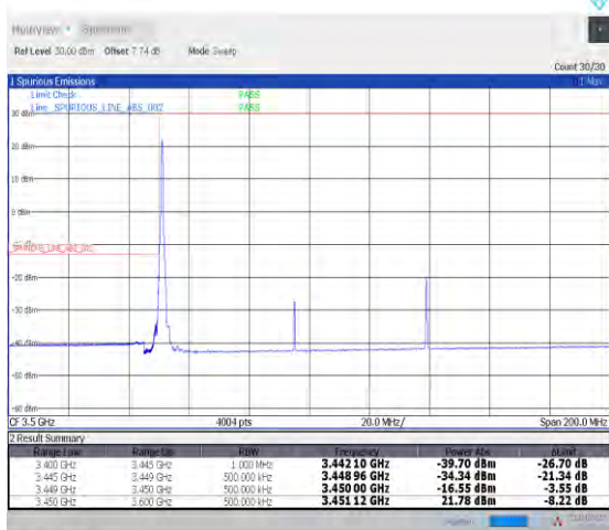
1-N78-3450-3550--30-90-L-4-CP-QPSK-Edge_1RB_L_eft-1@0-Ant1-PASS-see graph
