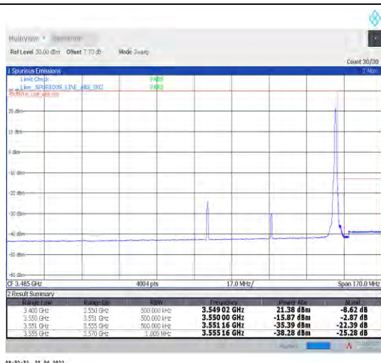
1-N78-3450-3550--30-60-H-2-DFT-PI2BPSK-Edge_1R_B_Right-1@161-Ant1-PASS-see graph
