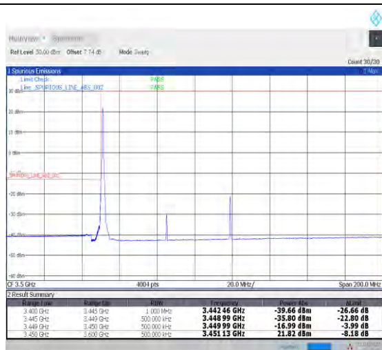
1-N78-3450-3550--30-70-L-1-DFT-PI2BPSK-Edge_1R_B_Left-1@0-Ant1-PASS-see graph
