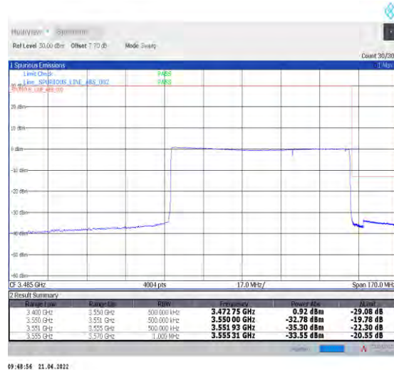
1-N78-3450-3550--30-80-H-6-CP-QPSK-Outer_Full-217@0-Ant1-PASS-see graph
