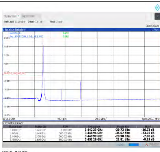
1-N78-3450-3550--30-50-L-1-DFT-PI2BPSK-Edge_1R_B_Left-1@0-Ant1-PASS-see graph
