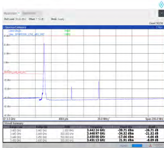
1-N78-3450-3550--30-70-L-4-CP-QPSK-Edge_1RB_L_eft-1@0-Ant1-PASS-see graph
