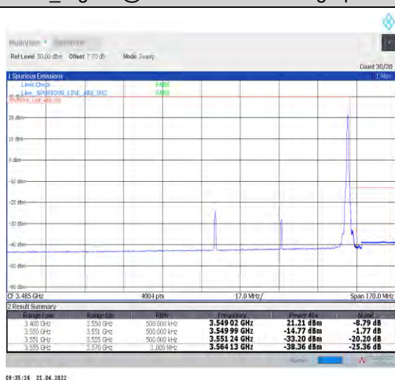
1-N78-3450-3550--30-60-H-5-CP-QPSK-Edge_1RB_Right-1@161-Ant1-PASS-see graph
