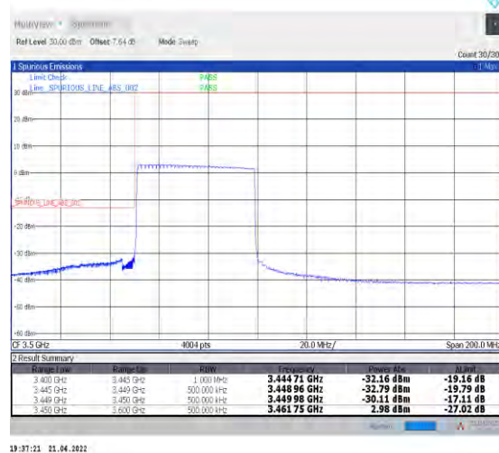
1-N78-3450-3550--30-50-L-6-CP-QPSK-Outer_Ful_I-133@0-Ant1-PASS-see graph
