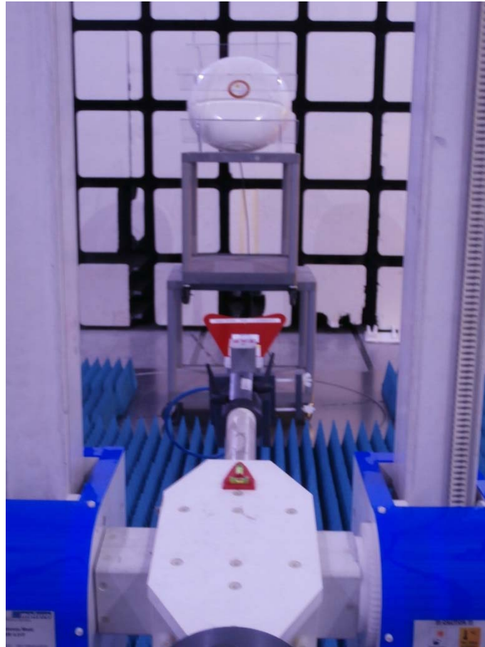
FCC Part 25 Radiated Emissions/EIRP - 1 GHz to 18 GHz – Reference View – 60 degrees
