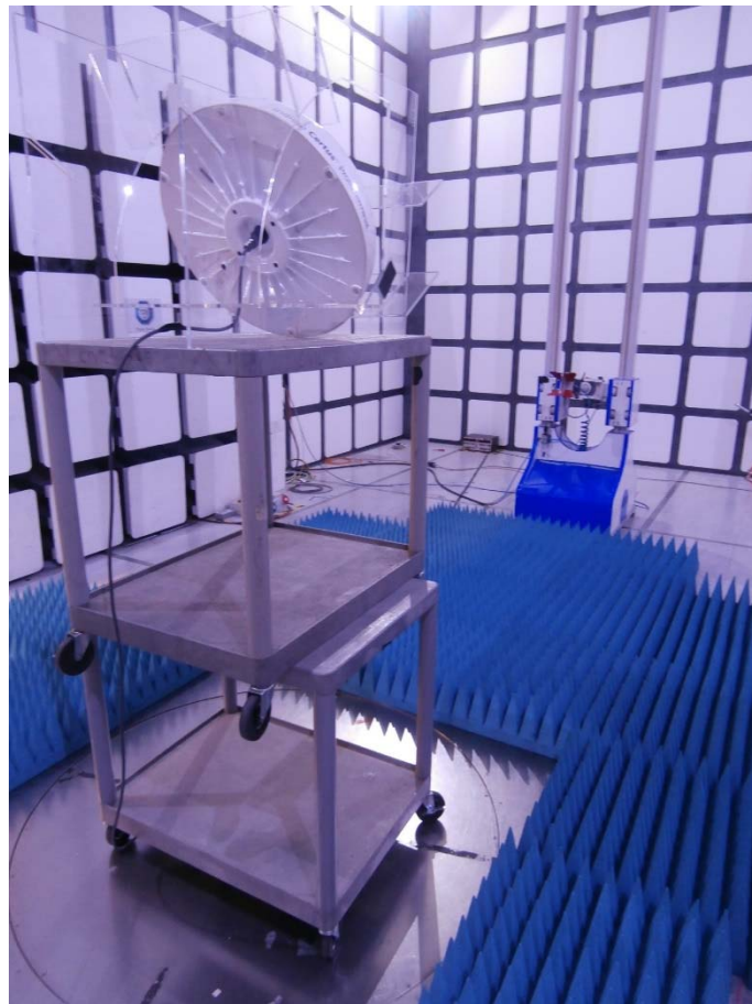
FCC Part 25 Radiated Emissions/EIRP - 1 GHz to 18 GHz – 60 degrees
