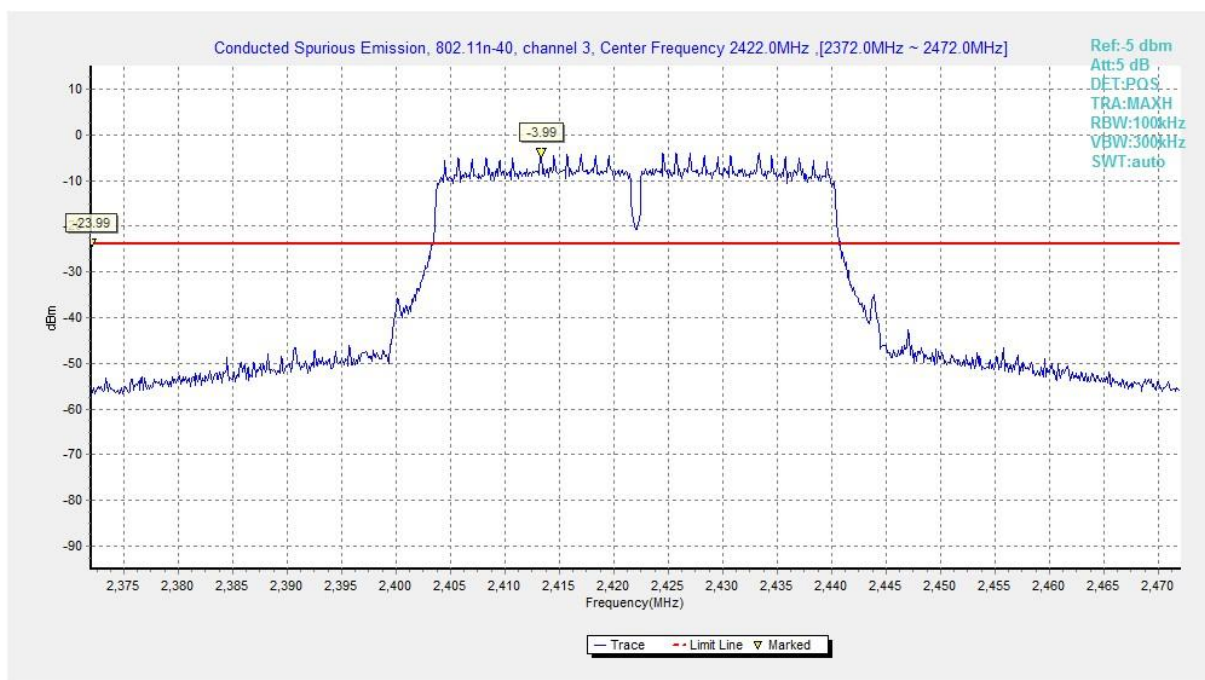
Fig.A.6.1.121 Transmitter Spurious Emission - Conducted (802.11n-HT40, Chain1, Ch3, Center Frequency)
