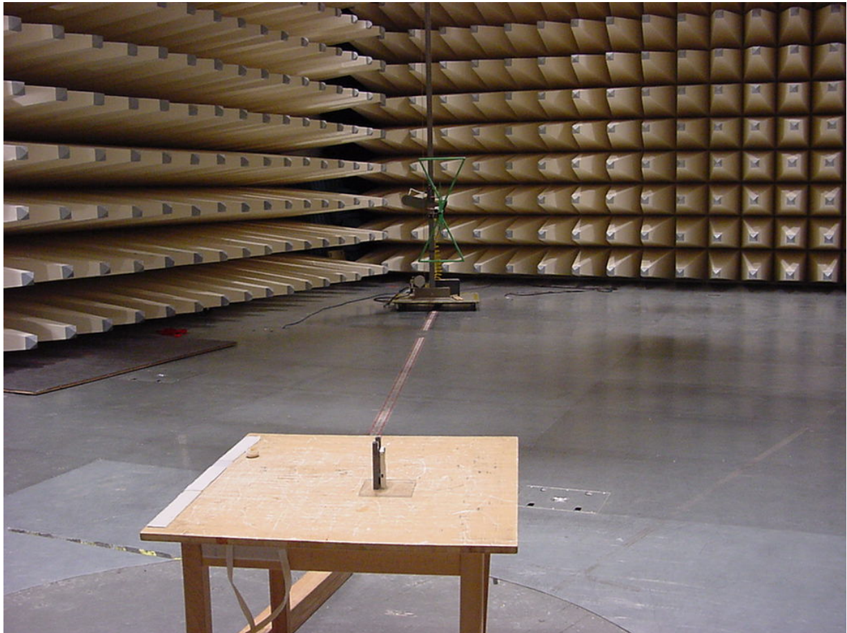
Photo 1: Radiated Emissions
