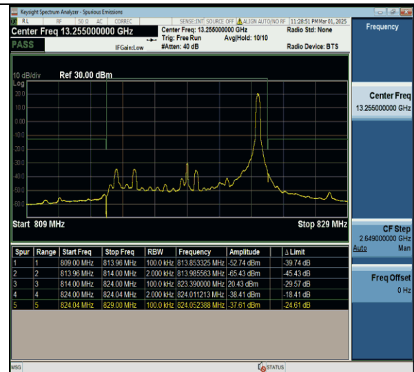
Band26(814-824)-10MHz-QPSK-26740-1RB#49-PASS
