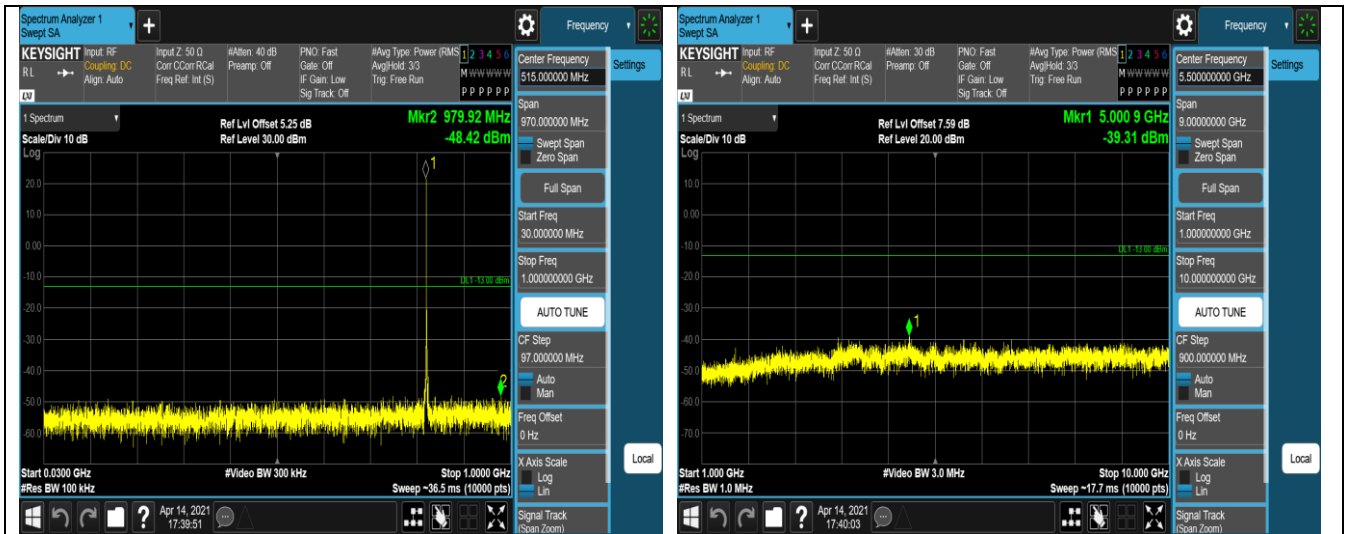
Band5-1.4MHz-16QAM-20525-1RB#0-Range1:30~1
