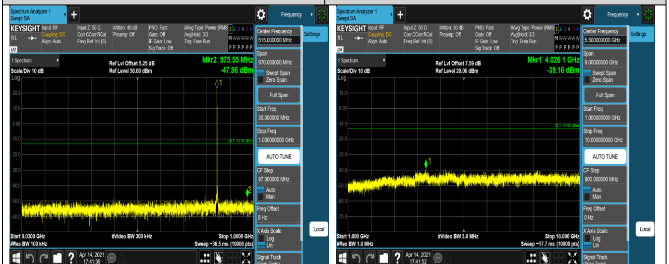
Band5-1.4MHz-16QAM-20643-1RB#0-Range1:30~1
