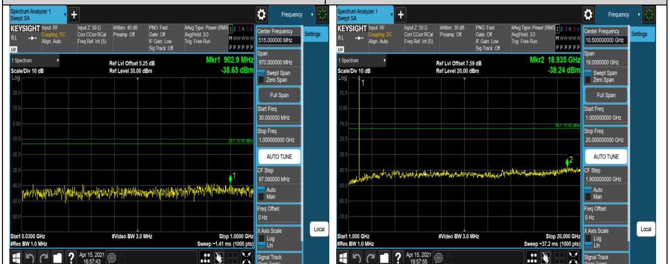
Band2-1.4MHz-16QAM-18900-1RB#0-Range1:30~1
