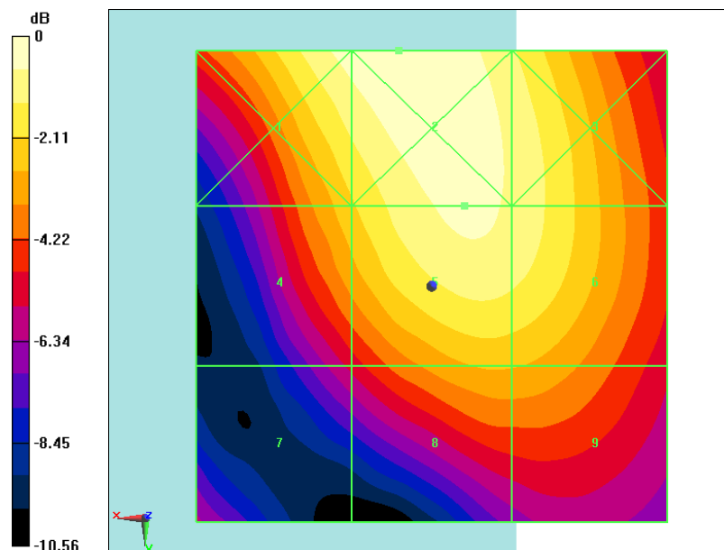
Fig B.33 HAC RF E-Field LTE Band41 QPSK CH40620
