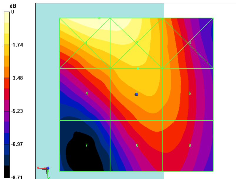
Fig B.45 HAC RF E-Field LTE Band41 64QAM CH39750
