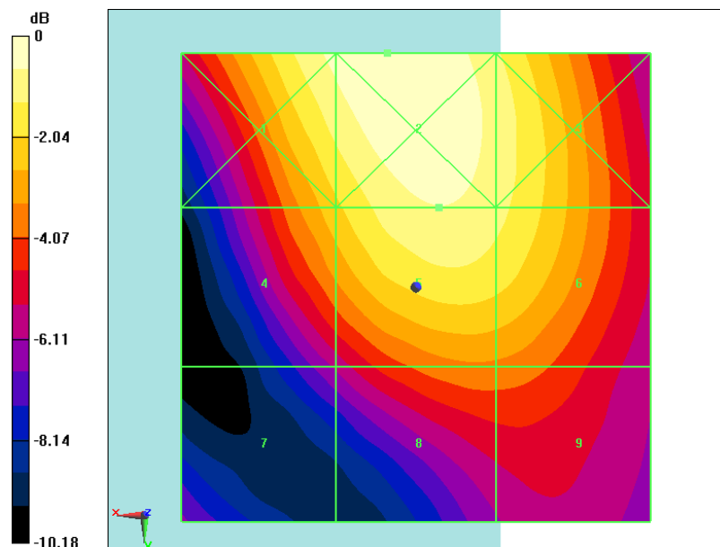
Fig B.43 HAC RF E-Field LTE Band41 64QAM CH40620
