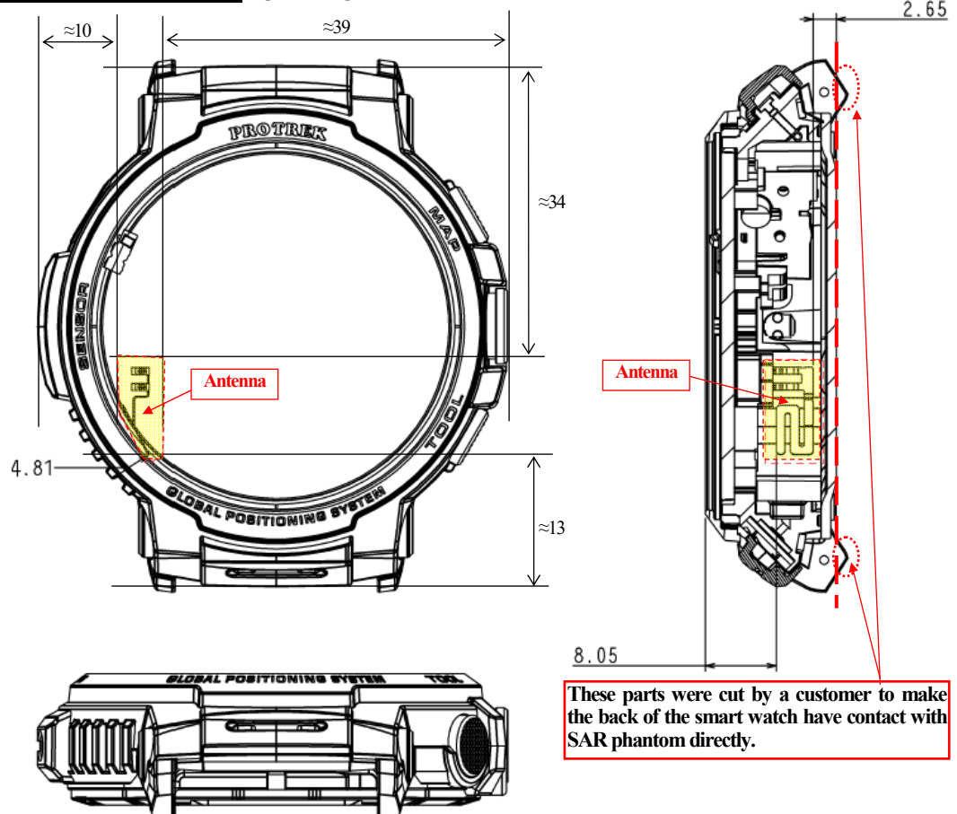
Antenna location and antenna distance [Unit: mm]
