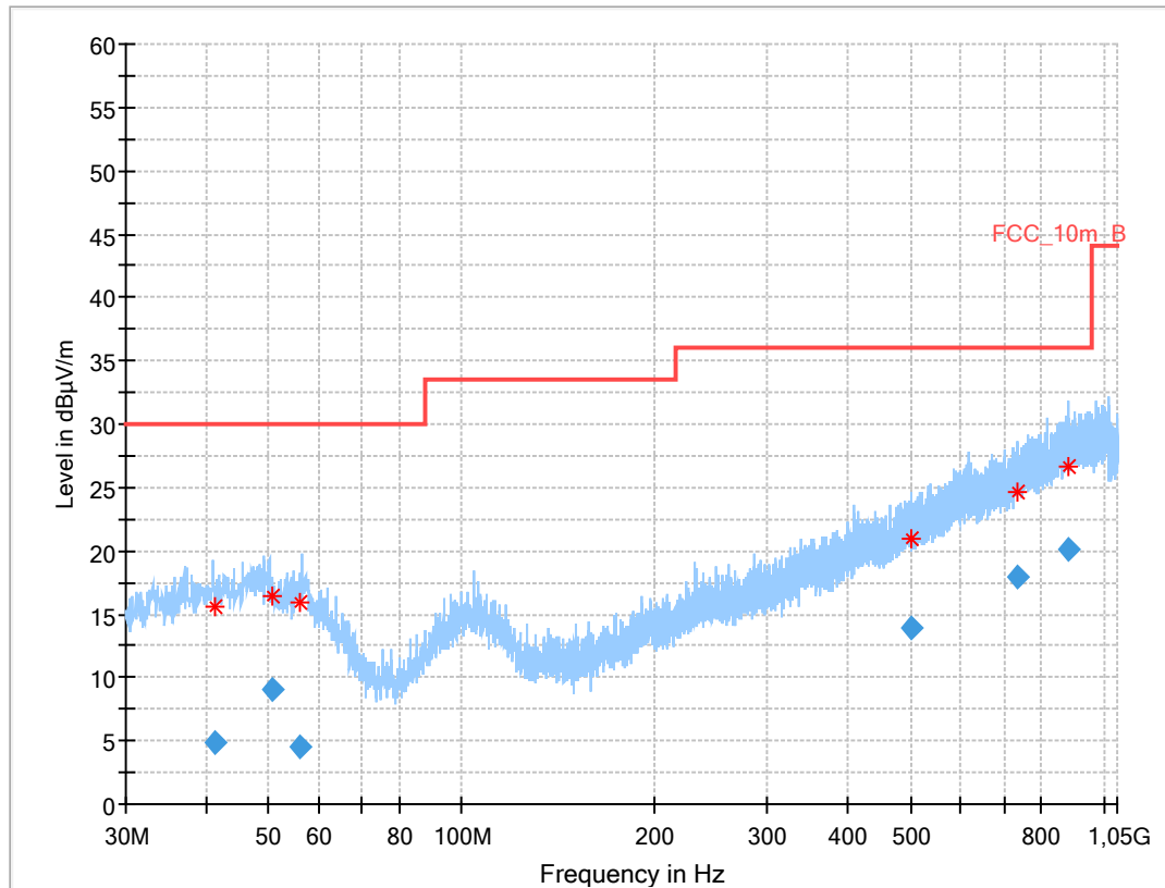
Plot 2: 30 MHz to 1 GHz, TX mode, vertical & horizontal polarization, valid for all channels of 2 Msps mode
