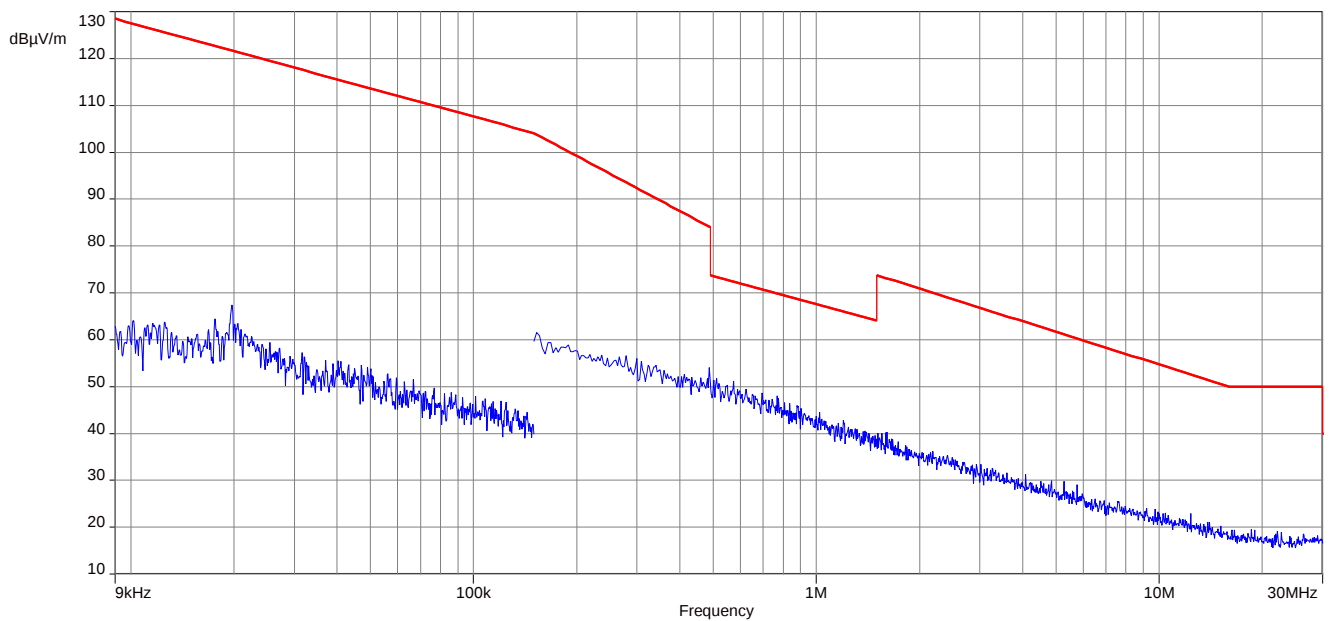
Plot 4: 9 kHz to 30 MHz, 2404 MHz, transmit mode, 2 Msps
