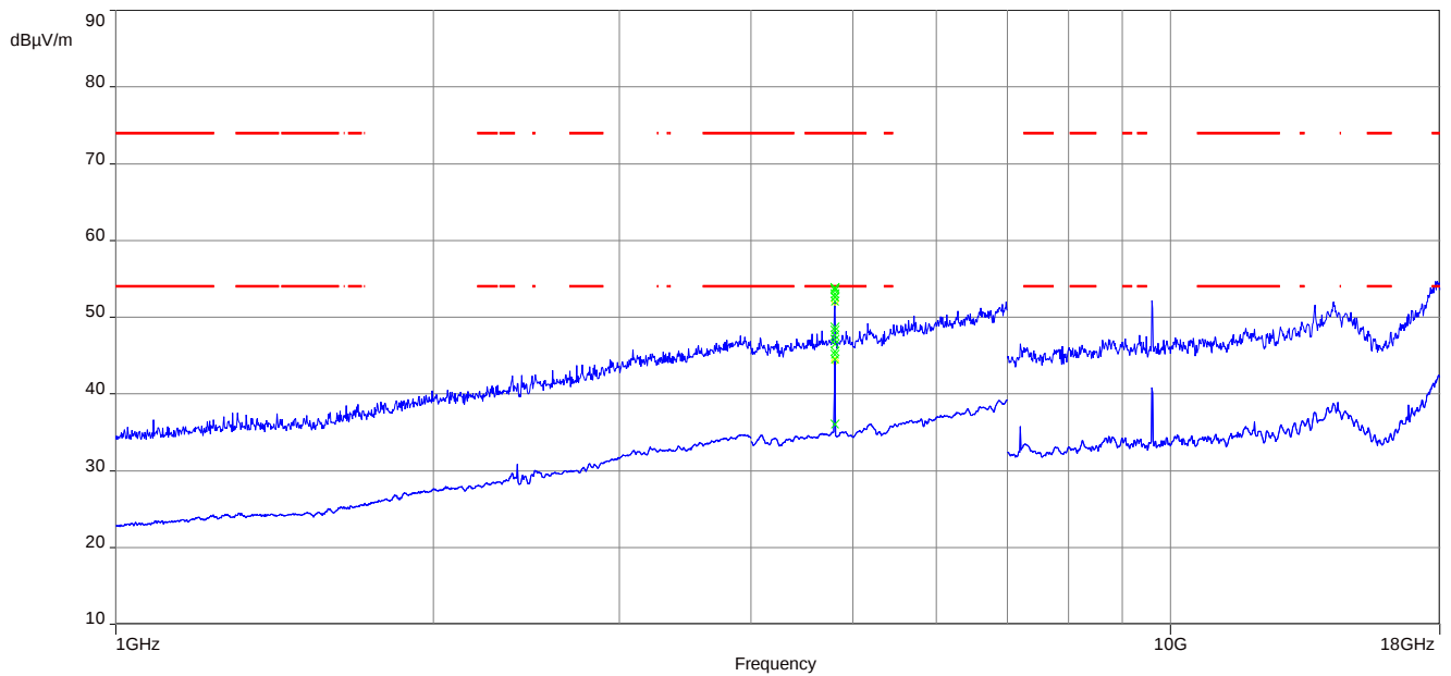
Plot 1: 1 GHz to 18 GHz, TX mode, 2402 MHz, vertical & horizontal polarization, 1 Msp
