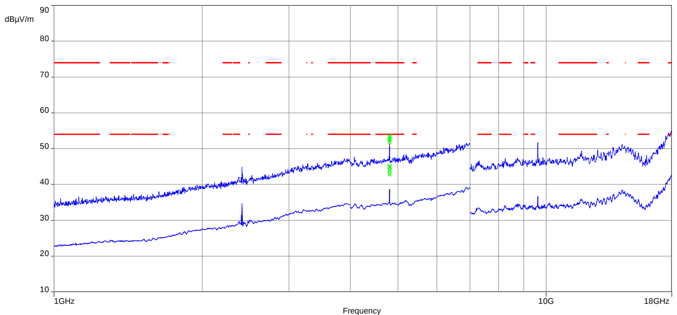
Plot 4: 1 GHz to 18 GHz, TX mode, 2404 MHz, vertical & horizontal polarization, 2 Msps
