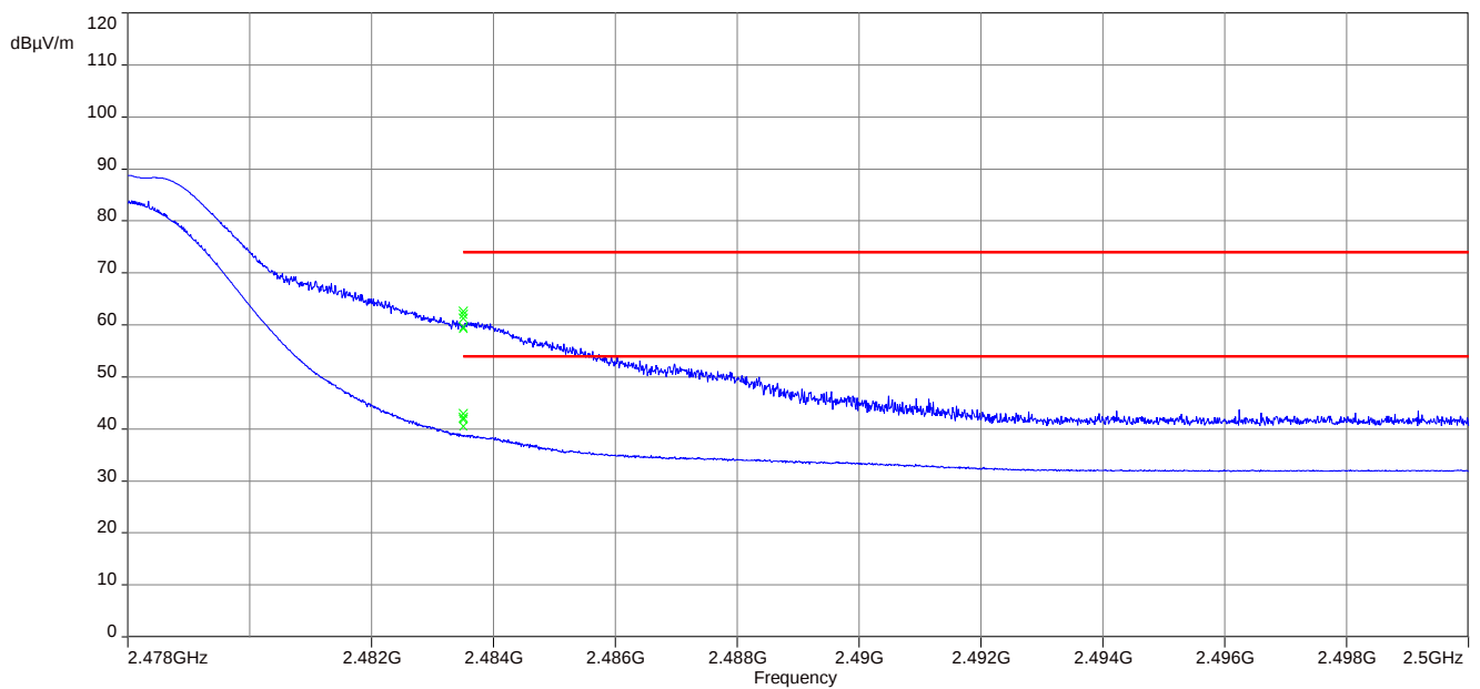
Plot 4: Upper restricted band, 2 Msp
