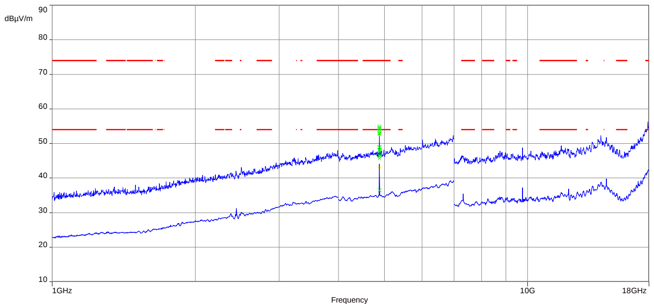
Plot 2: 1 GHz to 18 GHz, TX mode, 2440 MHz, vertical & horizontal polarization, 1 Msp
