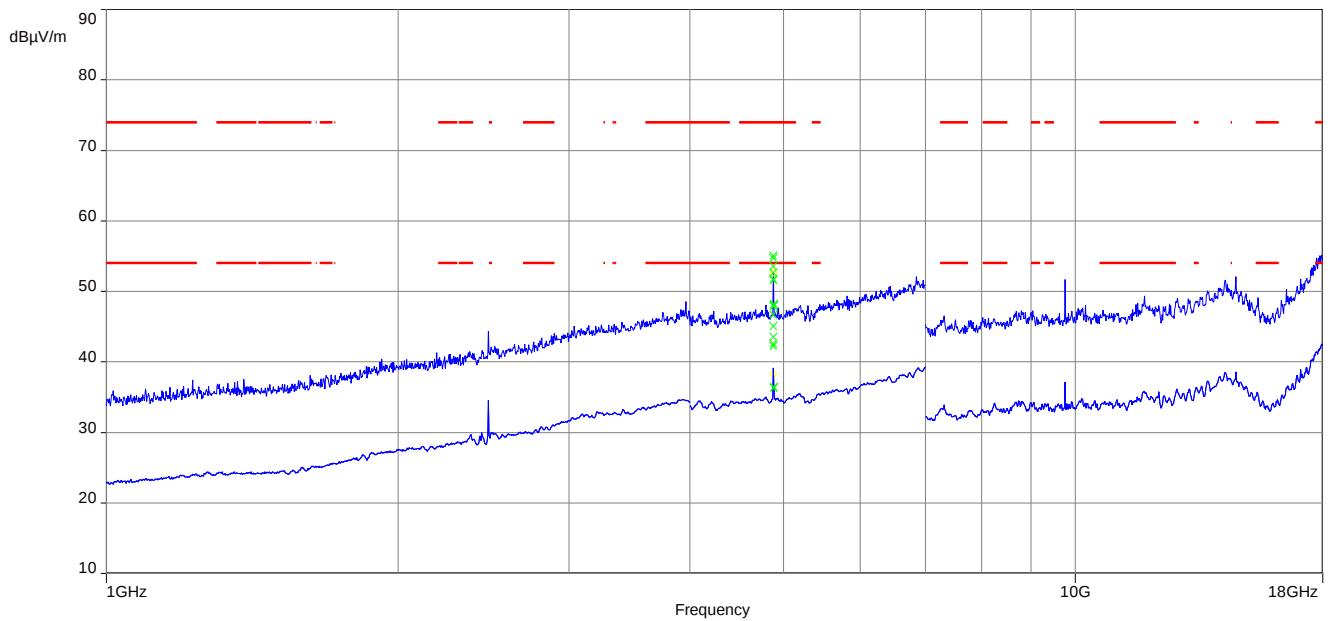
Plot 5: 1 GHz to 18 GHz, TX mode, 2440 MHz, vertical & horizontal polarization, 2 Msps
