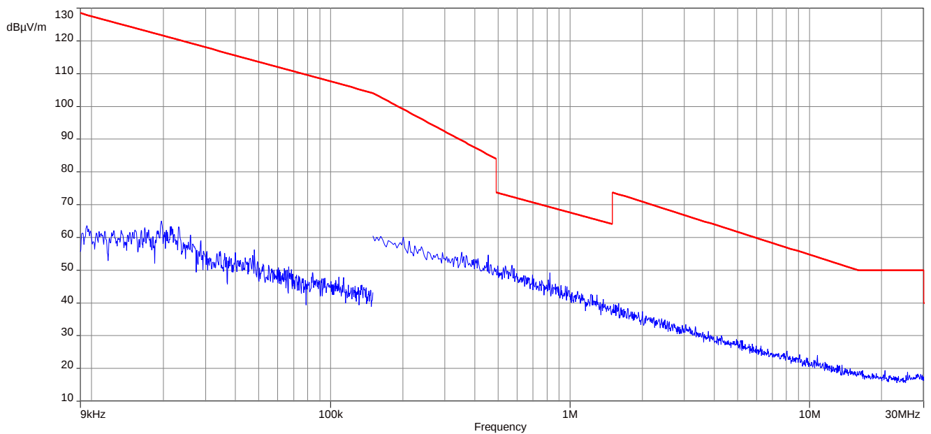
Plot 6: 9 kHz to 30 MHz, 2478 MHz, transmit mode, 2 Msps
