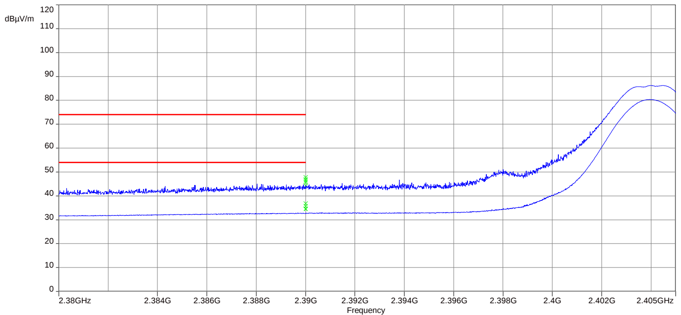
Plot 3: Lower restricted band, 2 Msp
