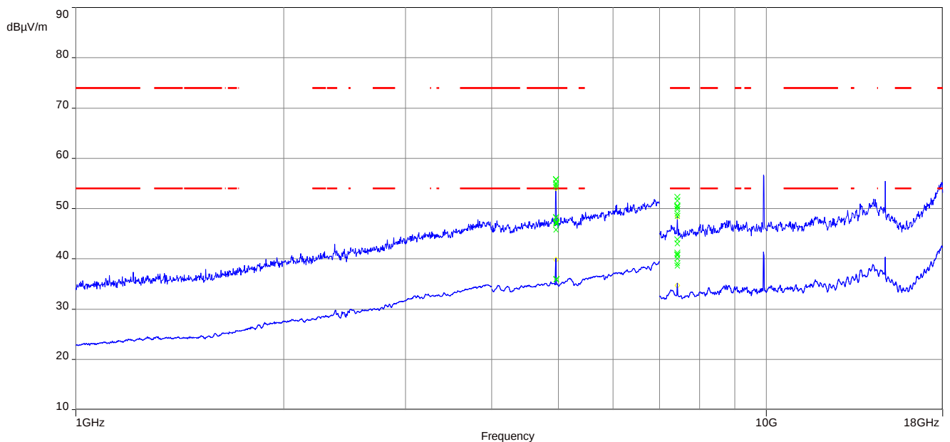
Plot 6: 1 GHz to 18 GHz, TX mode, 2478 MHz, vertical & horizontal polarization, 2 Msps
