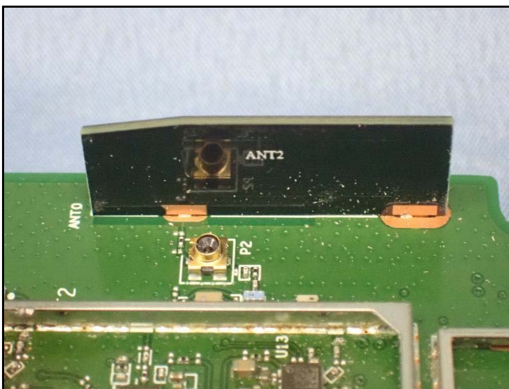
Antenna 1 (Model: RFPCA291200NNLB001)
