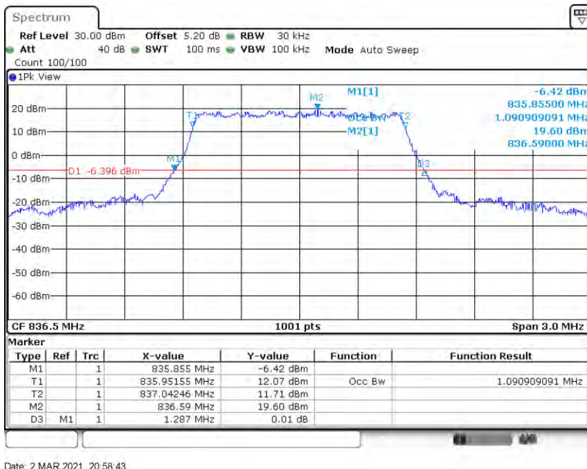
Band5-1.4MHz-QPSK-20525-6RB#0-1.091
