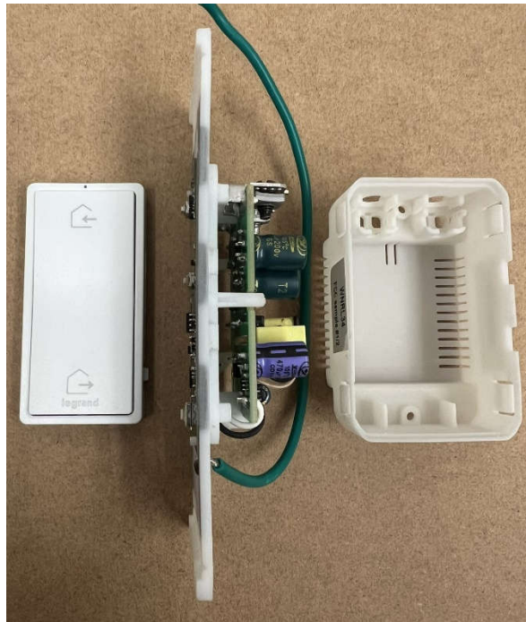
WNRL34 Front and Back Cover Removed
