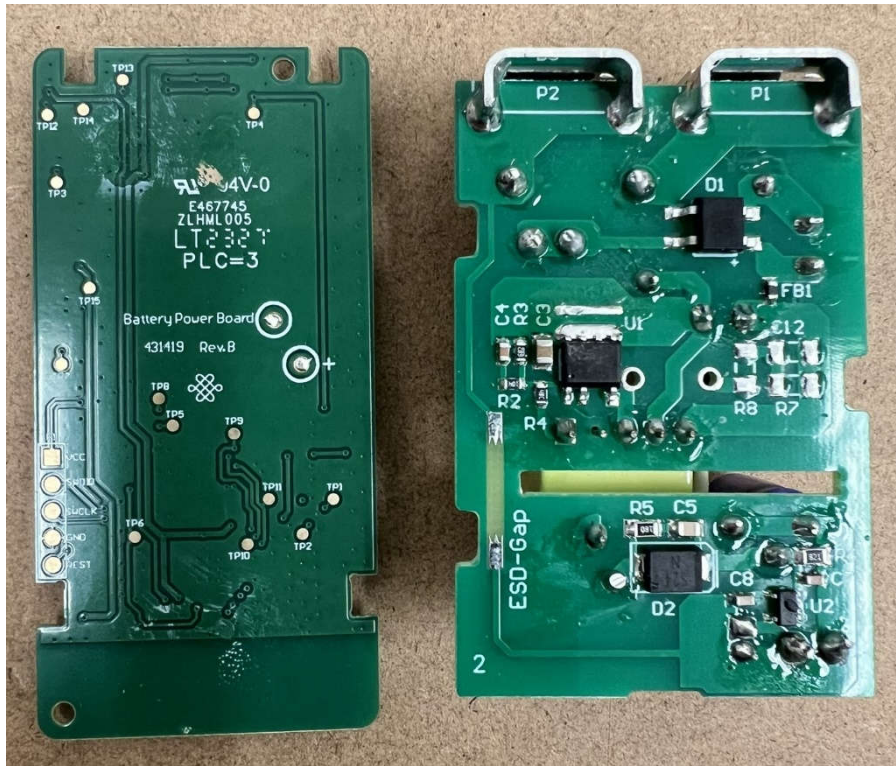
WNRL34 RF Board Back Side (Left) – AC Board Top Side (Right)
