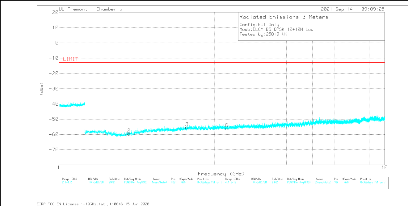
Vertical Polarity
