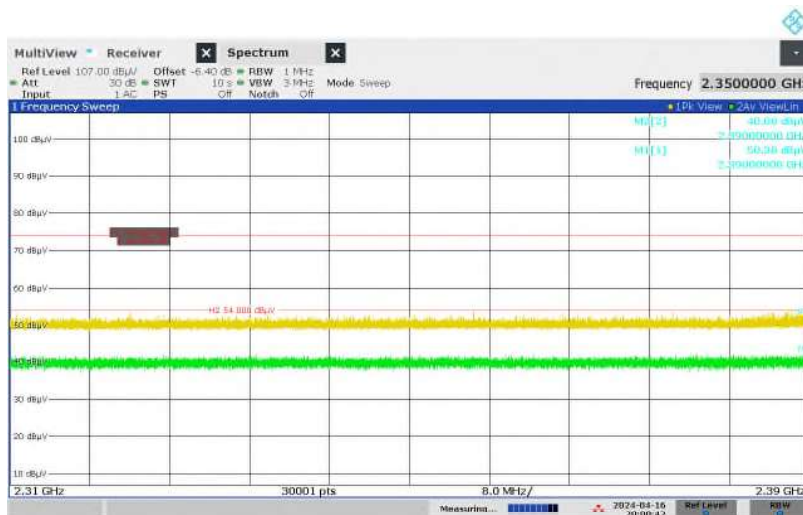
Figure 58: Restricted-band Band-edge, Spectral Diagram, Original Wireless Communication (2402MHz, ANT2) + WLAN 2.4GHz, Horizontal Antenna Orientation
