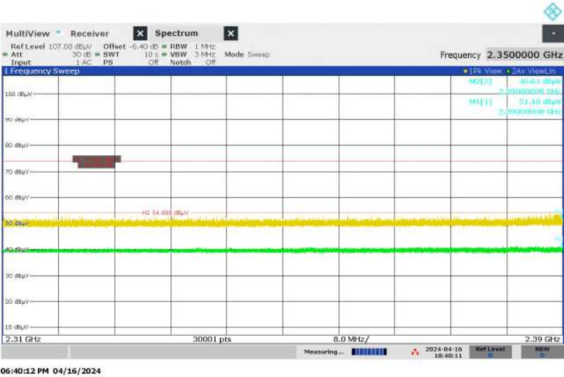
Figure 54: Restricted-band Band-edge, Spectral Diagram, Original Wireless Communication (2402MHz, ANT1) + WLAN 2.4GHz, Horizontal Antenna Orientation
