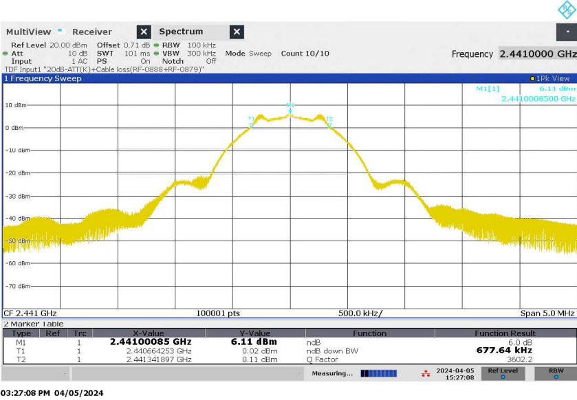
Figure 3: 6dB Bandwidth, Original Wireless Communication, Mode M (2441MHz), ANT1
