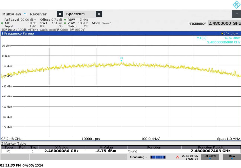
Figure 26: Power Spectral Density, Original Wireless Communication, Mode H (2480MHz), ANT1
