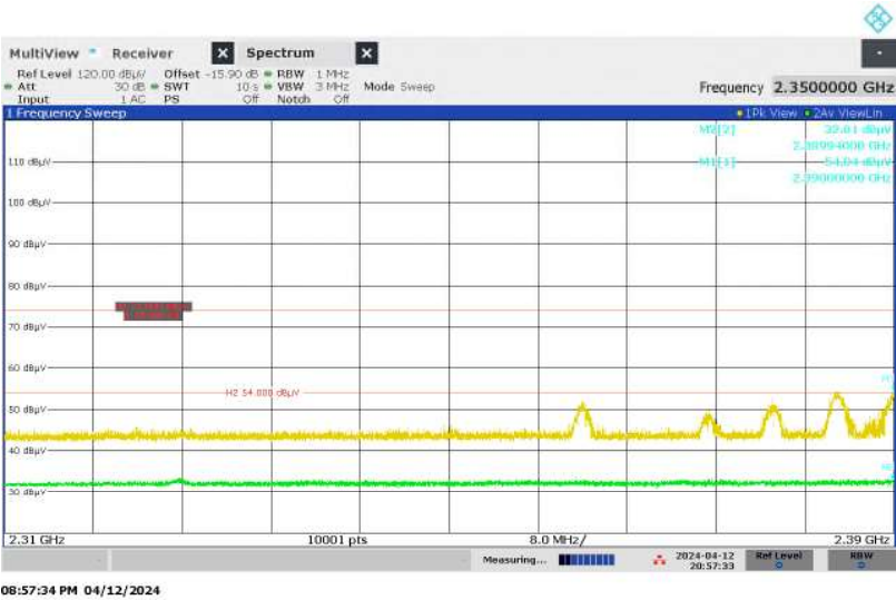
Figure 42: Restricted-band Band-edge, Spectral Diagram, Original Wireless Communication (2402MHz, ANT2) + WLAN 5GHz + Bluetooth Classic, Horizontal Antenna Orientation
