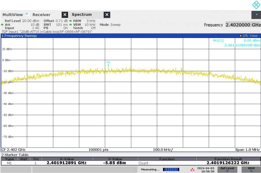
Figure 27: Power Spectral Density, Original Wireless Communication, Mode L (2402MHz), ANT2
