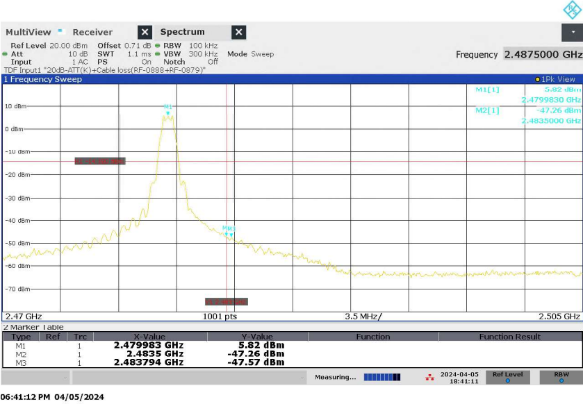
Figure 23: Authorized-band band-edge, Original Wireless Communication, Mode H (2480MHz), ANT 2
