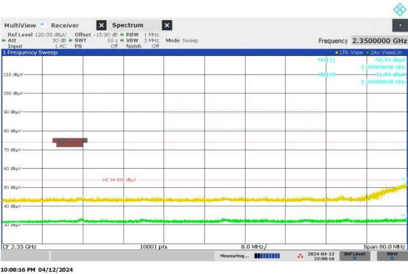
Figure 50: Restricted-band Band-edge, Spectral Diagram, Original Wireless Communication (2402MHz, ANT2) + WLAN 5GHz + Bluetooth Low Energy, Horizontal Antenna Orientation
