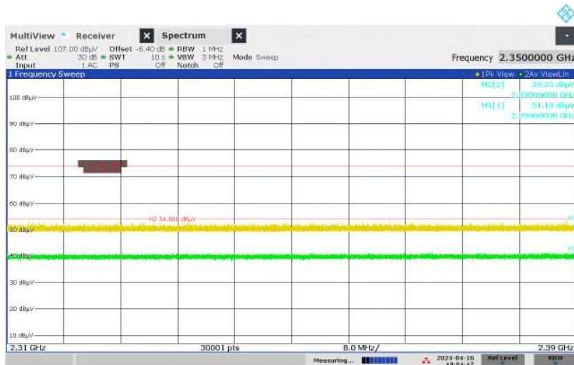
Figure 55: Restricted-band Band-edge, Spectral Diagram, Original Wireless Communication (2402MHz, ANT1) + WLAN 2.4GHz, Vertical Antenna Orientation
