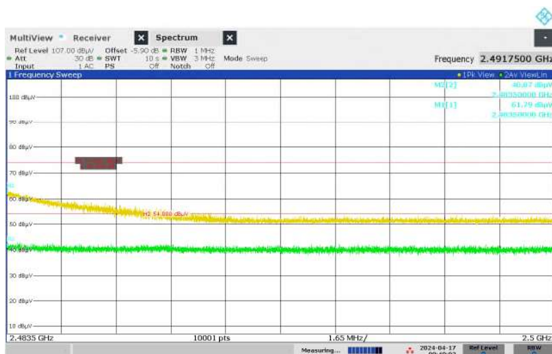
Figure 56: Restricted-band Band-edge, Spectral Diagram, Original Wireless Communication (2480MHz, ANT1) + WLAN 2.4GHz, Horizontal Antenna Orientation
