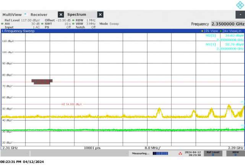
Figure 38: Restricted-band Band-edge, Spectral Diagram, Original Wireless Communication (2402MHz, ANT1) + WLAN 5GHz + Bluetooth Classic, Horizontal Antenna Orientation
