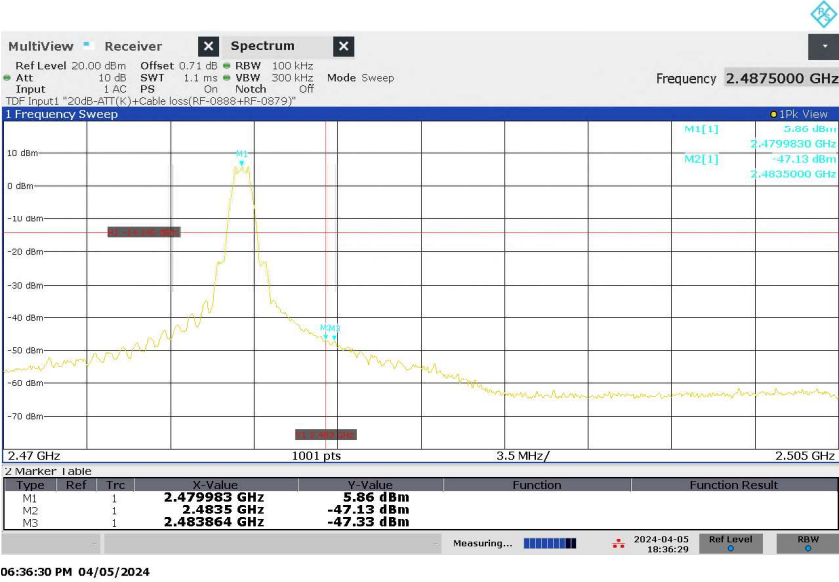
Figure 18: Authorized-band band-edge, Original Wireless Communication, Mode H (2480MHz), ANT 1
