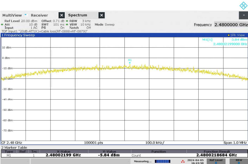
Figure 29: Power Spectral Density, Original Wireless Communication, Mode H (2480MHz), ANT2
