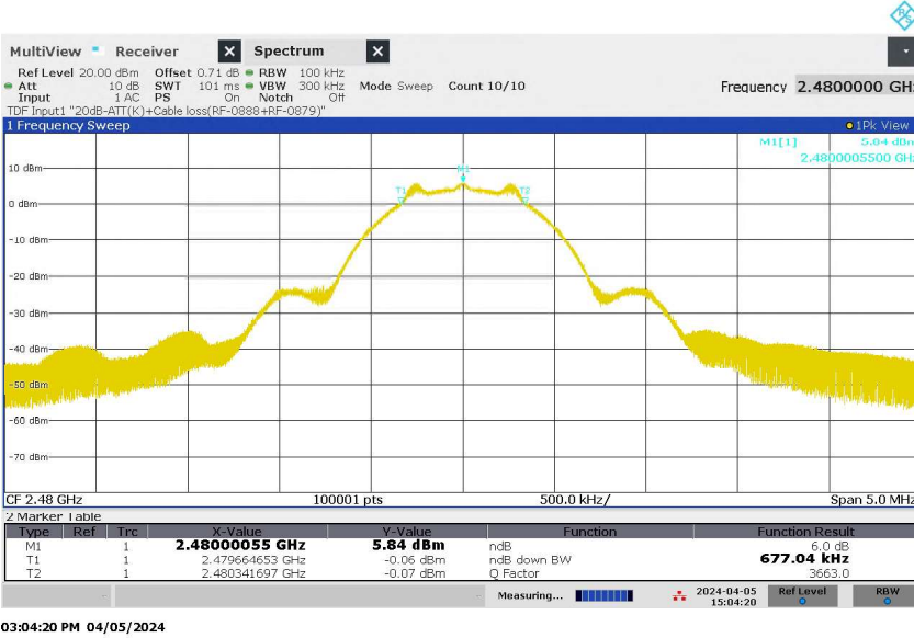
Figure 7: 6dB Bandwidth, Original Wireless Communication, Mode H (2480MHz), ANT2
