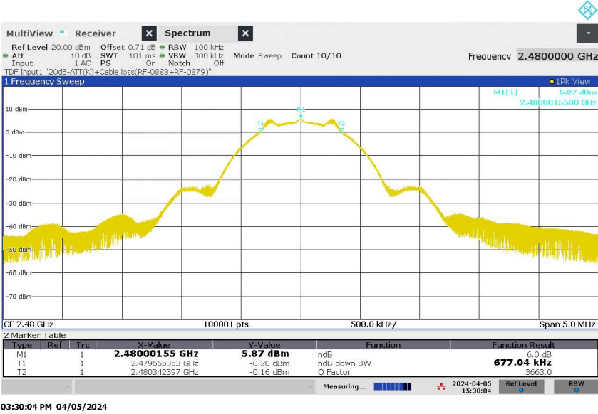
Figure 4: 6dB Bandwidth, Original Wireless Communication, Mode H (2480MHz), ANT1
