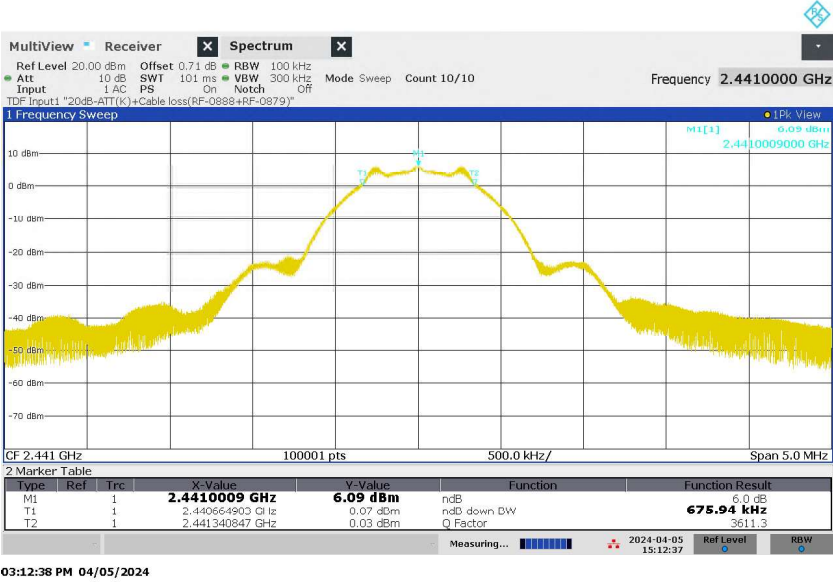
Figure 6: 6dB Bandwidth, Original Wireless Communication, Mode M (2441MHz), ANT2
