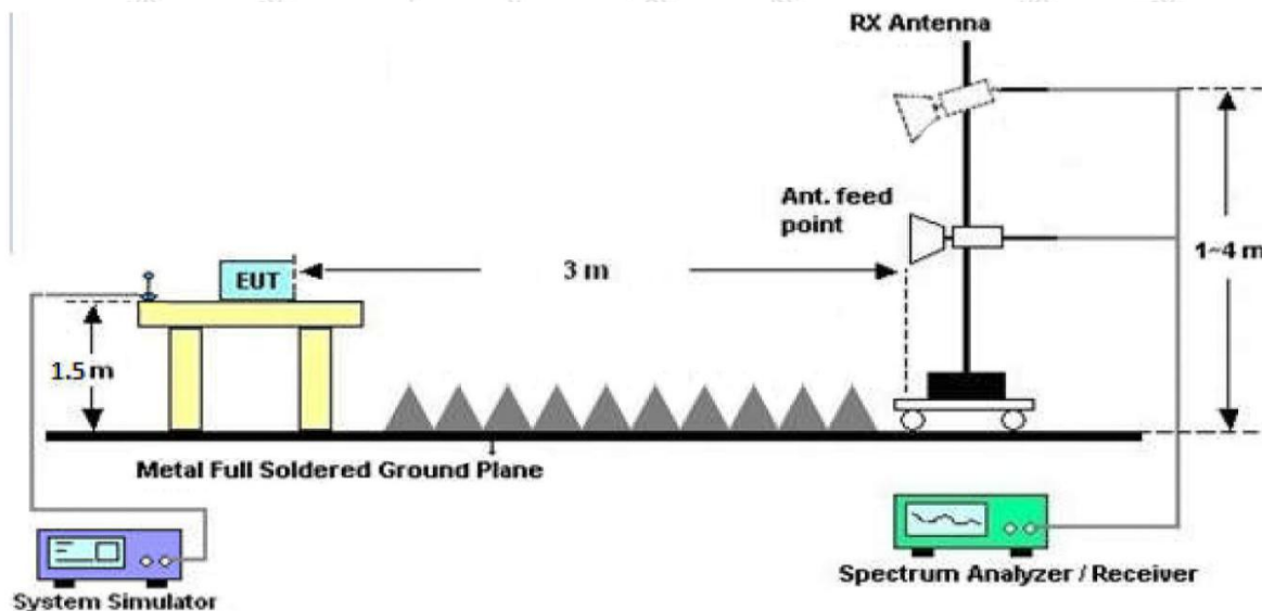
Figure 3. Above 1 GHz
