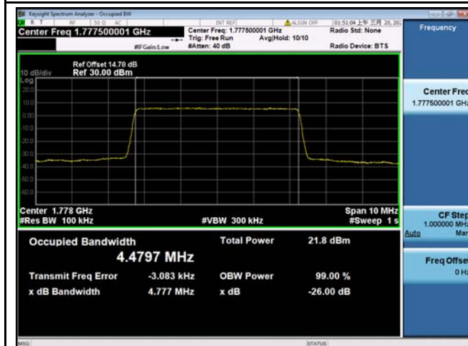
LTE band 66 - High CH QPSK-5
