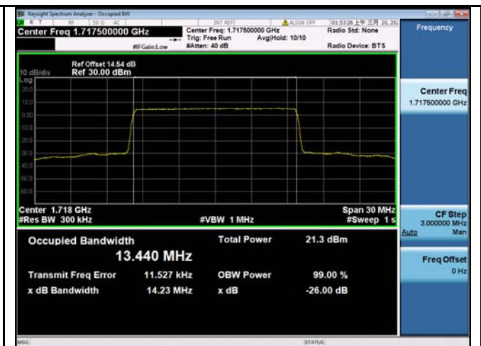
LTE band 66 - Low CH 16QAM-15
