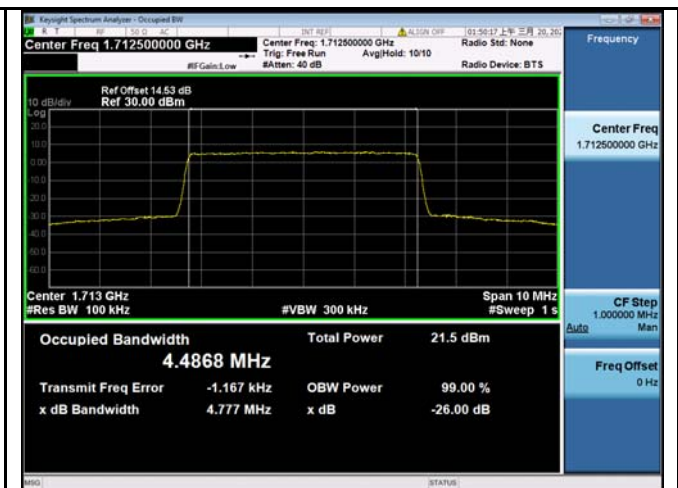
LTE band 66 - Low CH 16QAM-5
