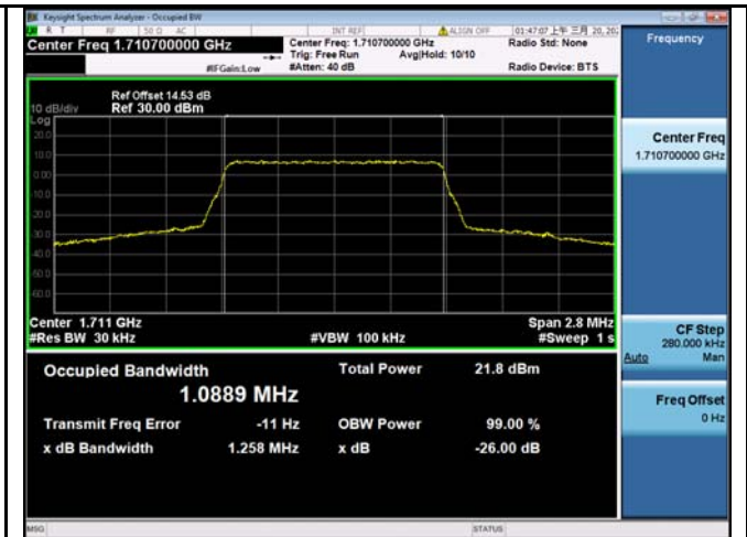
LTE band 66 - Low CH 16QAM-1.4
