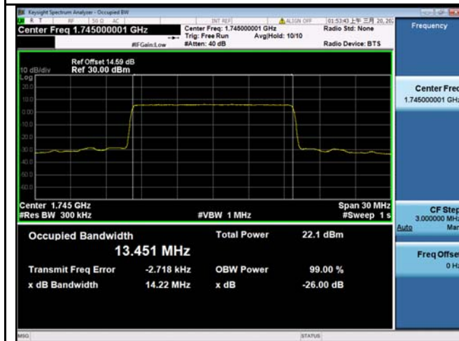
LTE band 66 - Middle CH QPSK-15
