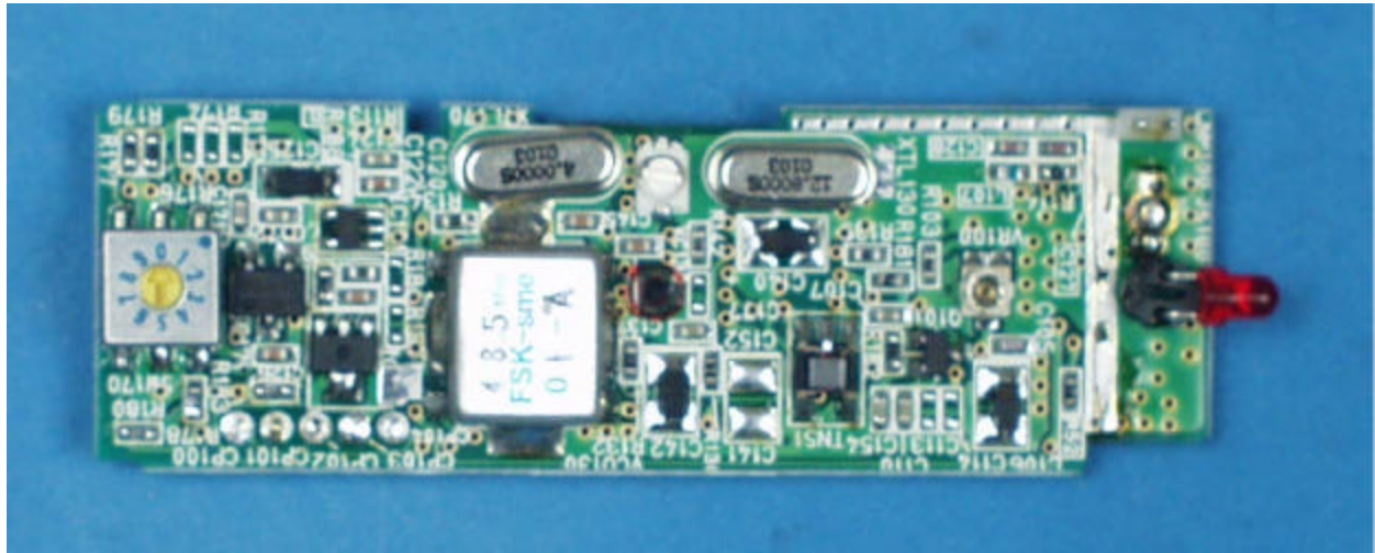
RF Board, Side 2 w/o Shield
