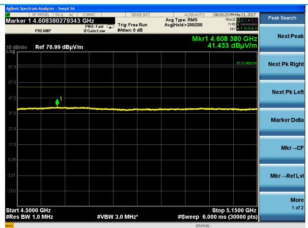
Low Channel – 802.11a HT-20 – Average
