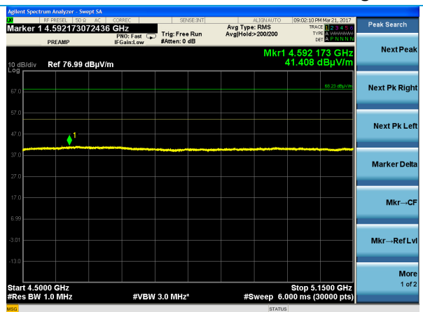
Low Channel – 802.1n HT-40 - Average
