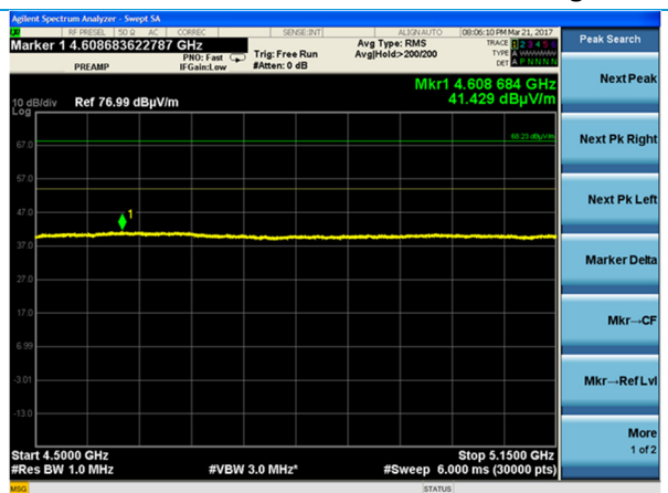
Low Channel – 802.11ac HT-20 – Average
