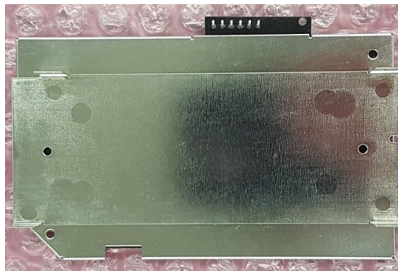
Charging coil element with connector, ferrite plate and metal shield, view from top and bottom side.
