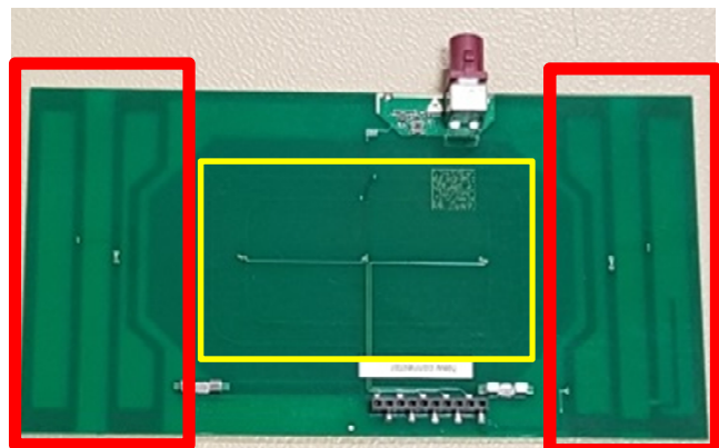
Antenna-PCB (NFC-Antenna and GSM-Coupling-Antenna), top and bottom view. The violet Fakra-Connector connects the GSM Roof-Antenna and the coupling Antenna (Red marked). The NFC-Antenna is yellow marked in the inner Layer of the PCB.
